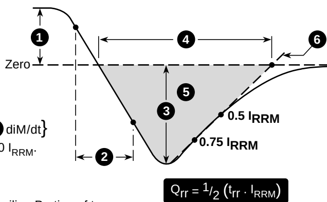
Figure 33, Diode Reverse Recovery Wave Forms and Definitions
