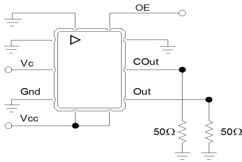
Figure 2. Production test setup (single ended into 50 Ohm)
