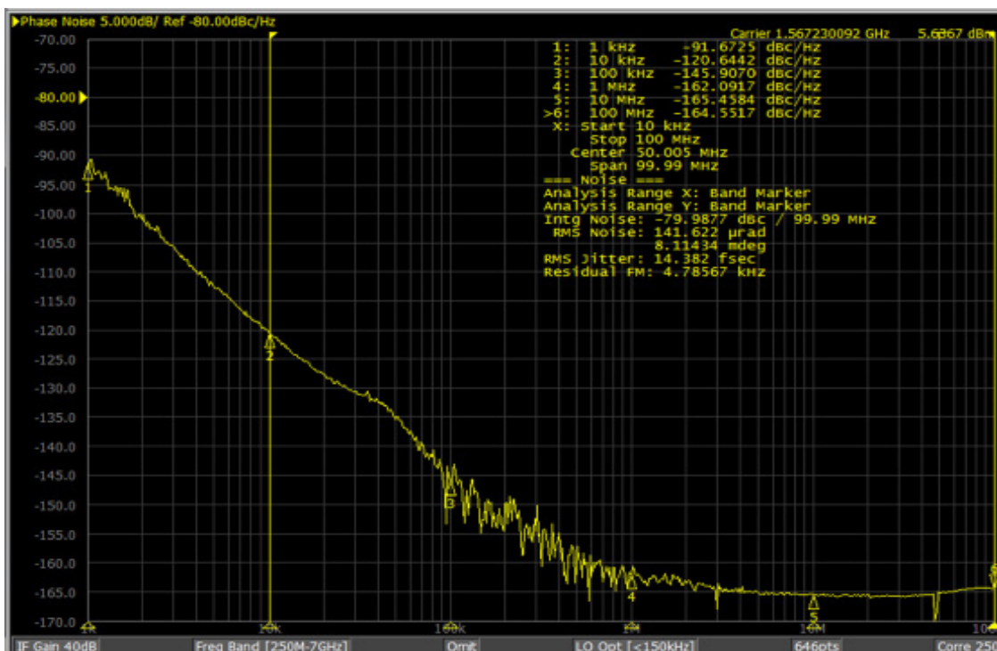
Figure 7. Typical Phase Noise Performance @ 1.56897 GHz
