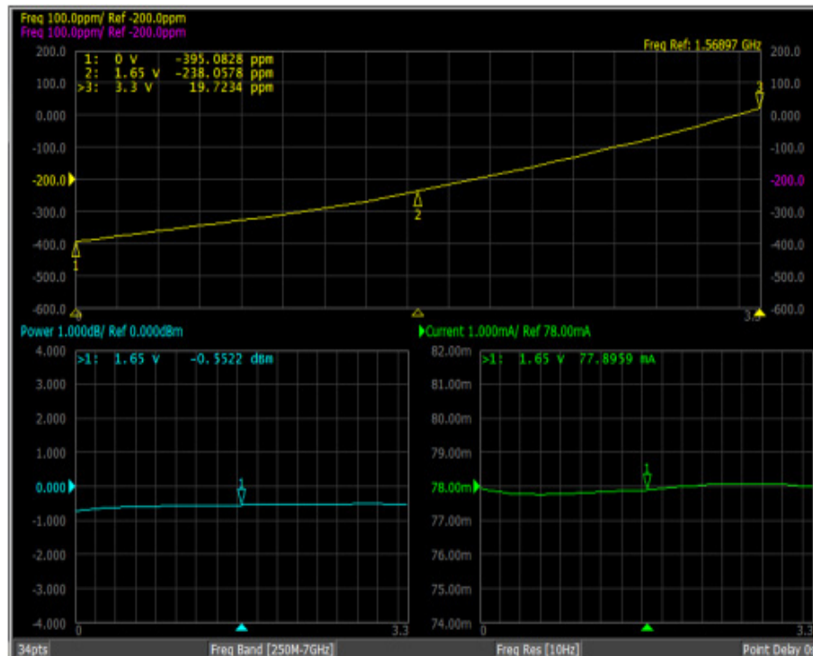
Figure 4. Vc Pull Performance Characteristics @ 1.56897 GHz
