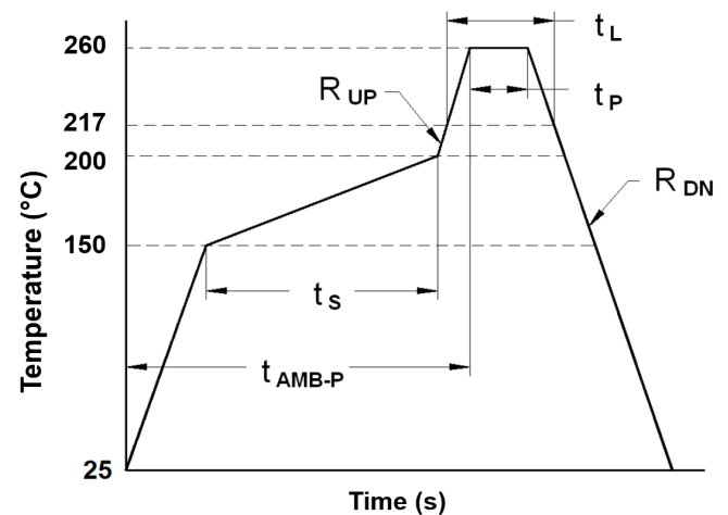
Figure 9. Recommended Reflow Profile (Not to scale)
