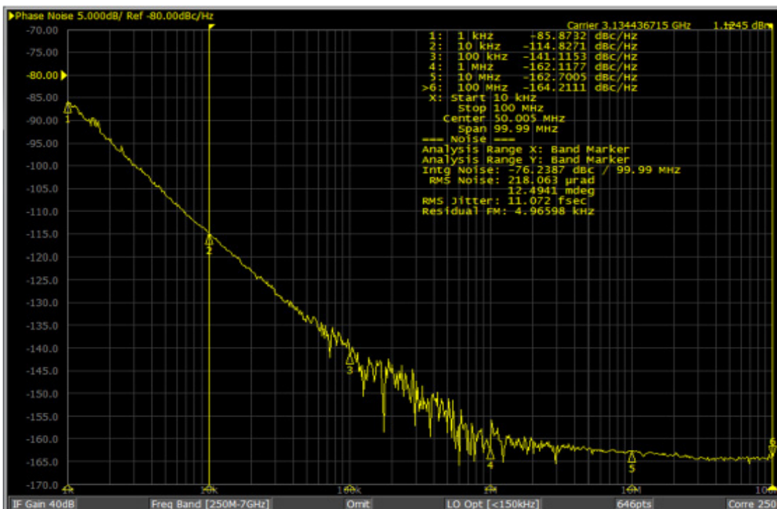
Figure 8. Typical Phase Noise Performance @ 3.13794 GHz
