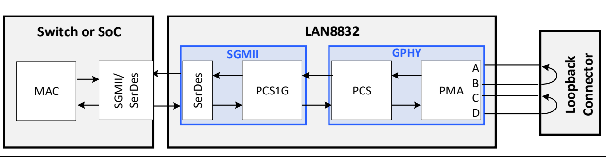
FIGURE 5-7: EXTERNAL CONNECTOR LOOPBACK
