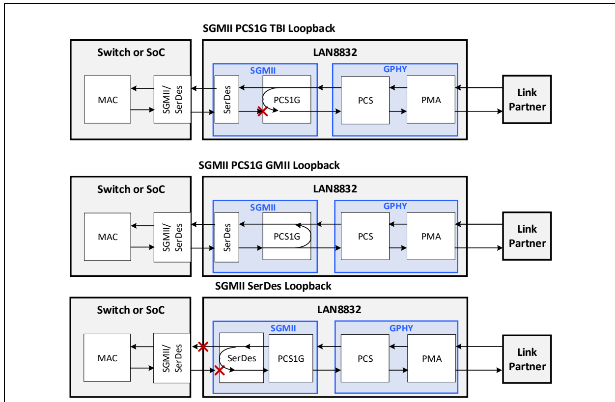
FIGURE 5-8: SGMII LOOPBACK
