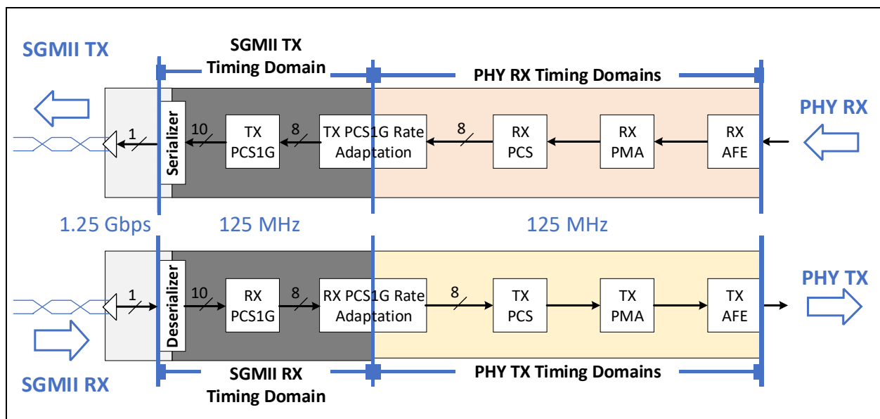
FIGURE 5-2: SGMII SYSTEM DIAGRAM
