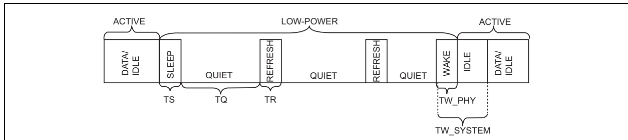
FIGURE 5-4: LPI MODE (REFRESH TRANSMISSIONS AND QUIET PERIODS)
