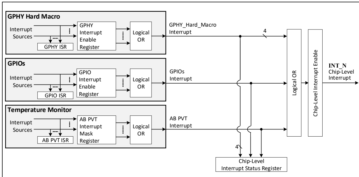
FIGURE 5-9: INTERRUPT STRUCTURE
