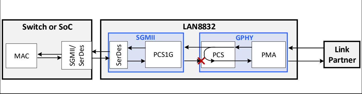
FIGURE 5-6: REMOTE (FAR-END) LOOPBACK
