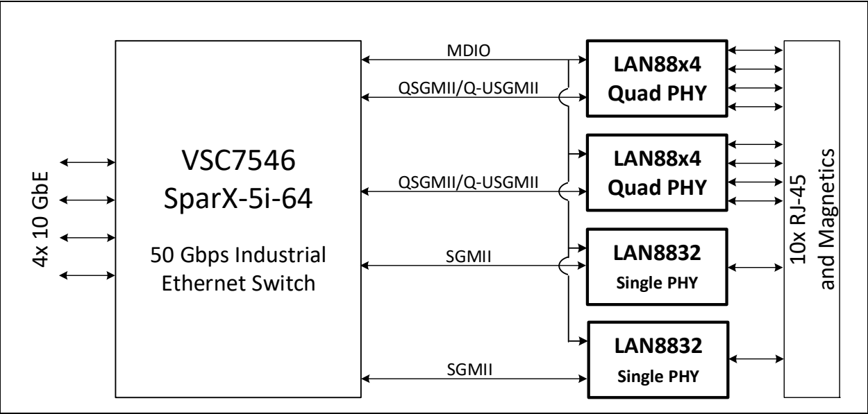
FIGURE 2-2: SWITCH APPLICATION
