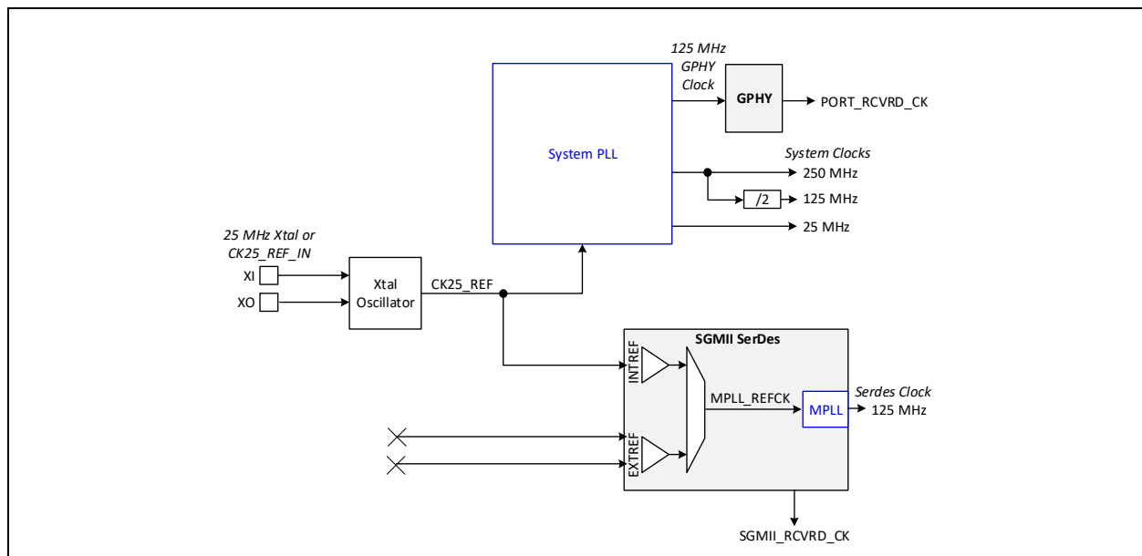
FIGURE 5-3: LAN8832 CLOCKS
