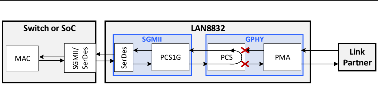
FIGURE 5-5: DIGITAL (NEAR-END) LOOPBACK
