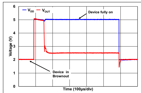
FIGURE 2-43: Brownout Recovery.
