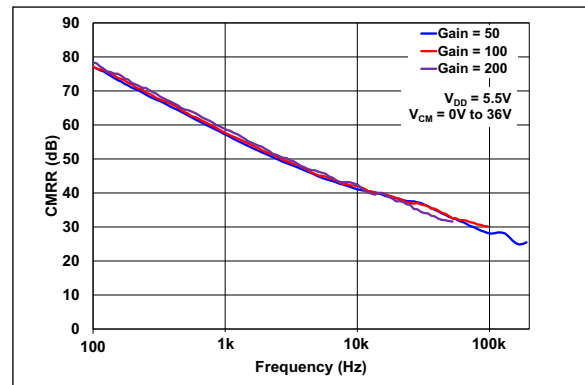
FIGURE 4: CMRR vs. Frequency.
