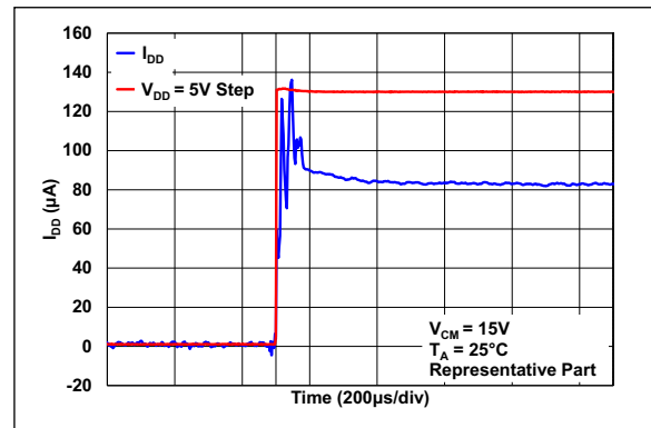
FIGURE 2-47: Supply Current During Power Up.
