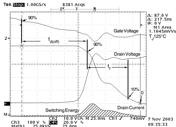
Figure 19, Turn-on Switching Waveforms and Definitions
