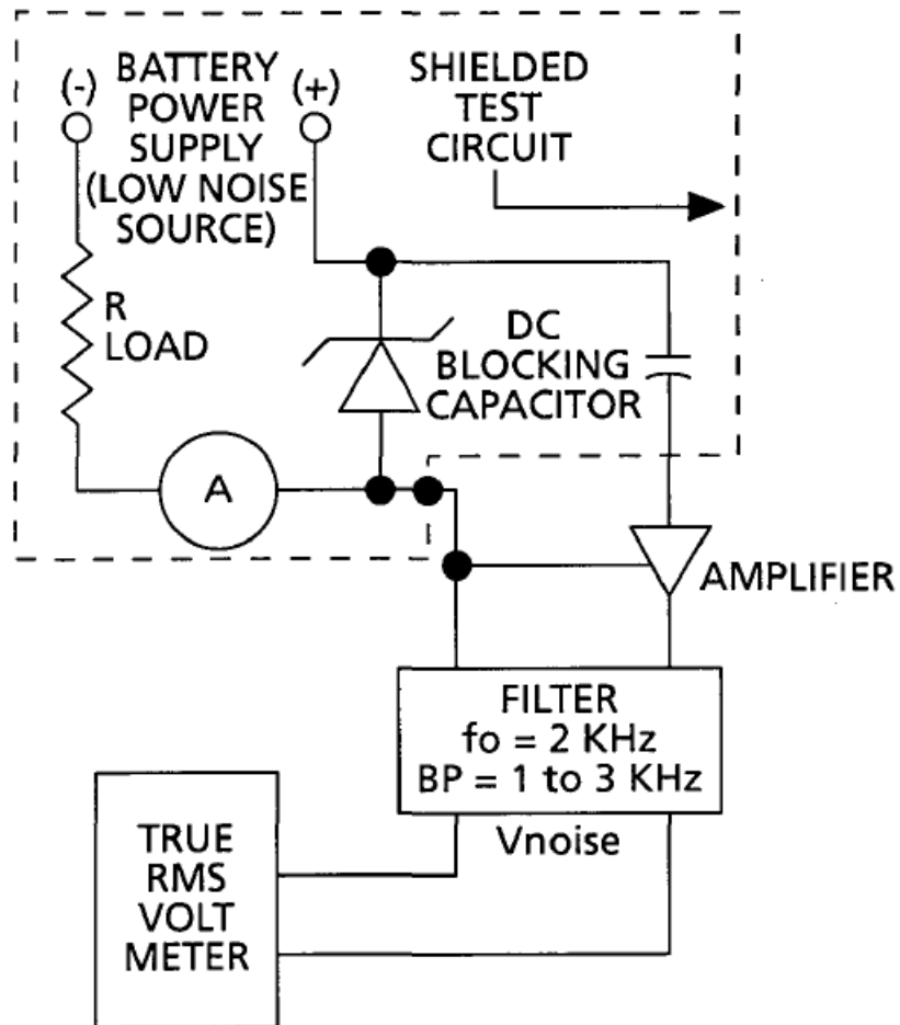
Figure 4-1. Noise Density Measurement Circuit
