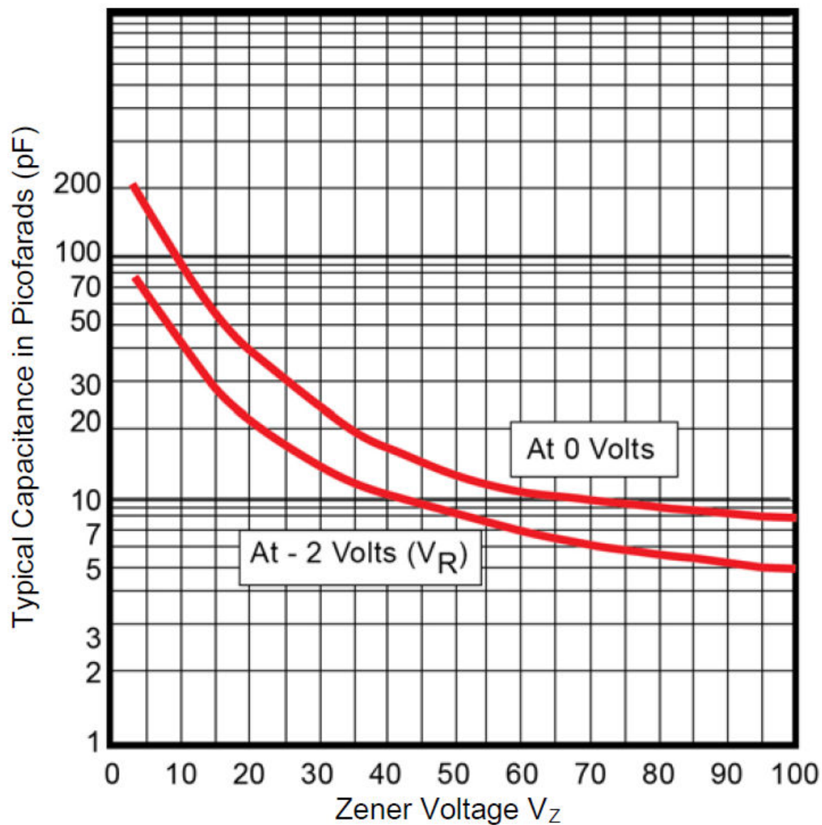
Figure 4-3. Capacitance vs. Zener Voltage (Typical)
