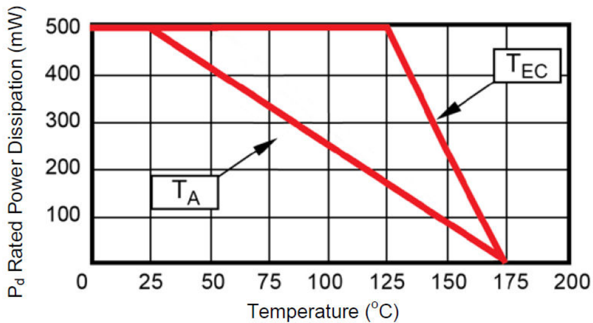
Figure 4-2. Power Derating Curve
