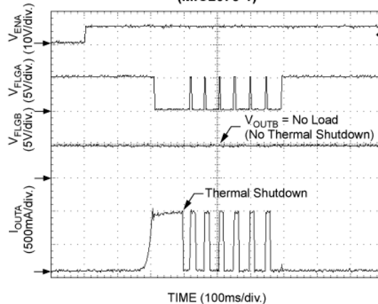
Independent Thermal Shutdown (MIC2073-1)
