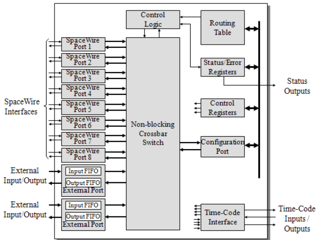
Figure 1-1. SpaceWire Router Block Diagram
