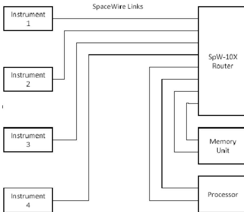
Figure 2-1. AT7910E as SpaceWire router
