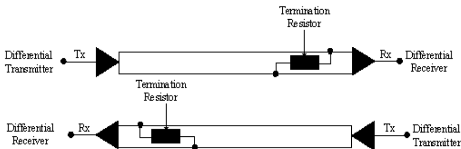
Figure 4-1. LVDS communication principle
