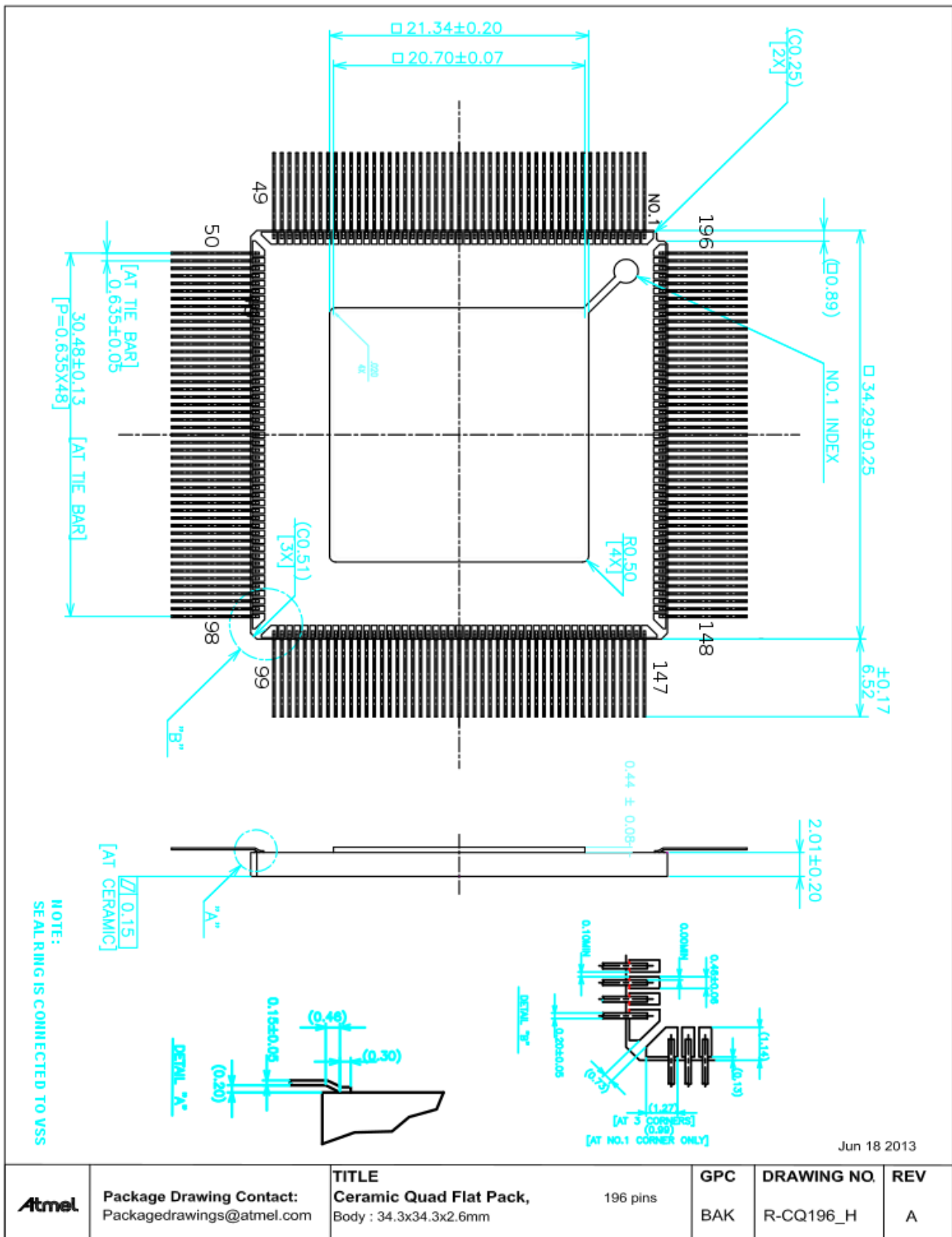
Figure 7-1. MQFPF 196 package
