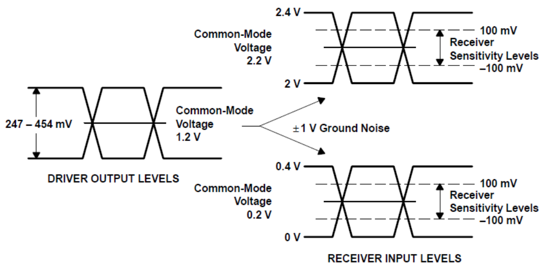
Figure 5-2. Transmitter to Receiver Electrical Characteristics
