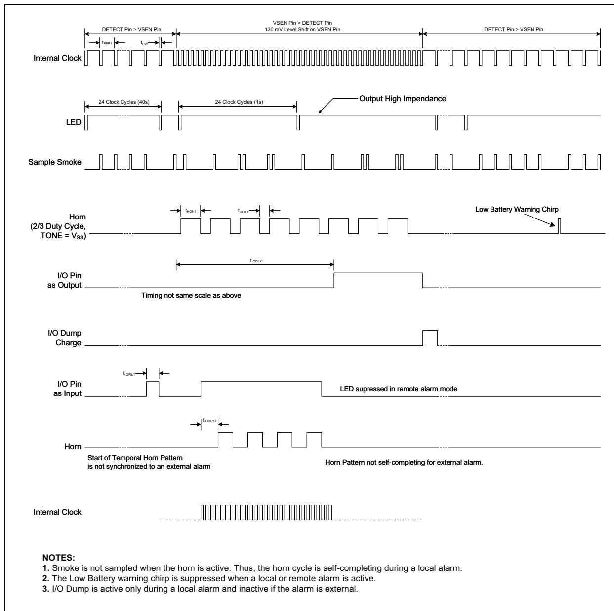
FIGURE 3-1: RE46C129 Timing Diagram.
