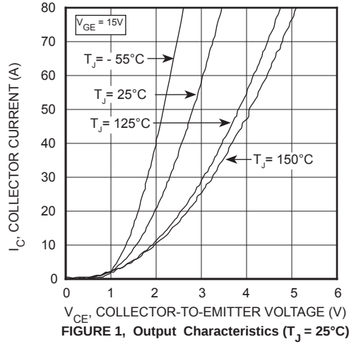
FIGURE 1, Output Characteristics ( T_J = 25^\circ C )
