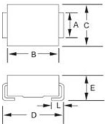
Figure 4-2. SMCJ (DO-214AB)
