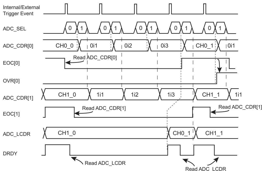
Figure 45-8. Digital Averaging Function Waveforms Over Multiple Trigger Events
