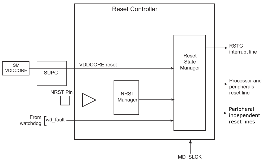
Figure 24-1. Reset Controller Block Diagram
