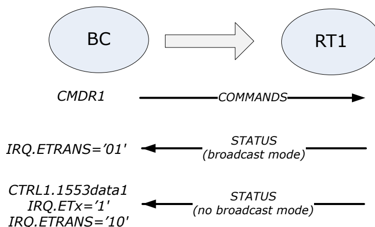
Figure 35-9. Command Frame Transfer
