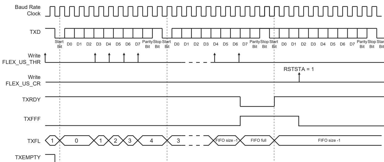
Figure 37-39. TXRDY in Single Data Mode and TXRDYM = 0
