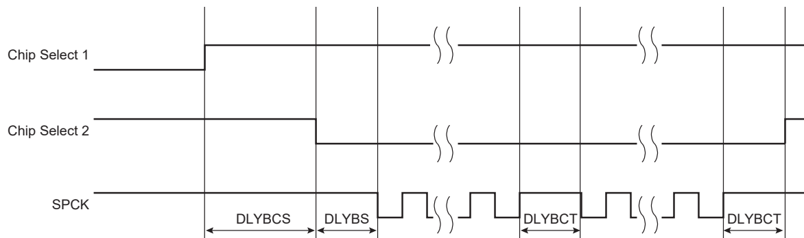
Figure 37-47. Programmable Delays
