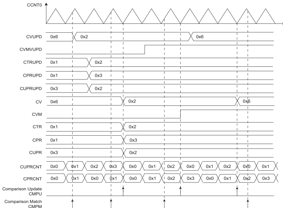
Figure 40-24. Comparison Waveform
