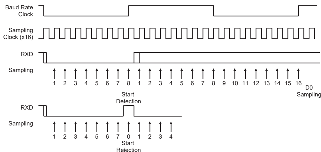
Figure 37-10. Asynchronous Start Detection
