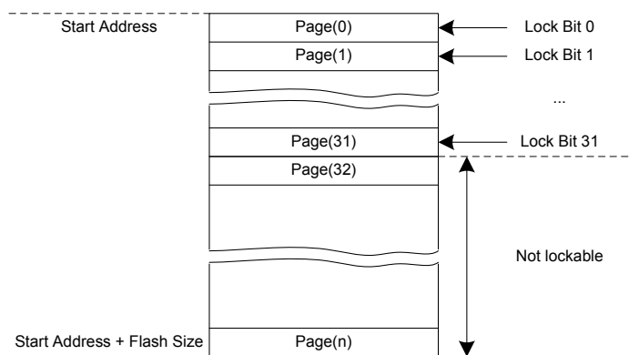
Figure 20-4. Flash Memory Plane Lockable Region
