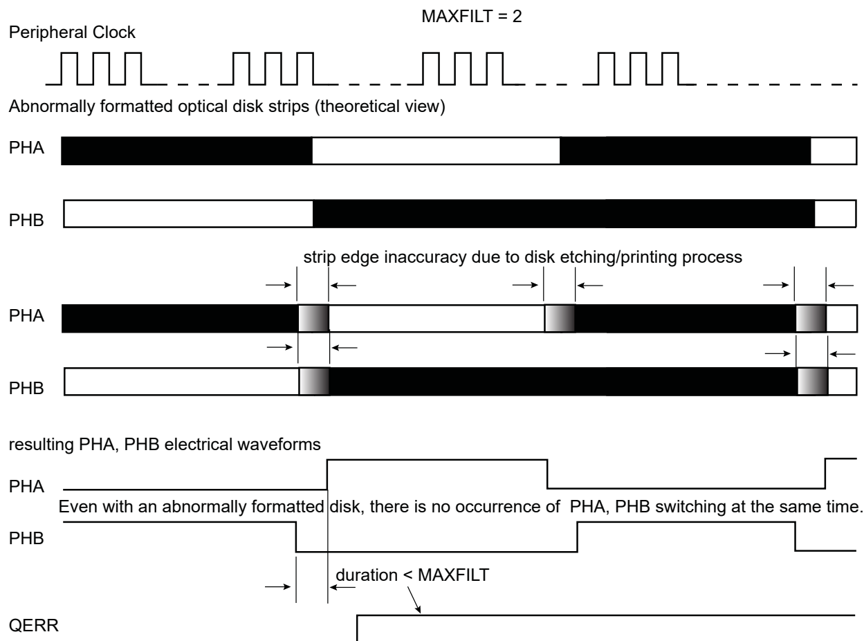
Figure 39-21. Quadrature Error Detection
