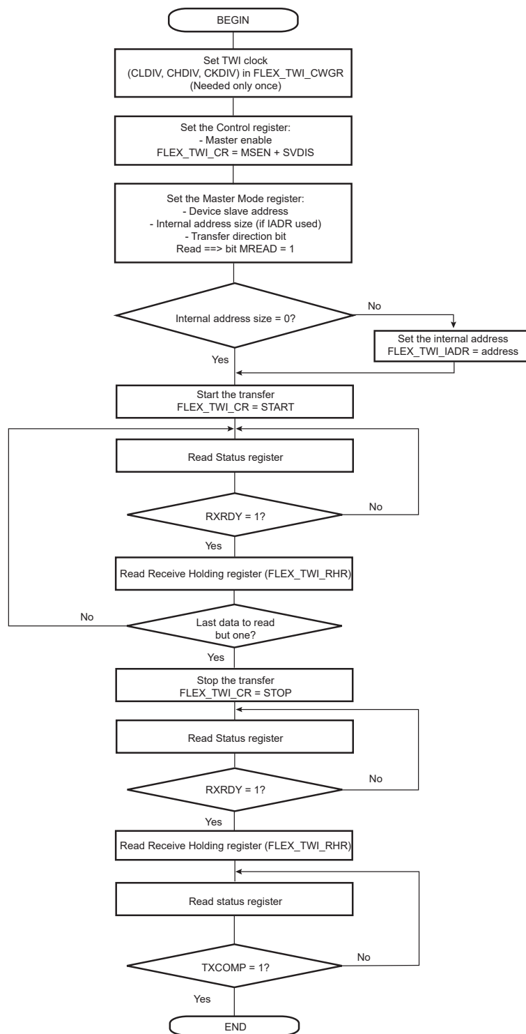
Figure 37-78. TWI Read Operation with Multiple Data Bytes with or without Internal Address
