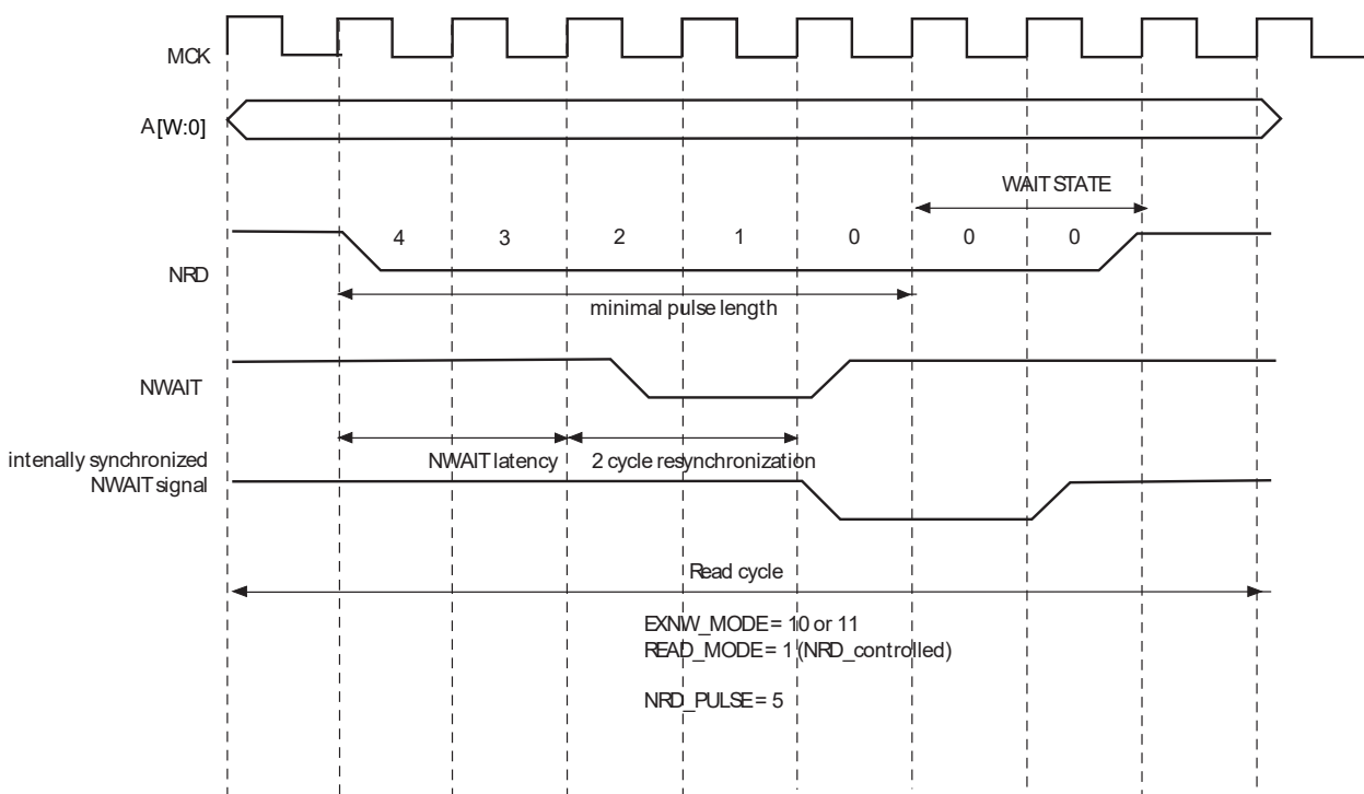
Figure 32-17. NWAIT Latency
