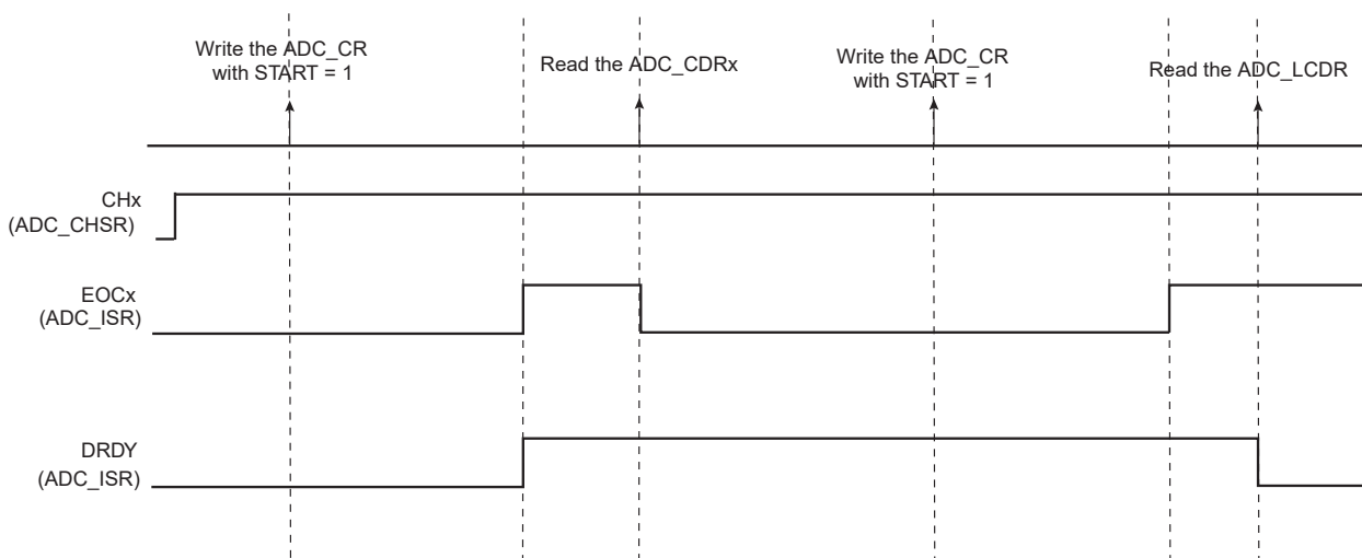
Figure 45-4. EOCx and DRDY Flag Behavior
