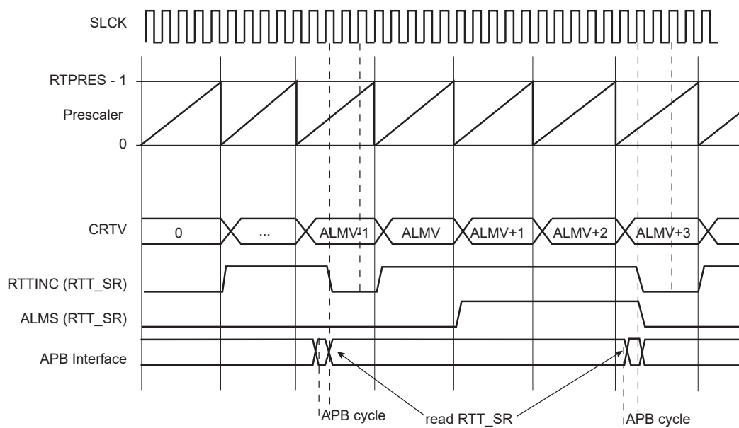
Figure 26-2. RTT Counting
