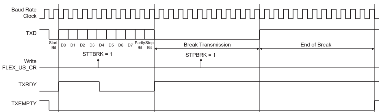
Figure 37-24. Break Transmission
