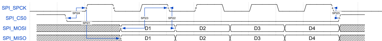
Figure 50-14. FlexCom—SPI Timings - Slave Mode (CPOL=0 and NCPHA=0 OR CPOL=0 and NCPHA=0)
