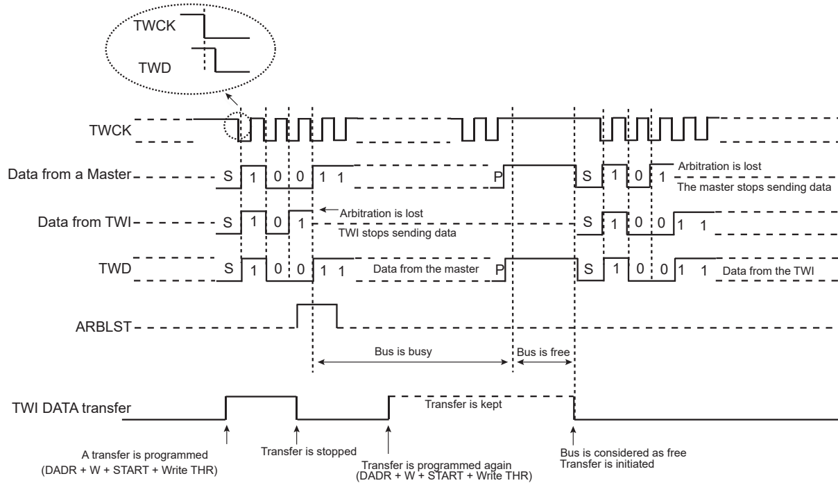
Figure 37-84. Arbitration Cases
