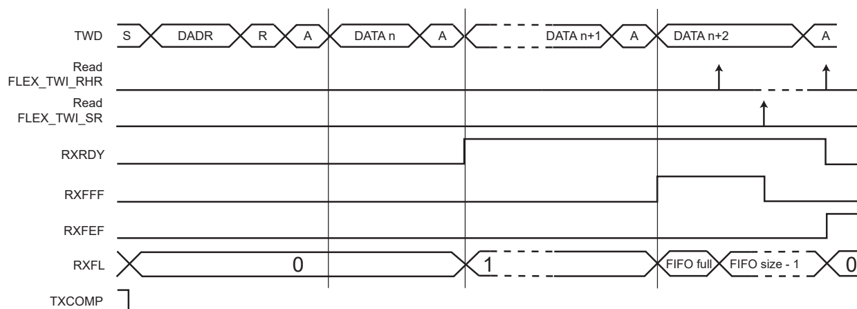
Figure 37-102. RXRDY Behavior when RXRDYM = 0 in Master and Slave Modes
