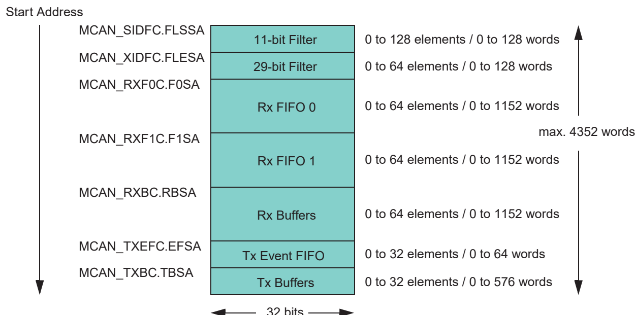
Figure 38-12. Message RAM Configuration
