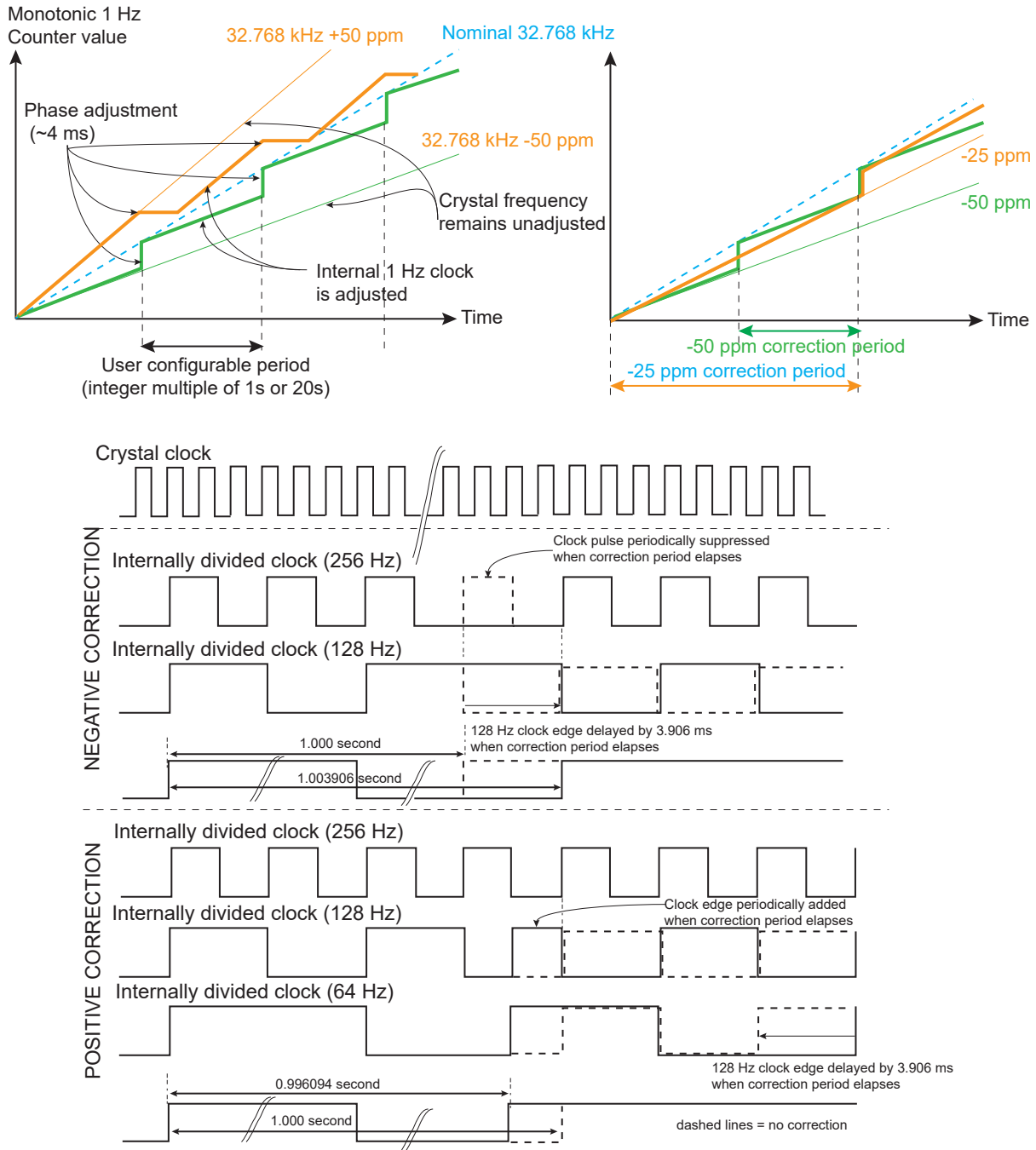
Figure 25-5. Calibration Circuitry Waveforms
