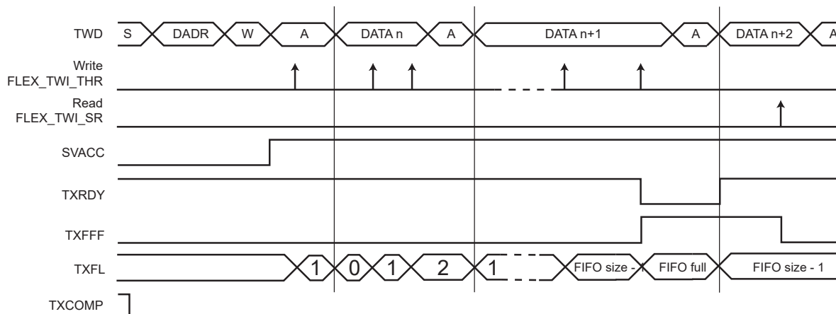
Figure 37-103. TXRDY Behavior when TXRDYM = 0 in Slave Mode
