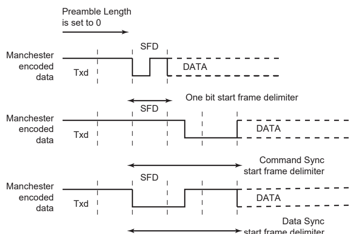
Figure 37-8. Start Frame Delimiter
