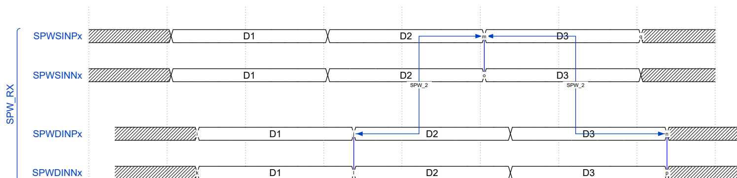
Figure 50-8. SPW RX Characteristics (LVDS Mode)
