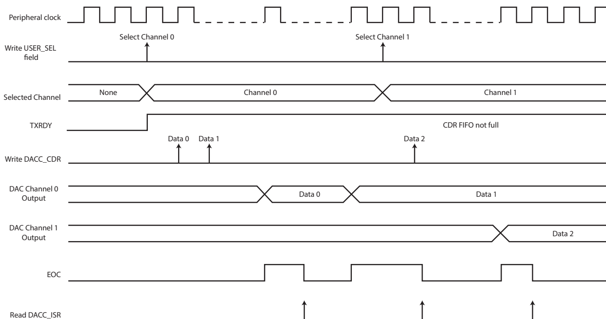
Figure 46-2. Conversion Sequence
