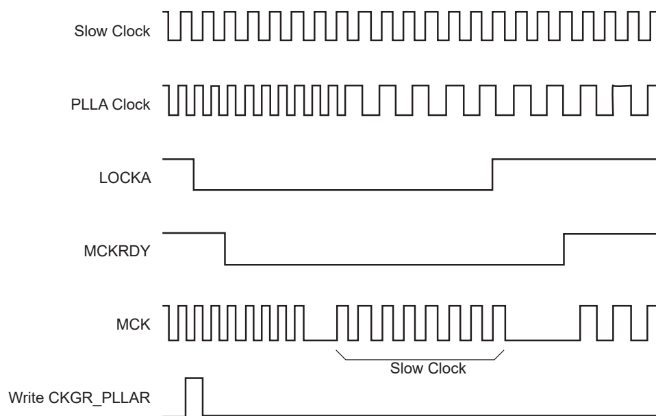
Figure 28-6. Change PLLA Programming
