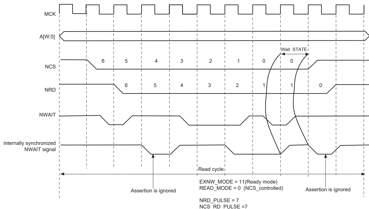
Figure 32-16. NWAIT Assertion in Read Access: Ready Mode (HSMC_MODE.EXNW_MODE = 11)
