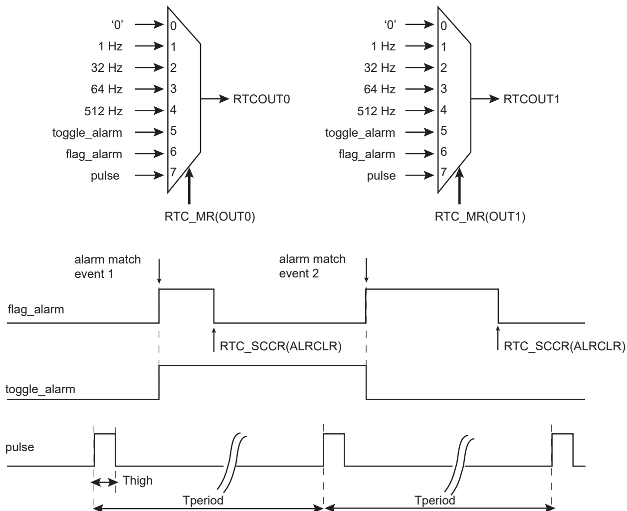
Figure 25-6. Waveform Generation
