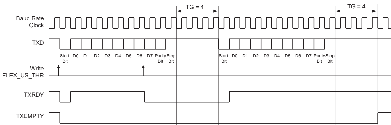
Figure 37-21. Timeguard Operations
