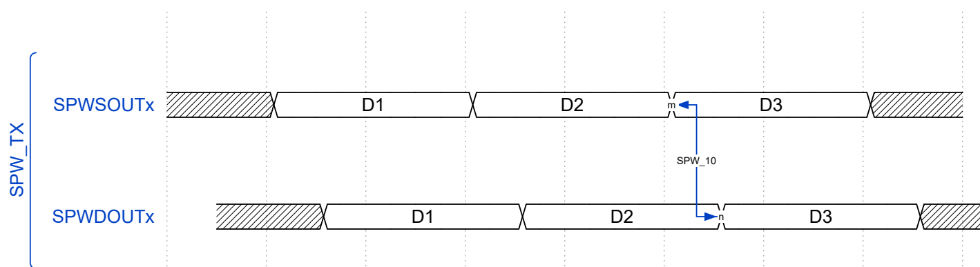
Figure 50-11. SPW TX Characteristics (TTL Mode)
