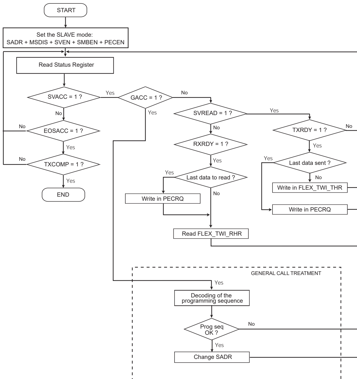
Figure 37-95. Read/Write in Slave Mode with SMBus PEC
