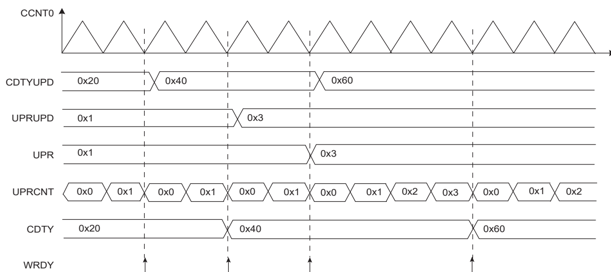
Figure 40-20. Method 2 (UPDM = 1)
