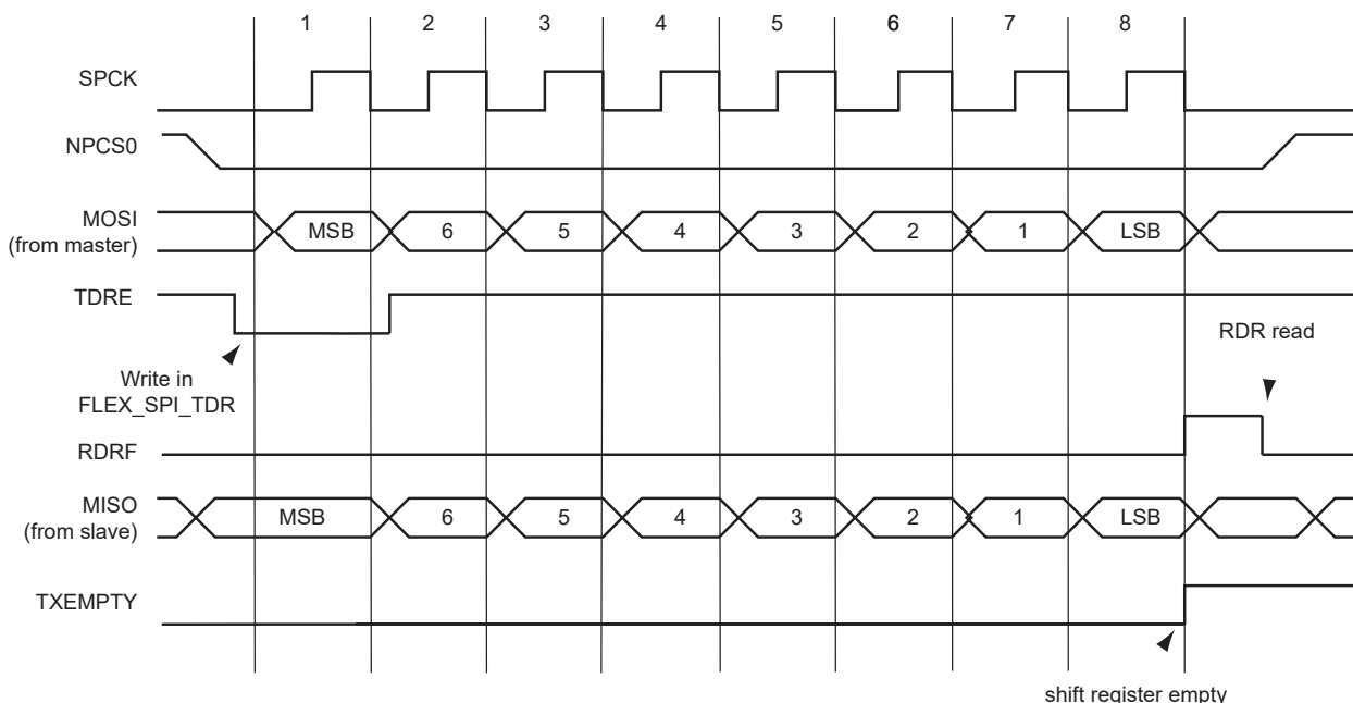
Figure 37-46. Status Register Flags Behavior
