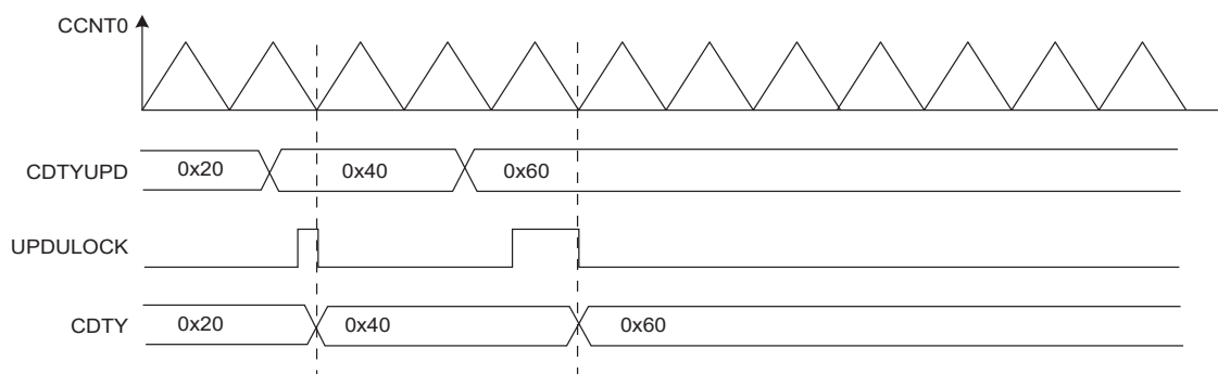
Figure 40-19. Method 1 (UPDM = 0)
