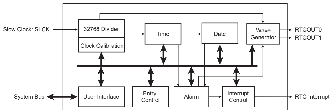
Figure 25-1. Real-time Clock Block Diagram
