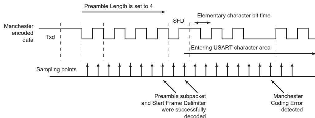
Figure 37-14. Manchester Error Flag
