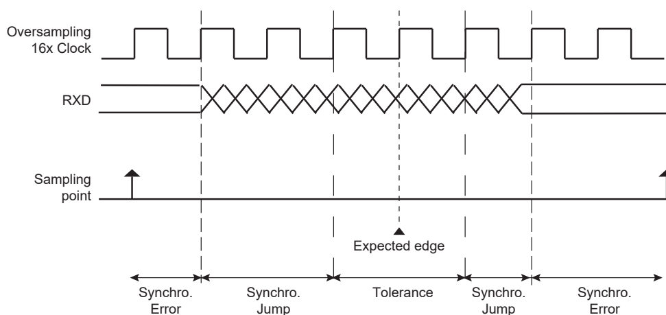
Figure 37-9. Bit Resynchronization
