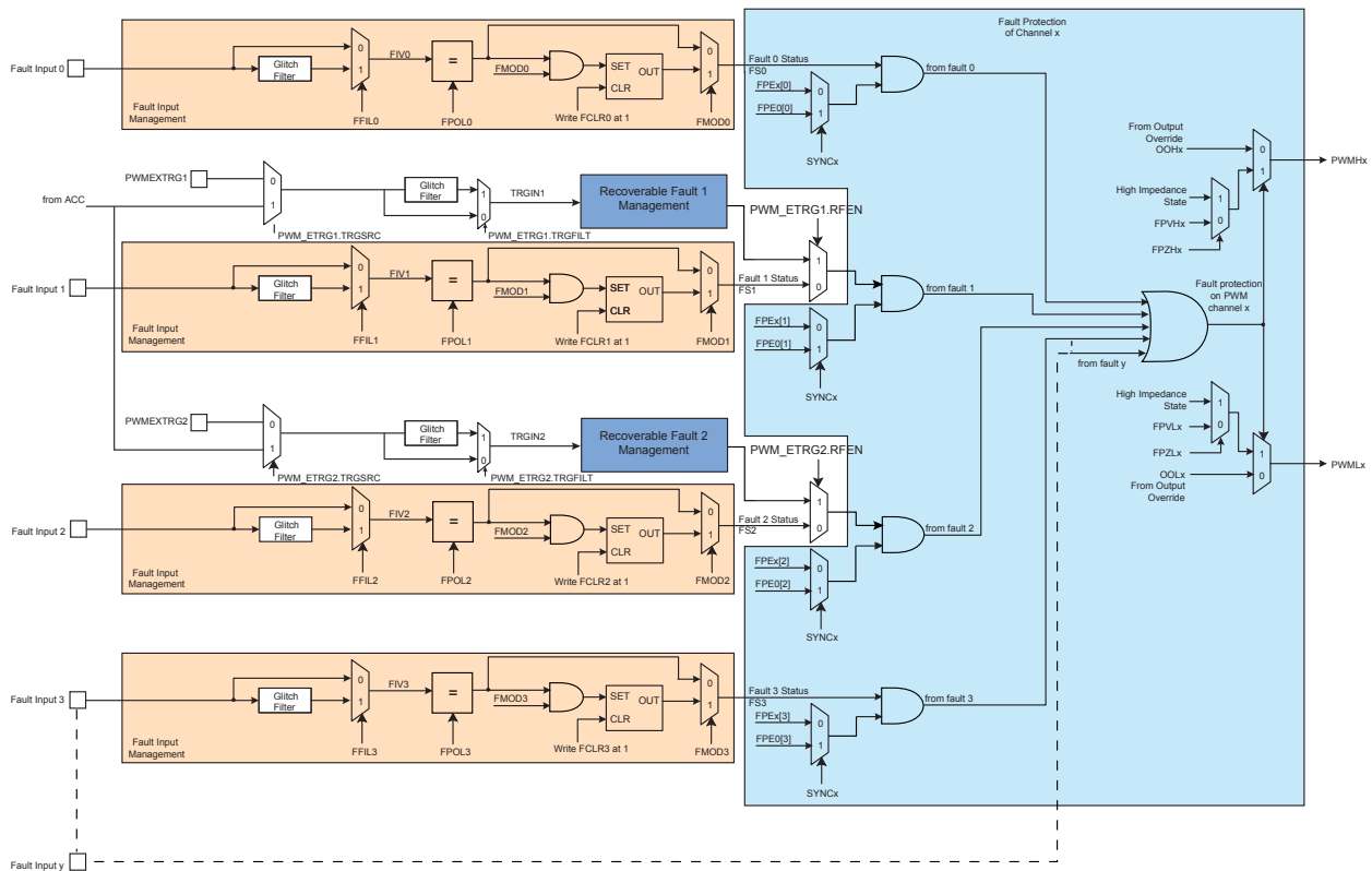
Figure 40-16. Fault Protection
