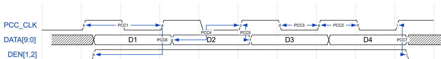
Figure 50-21. PCC Characteristics
