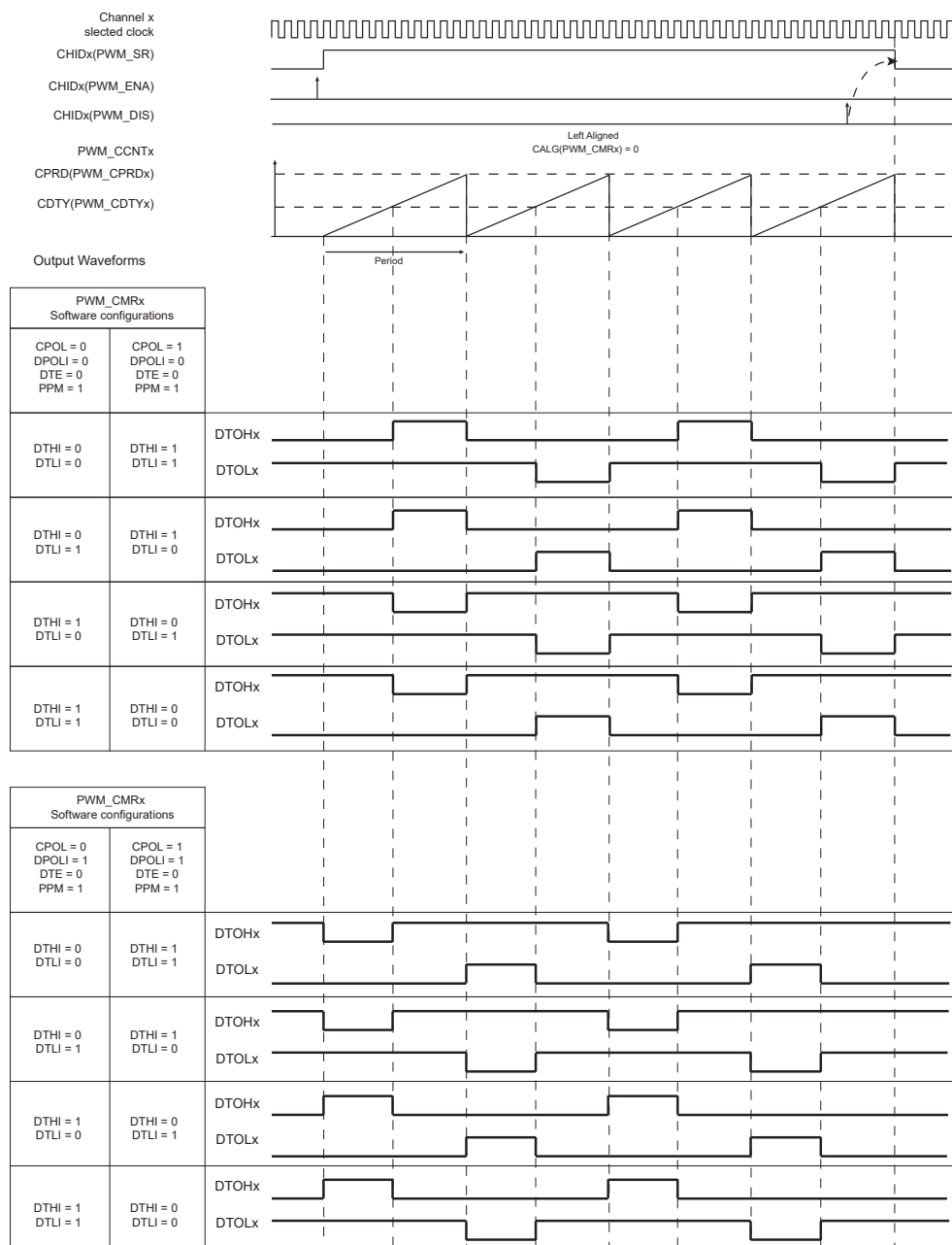
Figure 40-11. PWM Push-Pull Waveforms: Left-Aligned Mode
