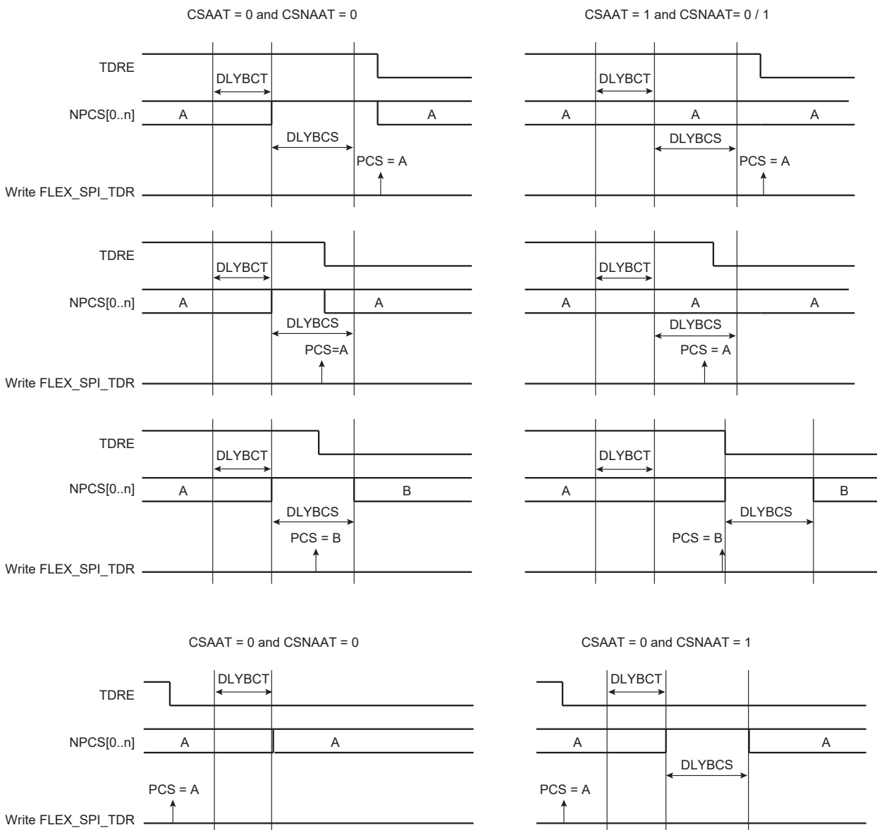
Figure 37-49. Peripheral Deselection
