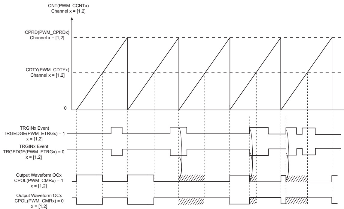
Figure 40-31. Cycle-By-Cycle Duty Mode
