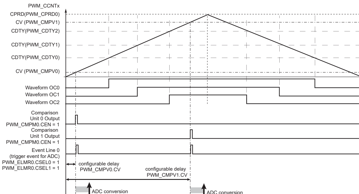
Figure 40-26. Event Line Generation Waveform (Example)
