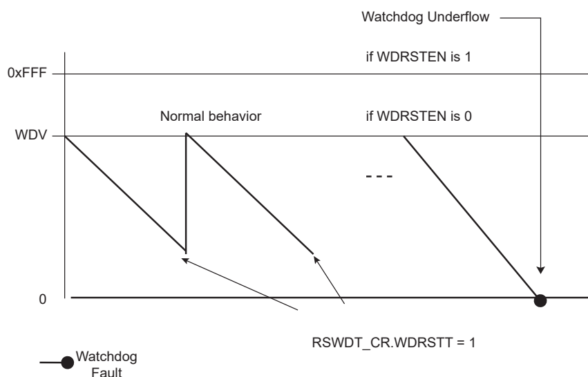
Figure 23-2. Watchdog Behavior
