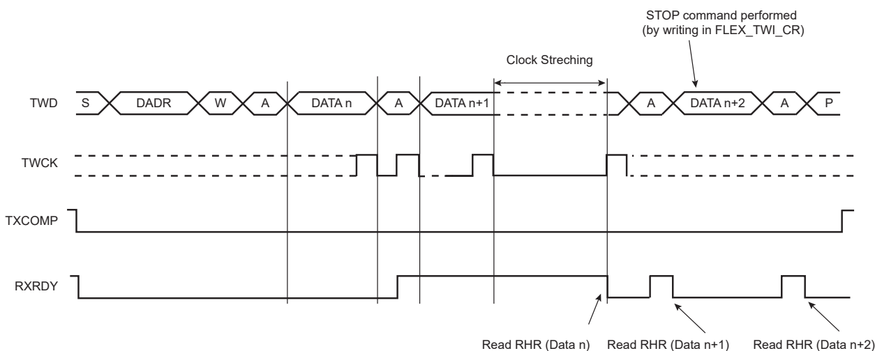
Figure 37-64. Master Read Clock Stretching with Multiple Data Bytes
