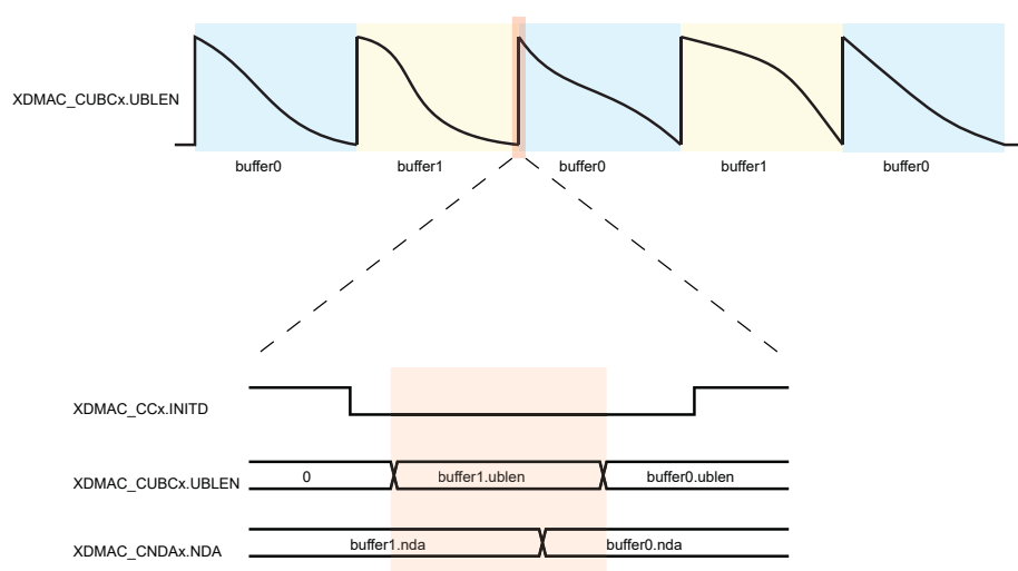
Figure 34-4. INITD Timing Diagram
