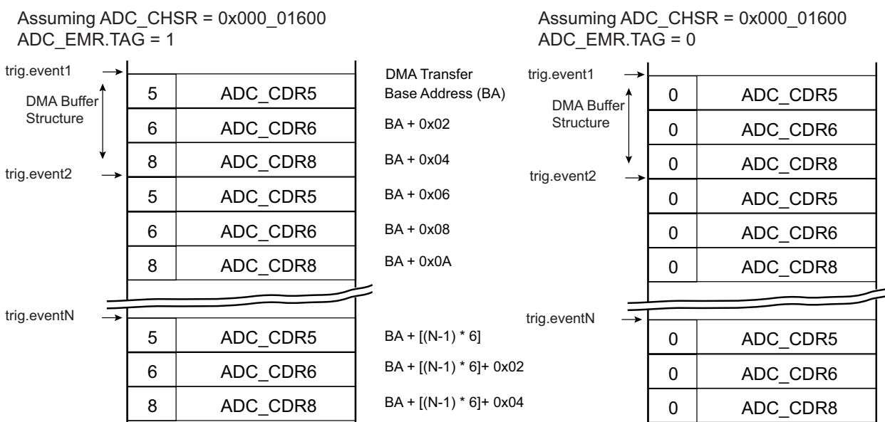
Figure 45-11. Buffer Structure
