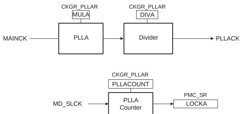
Figure 27-3. Divider and PLLA Block Diagram
