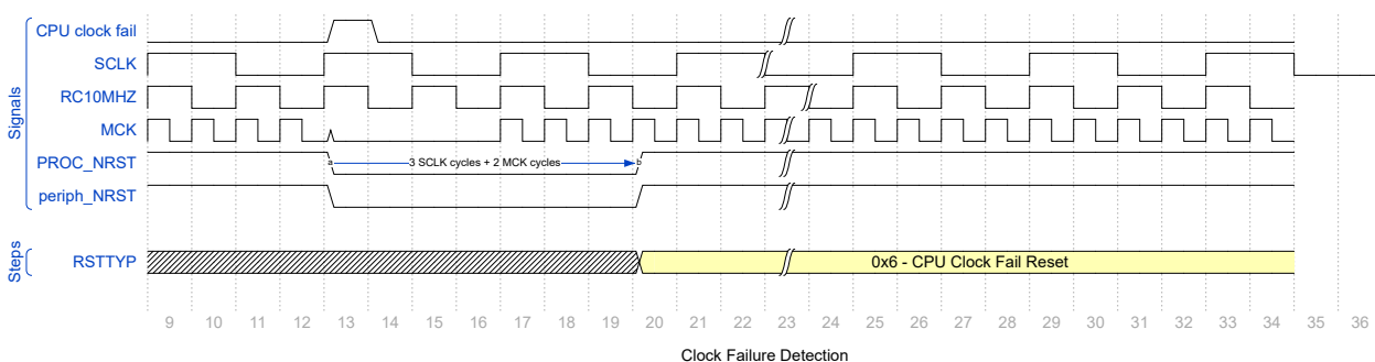
Figure 24-4. CPU Clock Failure Detection Reset Timing Diagram
