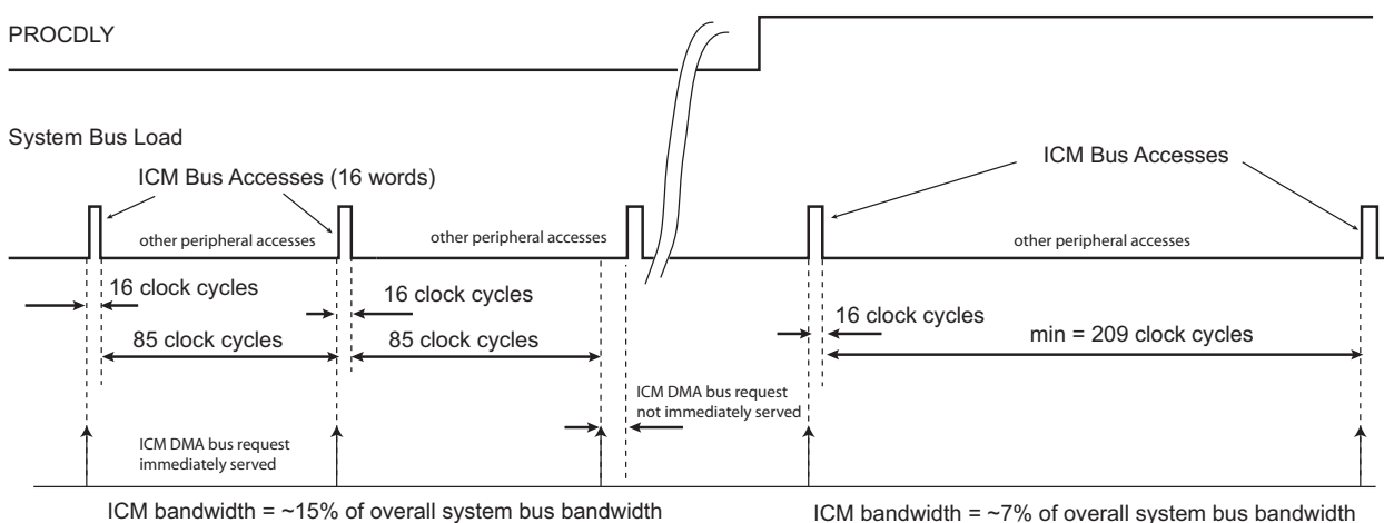
Figure 41-6. Bandwidth Usage in SHA1 Mode
