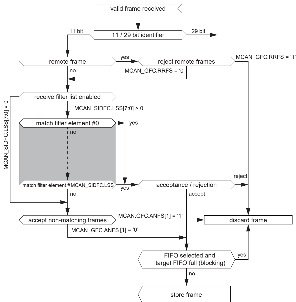
Figure 38-5. Standard Message ID Filter Path
