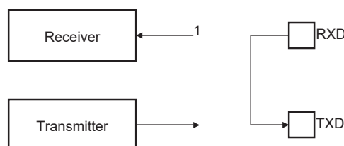
Figure 37-35. Remote Loopback Mode Configuration
