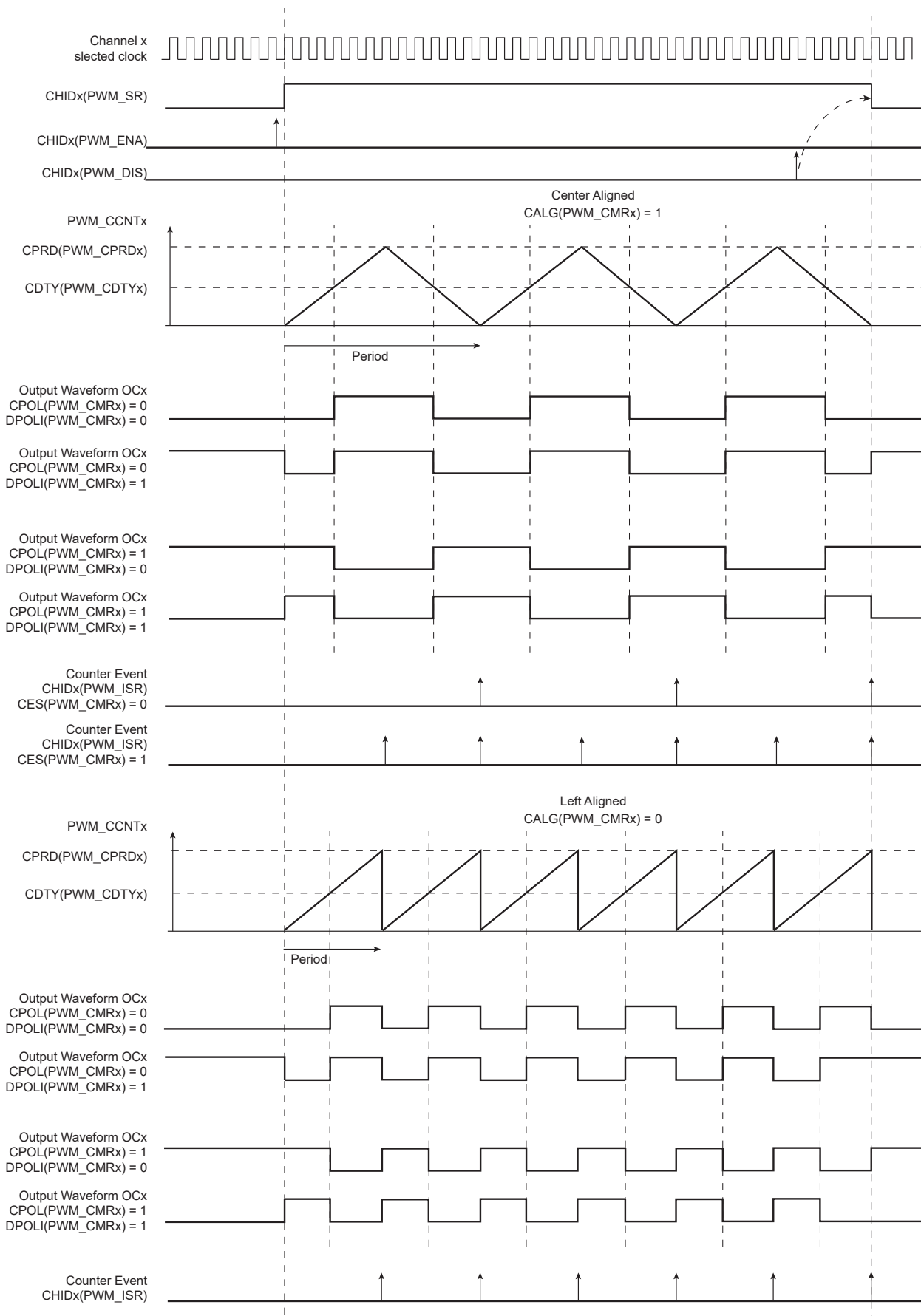
Figure 40-5. Waveform Properties
