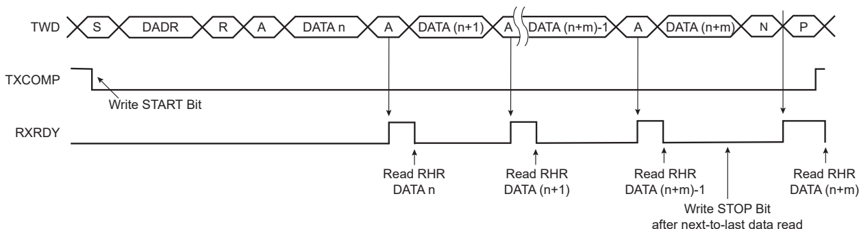
Figure 37-64. Master Read Clock Stretching with Multiple Data Bytes
