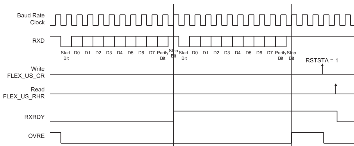
Figure 37-19. Receiver Status
