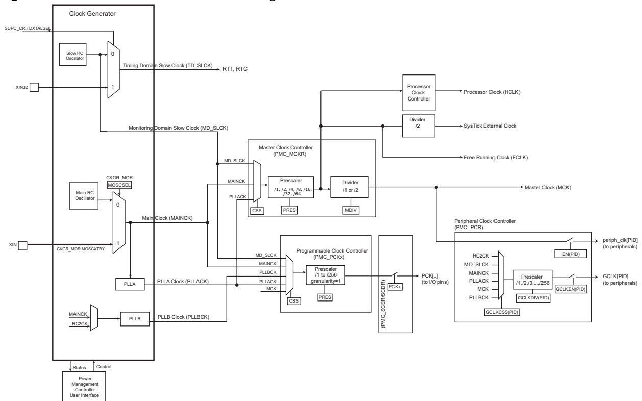
Figure 28-1. General Clock Distribution Block Diagram
