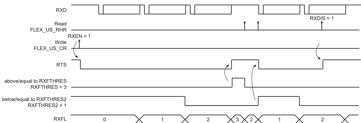
Figure 37-28. Receiver Behavior When FIFO Enabled and FRTSC Set to '1'
