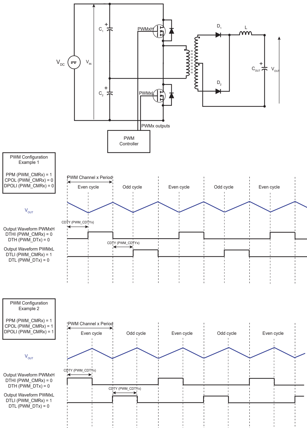
Figure 40-13. Half-Bridge Converter Application: No Feedback Regulation
