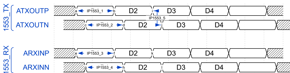
Figure 50-7. 1553 Characteristics
