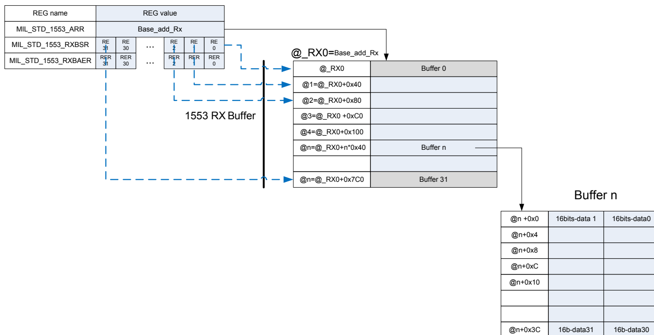
Figure 35-4. 1553 Rx Buffer
