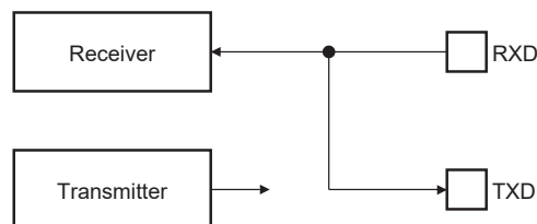
Figure 37-33. Automatic Echo Mode Configuration
