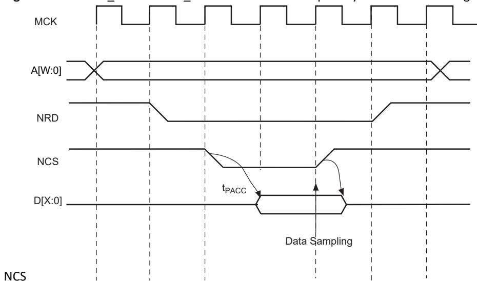
Figure 32-4. HSMC_MODE.READ_MODE = 0: Data is Sampled by HSMC on the Rising Edge of
