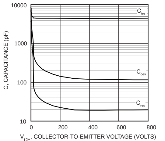
FIGURE 17, Capacitance vs Collector-To-Emitter Voltage
