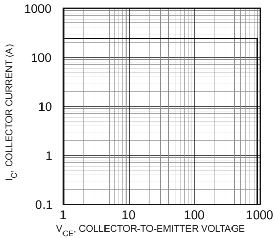
FIGURE 18, Minimum Switching Safe Operating Area
