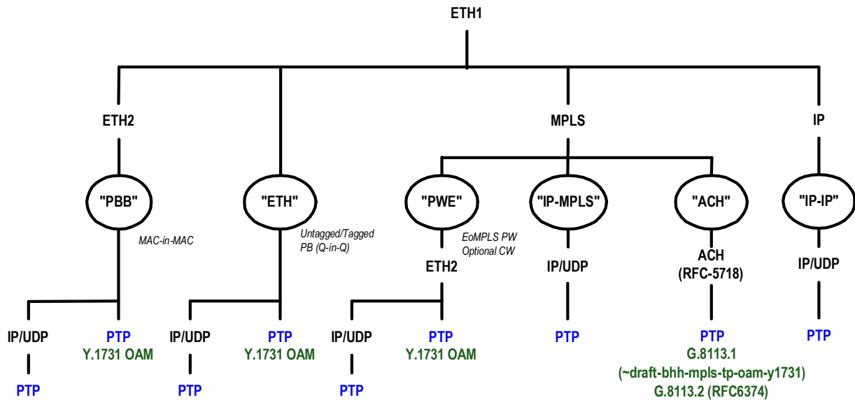
FIGURE 2-36: PTP PACKET ENCAPSULATIONS
