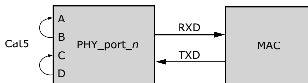
FIGURE 2-70: CONNECTOR LOOPBACK DIAGRAM
