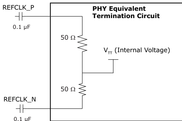
FIGURE 2-19: AC COUPLING FOR REFCLK INPUT
