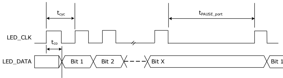
FIGURE 4-7: BASIC SERIAL LED TIMING
