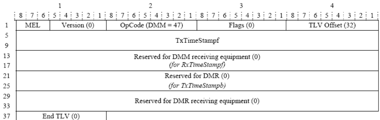
FIGURE 2-34: Y.1731 DMM PDU FORMAT
