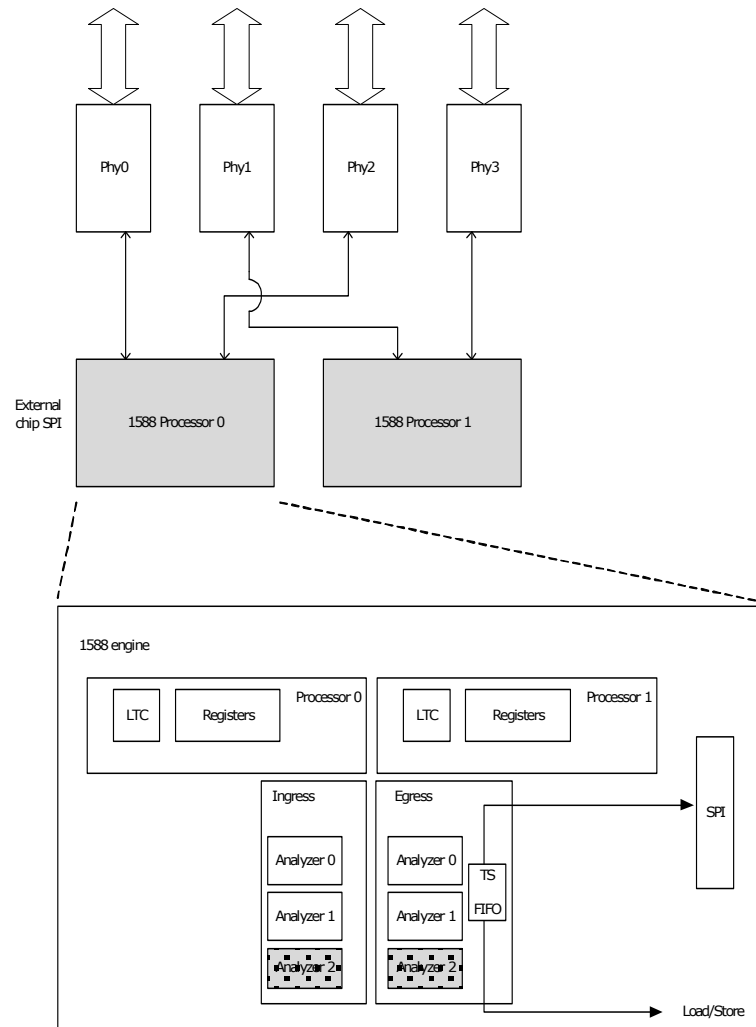
FIGURE 2-22: IEEE 1588 ARCHITECTURE
