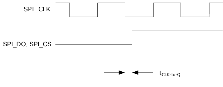
FIGURE 4-12: SERIAL TIMESTAMP INTERFACE TIMING DIAGRAM
