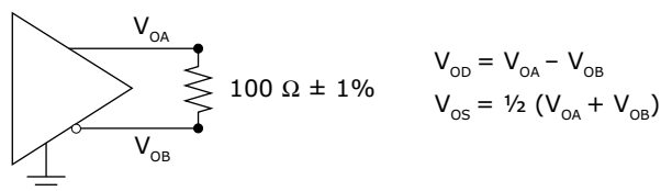
FIGURE 4-2: SGMII DC DEFINITIONS
