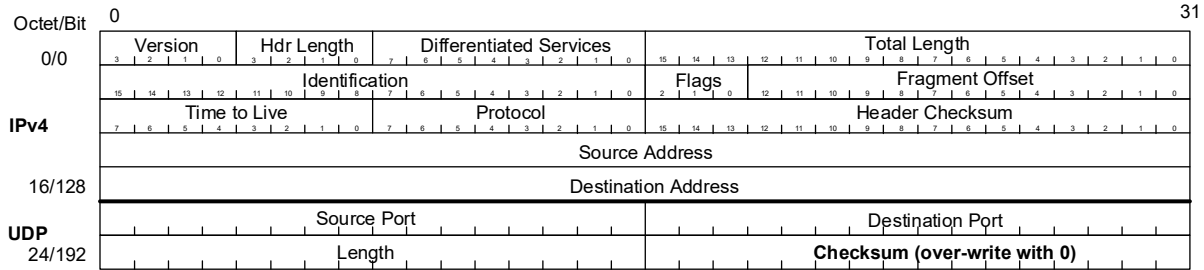
FIGURE 2-49: IPv4 WITH UDP
