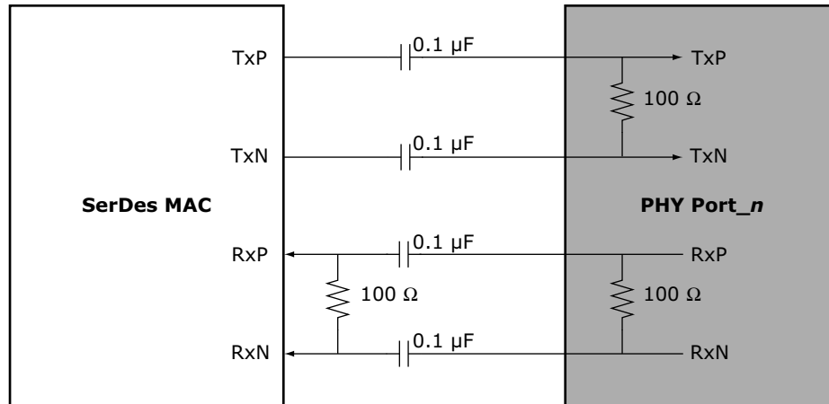
FIGURE 2-10: SERDES MAC INTERFACE
