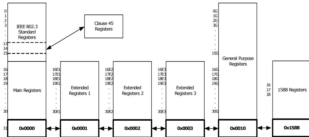
FIGURE 3-1: REGISTER SPACE DIAGRAM
