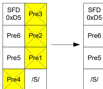
FIGURE 2-60: PREAMBLE REDUCTION IN REWRITER
