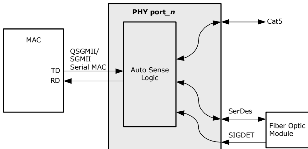
FIGURE 2-15: AUTOMATIC MEDIA SENSE BLOCK DIAGRAM
