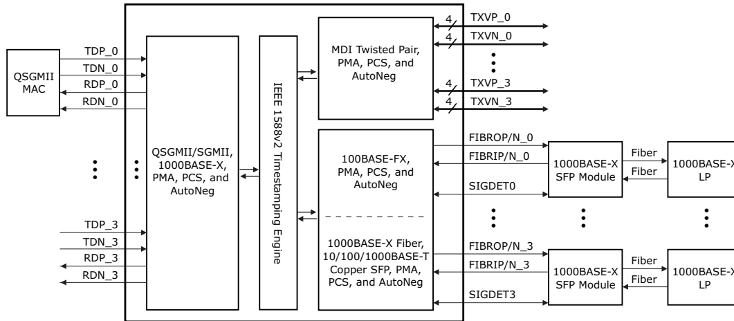
FIGURE 2-2: QSGMII MAC-TO-1000BASE-X LINK PARTNER
