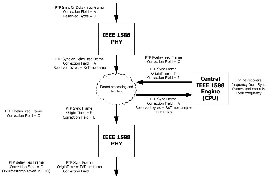
FIGURE 2-29: ONE-STEP E2E BC
