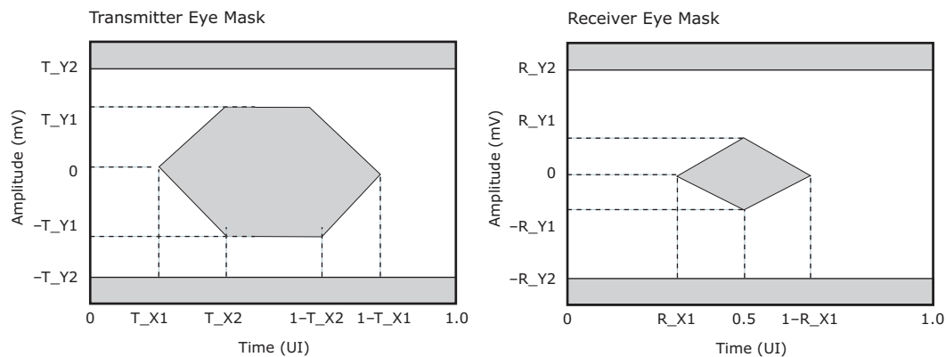
FIGURE 4-6: QSGMII TRANSIENT PARAMETERS
