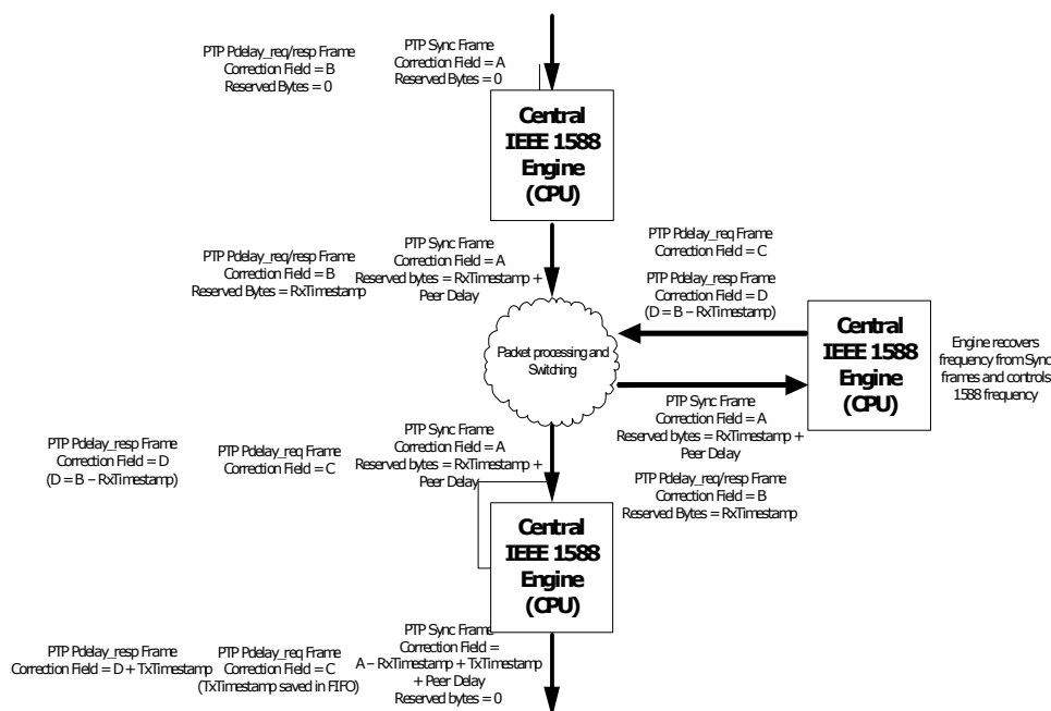
FIGURE 2-28: ONE-STEP P2P TC STANDARD
