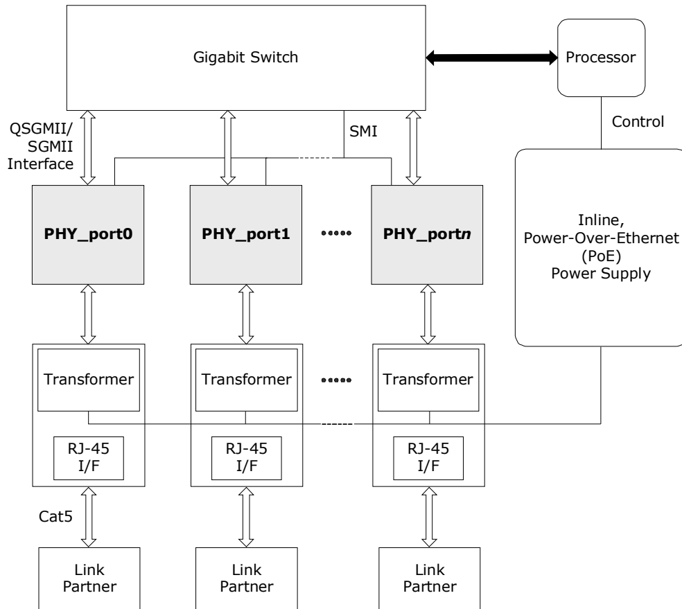
FIGURE 2-20: INLINE POWERED ETHERNET SWITCH DIAGRAM
