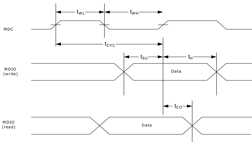
FIGURE 4-11: SERIAL MANAGEMENT INTERFACE TIMING
