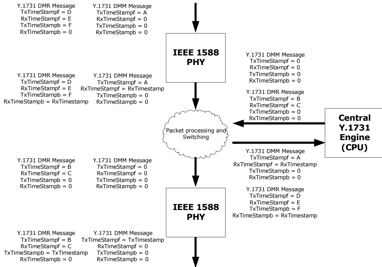
FIGURE 2-35: Y.1731 TWO-WAY DELAY
