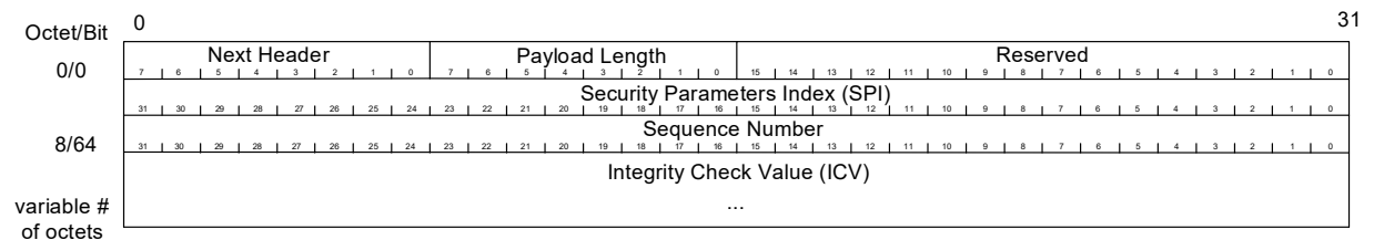
FIGURE 2-53: IPSEC HEADER FORMAT
