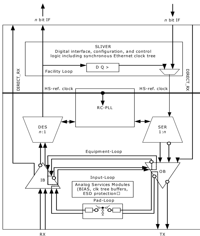
FIGURE 2-71: DATA LOOPS OF THE SERDES MACRO
