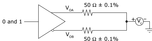
FIGURE 4-3: SGMII DC DRIVER OUTPUT IMPEDANCE TEST CIRCUIT
