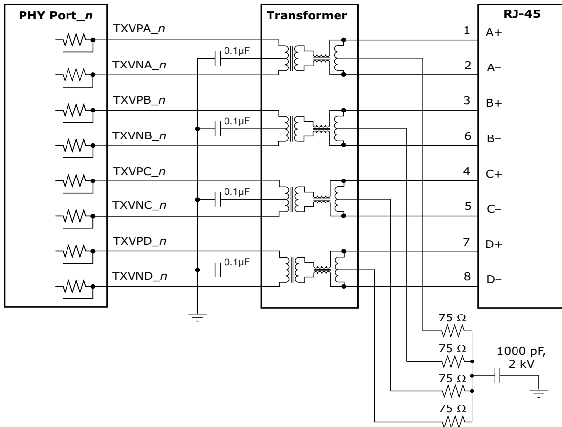
FIGURE 2-13: CAT5 MEDIA INTERFACE
