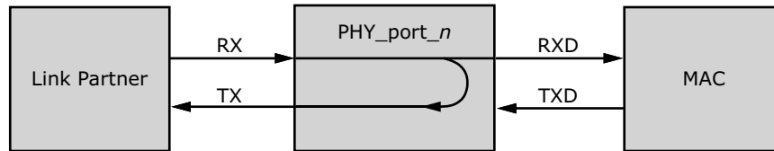
FIGURE 2-68: FAR-END LOOPBACK DIAGRAM
