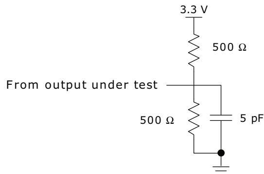
FIGURE 4-10: TEST CIRCUIT FOR TDO DISABLE TIME
