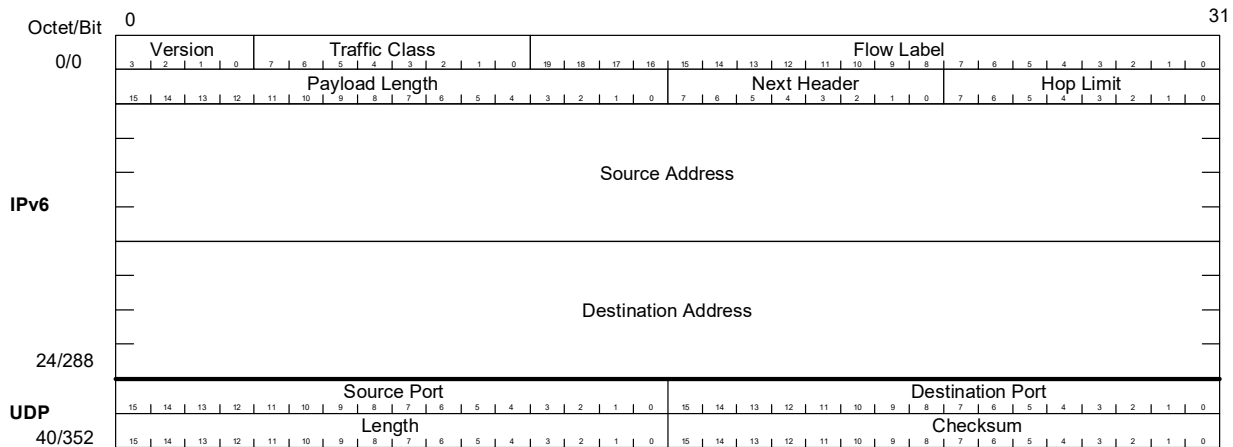
FIGURE 2-50: IPv6 WITH UDP
