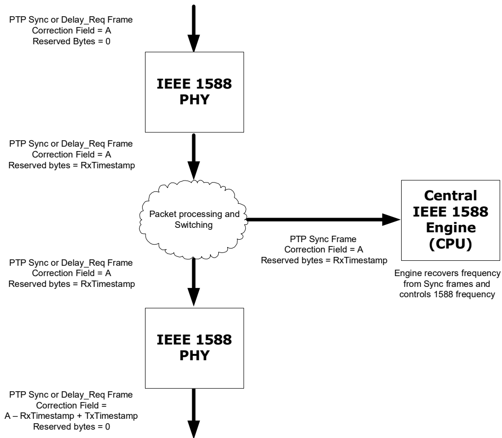
FIGURE 2-24: ONE-STEP E2E TC MODE B
