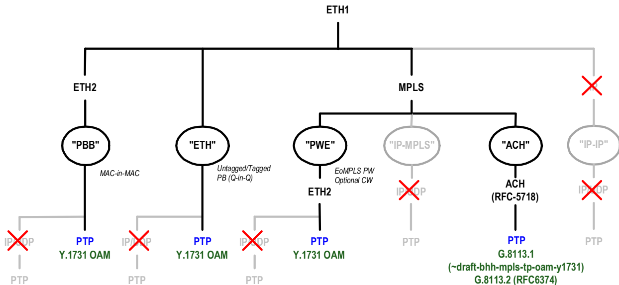
FIGURE 2-37: OAM PACKET ENCAPSULATIONS
