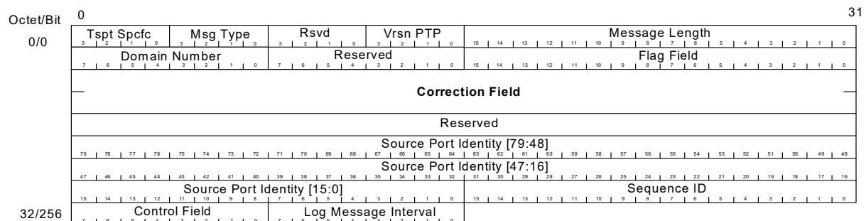
FIGURE 2-55: PTP FRAME LAYOUT
