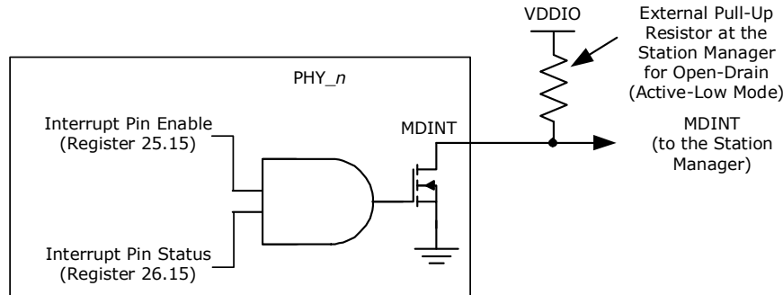
FIGURE 2-64: MDINT CONFIGURED AS AN OPEN-DRAIN (ACTIVE-LOW) PIN
