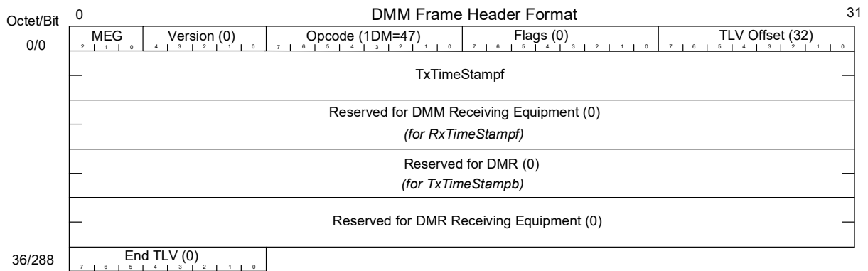
FIGURE 2-57: OAM DMM FRAME HEADER FORMAT
