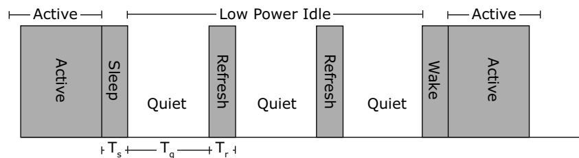
FIGURE 2-14: LOW POWER IDLE OPERATION
