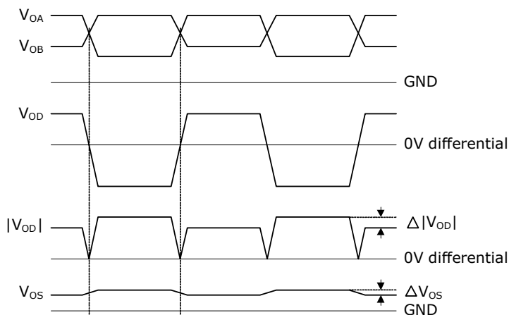
FIGURE 4-2: SGMII DC DEFINITIONS
