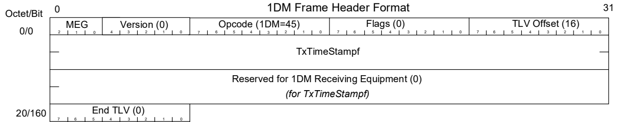
FIGURE 2-56: OAM 1DM FRAME HEADER FORMAT
