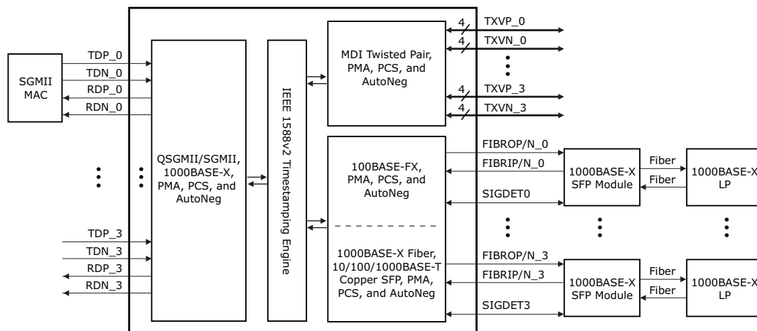
FIGURE 2-1: SGMII MAC-TO-1000BASE-X LINK PARTNER
