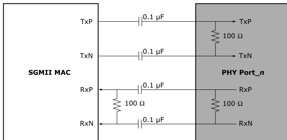
FIGURE 2-11: SGMII MAC INTERFACE
