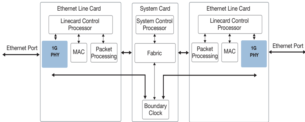
FIGURE 2-26: BC LINECARD APPLICATION
