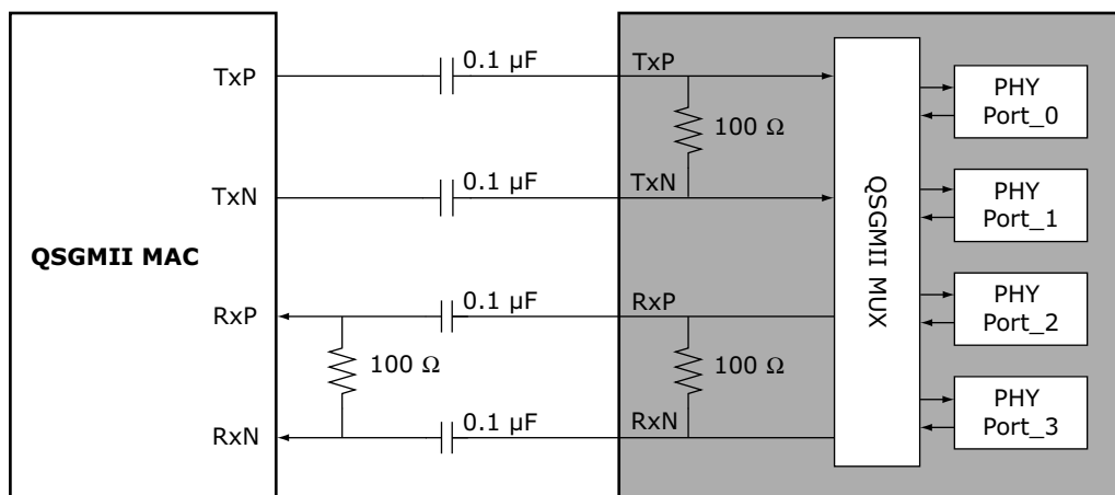
FIGURE 2-12: QSGMII MAC INTERFACE
