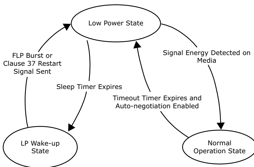
FIGURE 2-21: ACTiPHY STATE DIAGRAM
