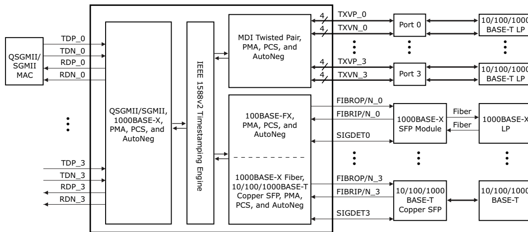
FIGURE 2-6: QSGMII/SGMII MAC-TO-AMS AND PROTOCOL TRANSFER MODE
