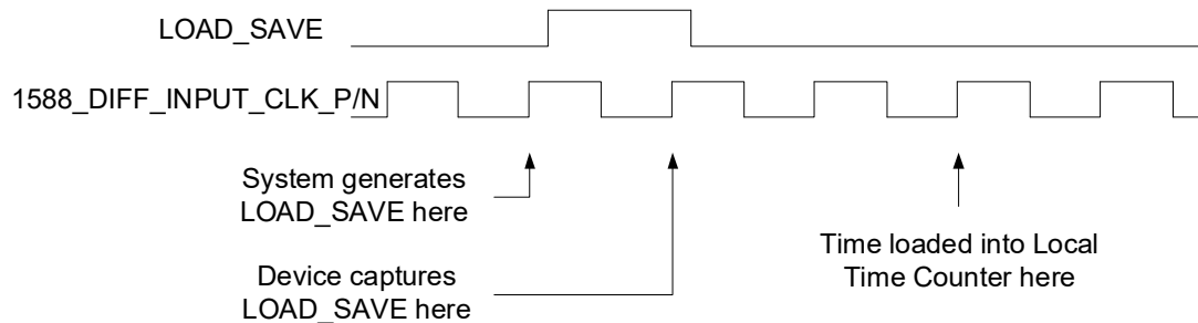
FIGURE 2-61: LOCAL TIME COUNTER LOAD/SAVE TIMING
