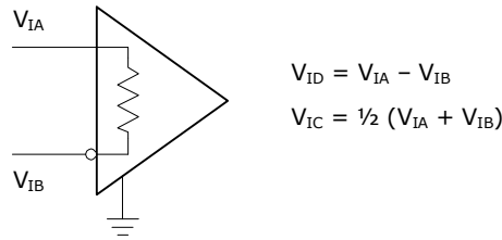
FIGURE 4-4: SGMII DC INPUT DEFINITIONS
