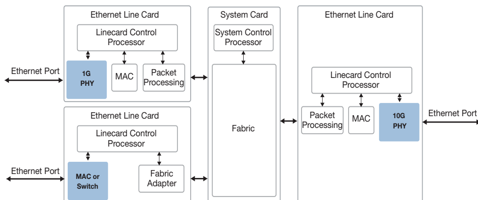
FIGURE 2-25: LINECARD E2E TC PHY APPLICATION
