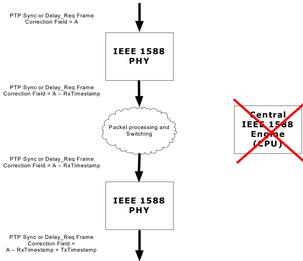
FIGURE 2-23: ONE-STEP E2E TC MODE A
