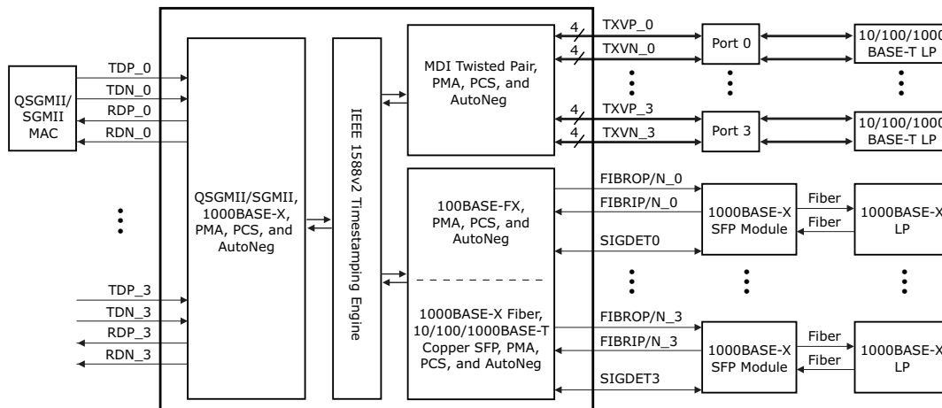
FIGURE 2-4: QSGMII/SGMII MAC-TO-AMS AND 1000BASE-X MEDIA SERDES
