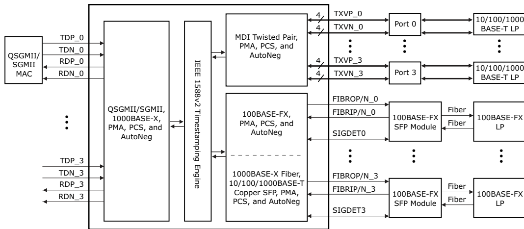
FIGURE 2-5: QSGMII/SGMII MAC-TO-AMS AND 100BASE-FX MEDIA SERDES
