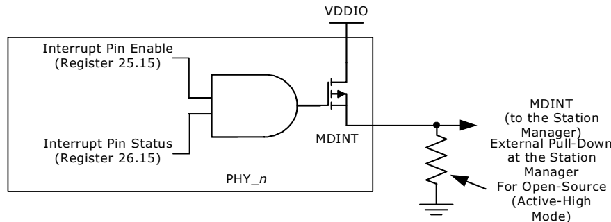
FIGURE 2-65: MDINT CONFIGURED AS AN OPEN-SOURCE (ACTIVE-HIGH) PIN
