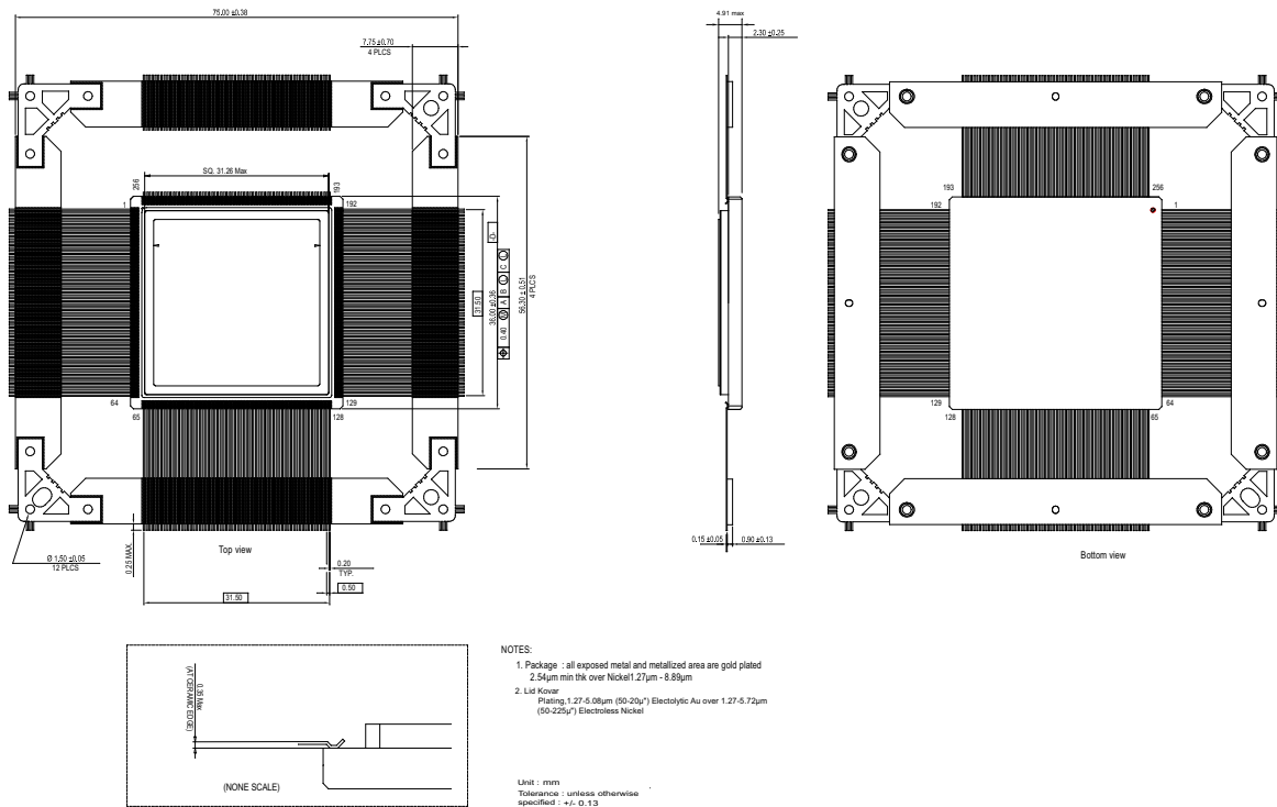
FIGURE 7-2: CQFP256 PACKAGE DRAWING
