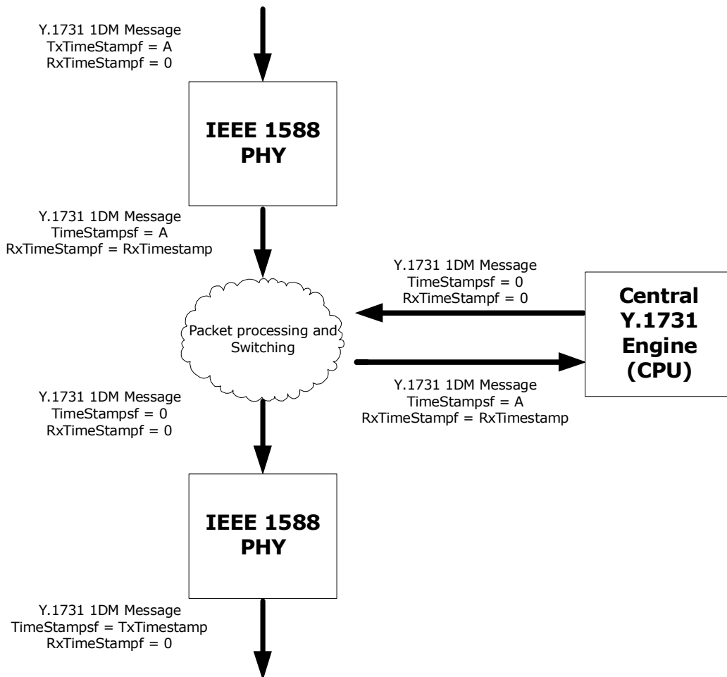
FIGURE 2-33: Y.1731 ONE-WAY DELAY
