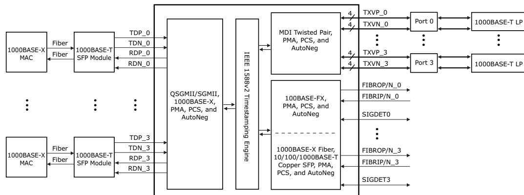
FIGURE 2-9: 1000BASE-X MAC-TO-CAT5 LINK PARTNER
