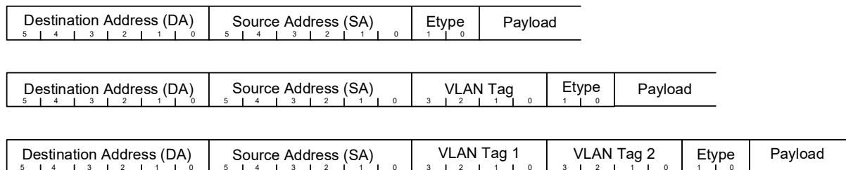
FIGURE 2-40: TYPE II ETHERNET BASIC FRAME FORMAT
