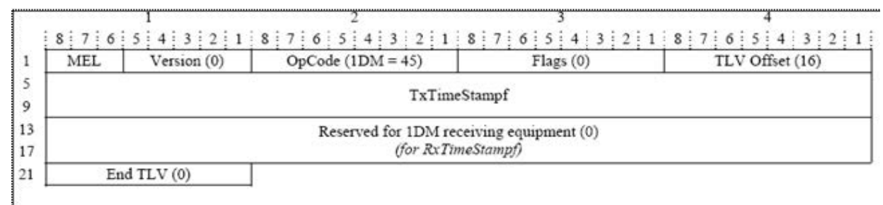
FIGURE 2-32: Y.1731 1DM PDU FORMAT
