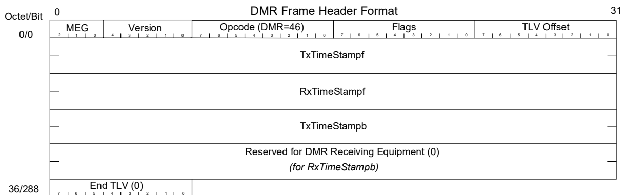
FIGURE 2-58: OAM DMR FRAME HEADER FORMAT
