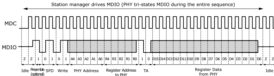
FIGURE 2-63: SMI WRITE FRAME
