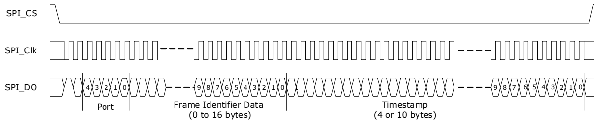
FIGURE 2-59: SERIAL TIME STAMP/FRAME SIGNATURE OUTPUT
