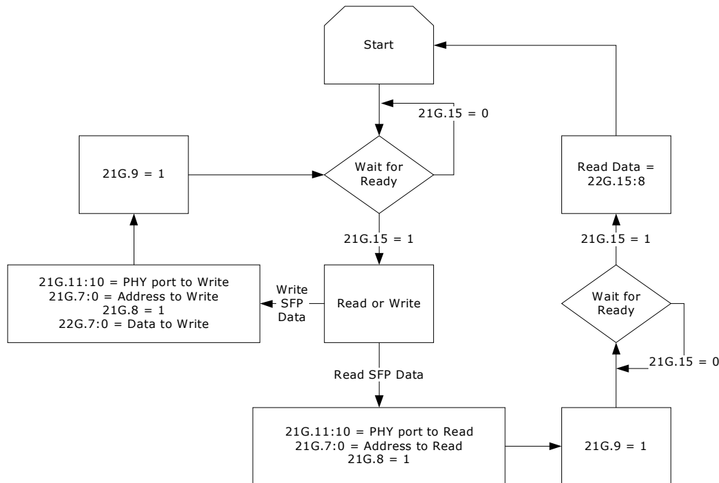
FIGURE 2-67: TWO-WIRE SERIAL MUX READ AND WRITE REGISTER FLOW
