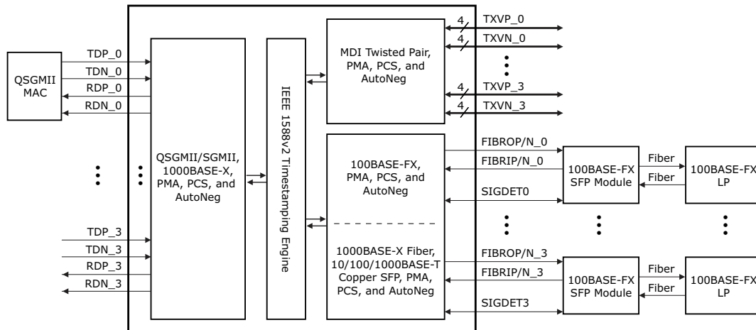
FIGURE 2-3: QSGMII/SGMII MAC-TO-100BASE-FX LINK PARTNER
