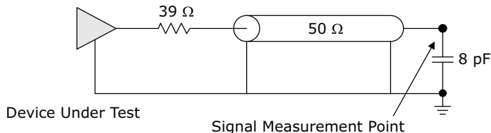
FIGURE 4-5: TEST CIRCUIT FOR RECOVERED CLOCK OUTPUT SIGNALS
