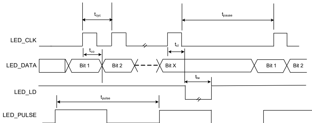
FIGURE 4-8: ENHANCED SERIAL LED TIMING
