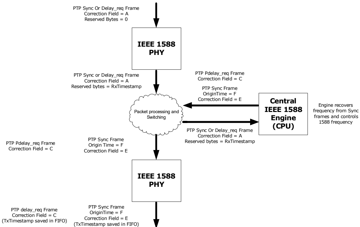
FIGURE 2-30: TWO-STEP E2E BC
