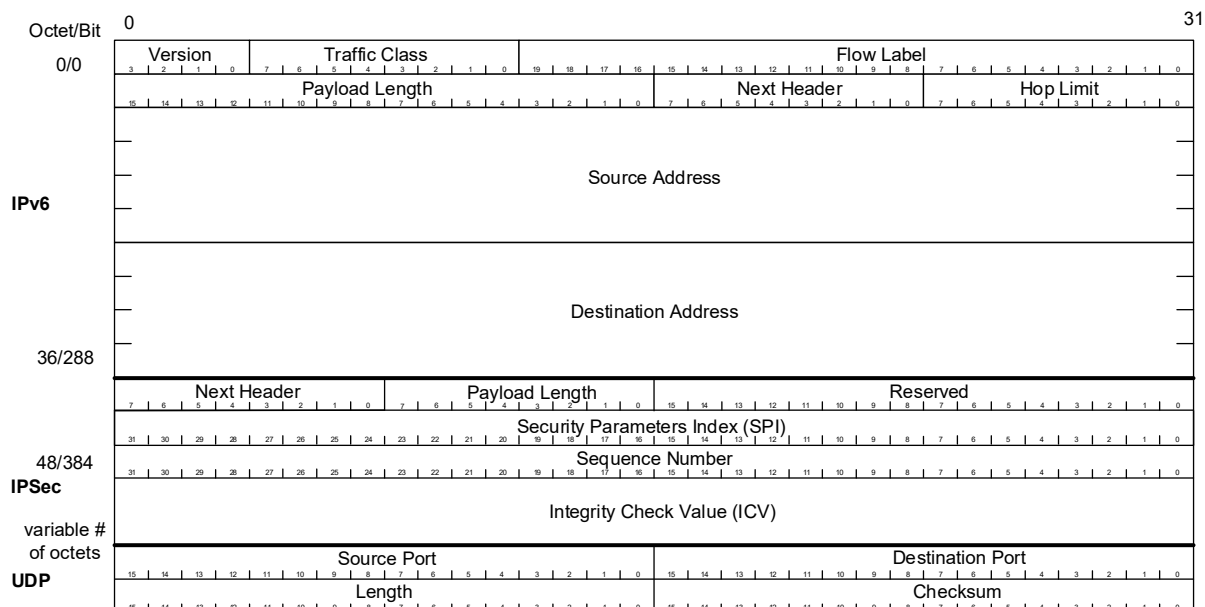
FIGURE 2-54: IPV6 WITH UDP AND IPSEC
