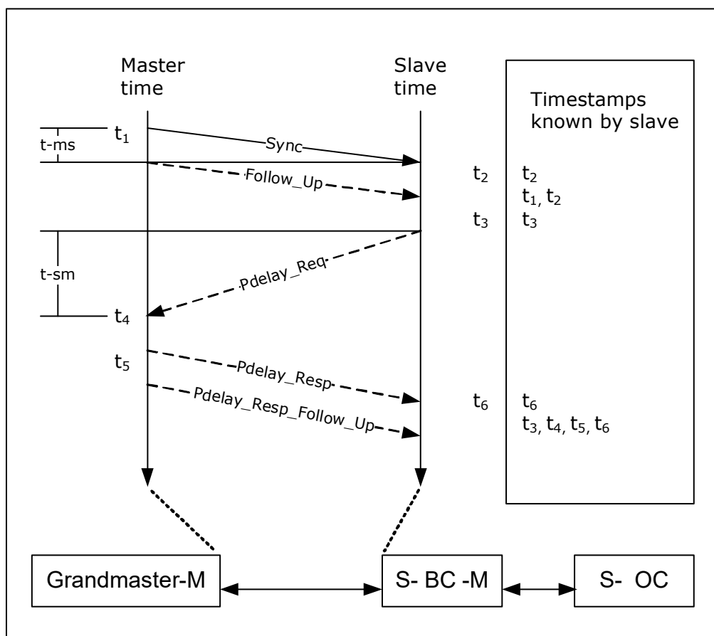
FIGURE 2-27: DELAY MEASUREMENTS
