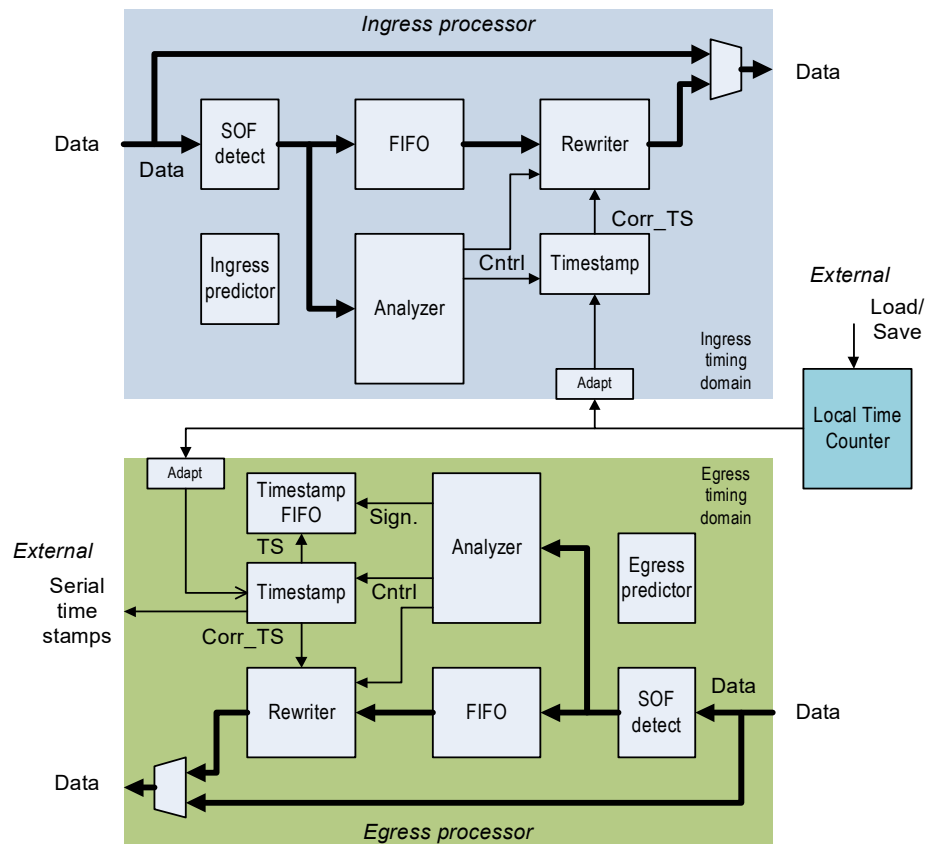
FIGURE 2-38: TSU BLOCK DIAGRAM
