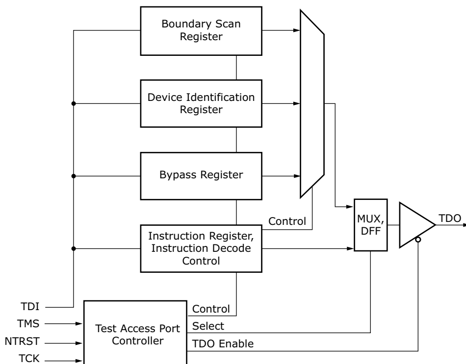
FIGURE 2-72: TEST ACCESS PORT AND BOUNDARY SCAN ARCHITECTURE
