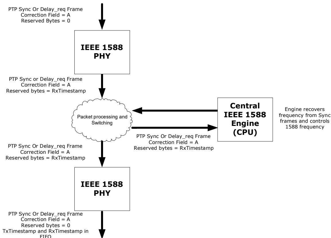
FIGURE 2-31: TWO-STEP E2E TC
