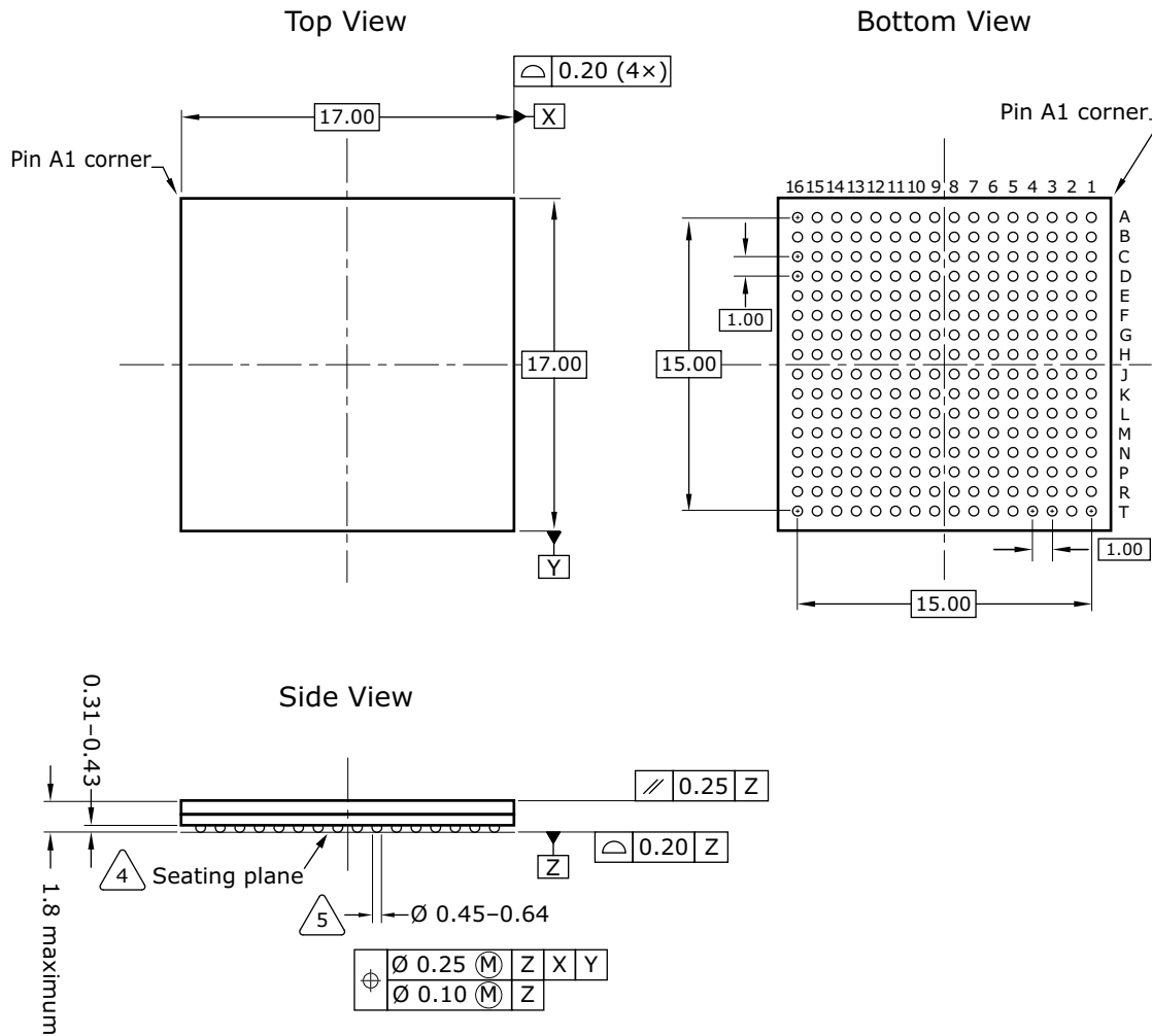
FIGURE 7-1: PBGA256 PACKAGE DRAWING
