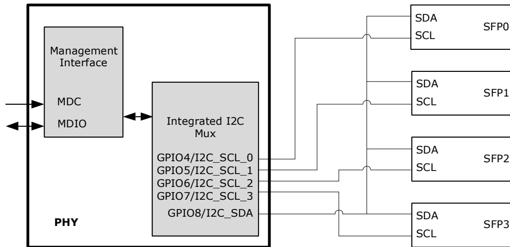
FIGURE 2-66: TWO-WIRE SERIAL MUX WITH SFP CONTROL AND STATUS
