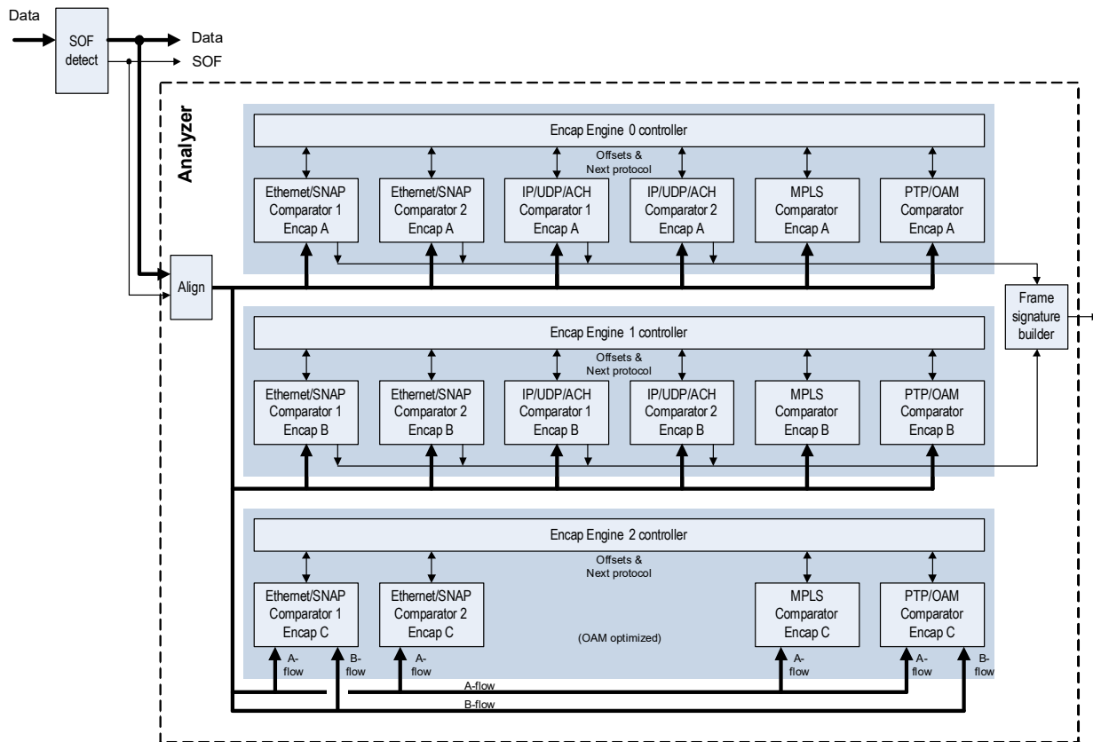
FIGURE 2-39: ANALYZER BLOCK DIAGRAM
