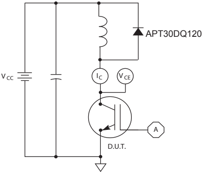
Figure 21, Inductive Switching Test Circuit
