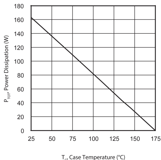
Figure 1-3. Maximum Power Dissipation vs. Case Temp.
