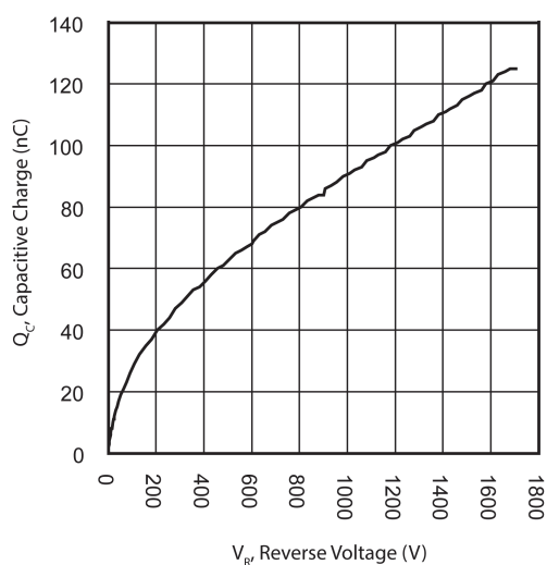
Figure 1-5. Total Charge vs. Reverse Voltage
