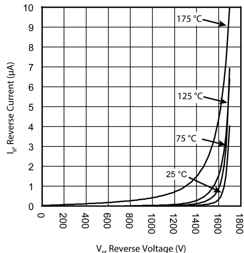
Figure 1-4. Reverse Current vs. Reverse Voltage
