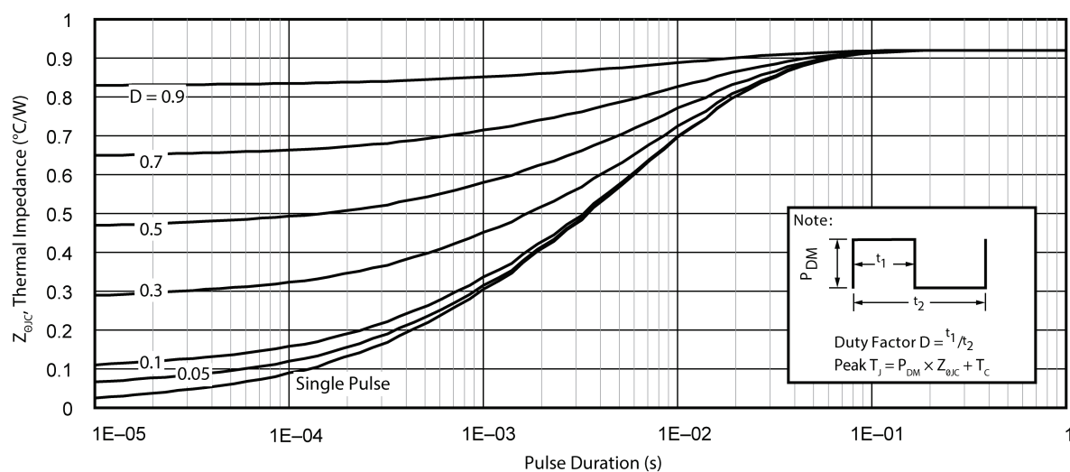
Figure 1-7. Maximum Transient Thermal Impedance
