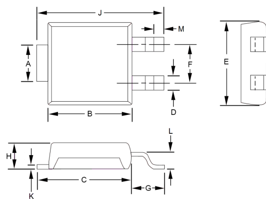
Figure 3-1. Package Dimensions
