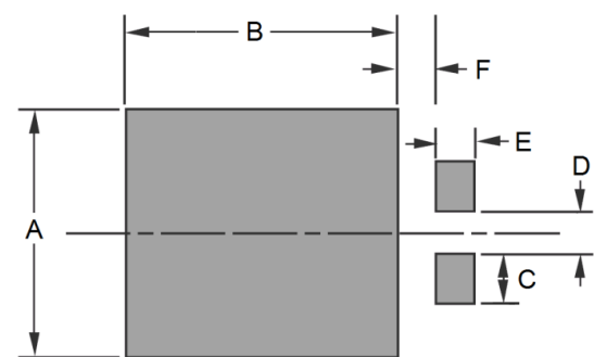
Figure 3-2. Pad Layout
