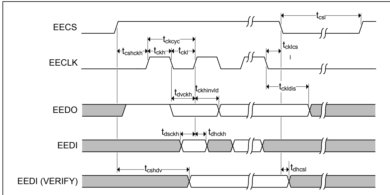
FIGURE 5-6: EEPROM TIMING
