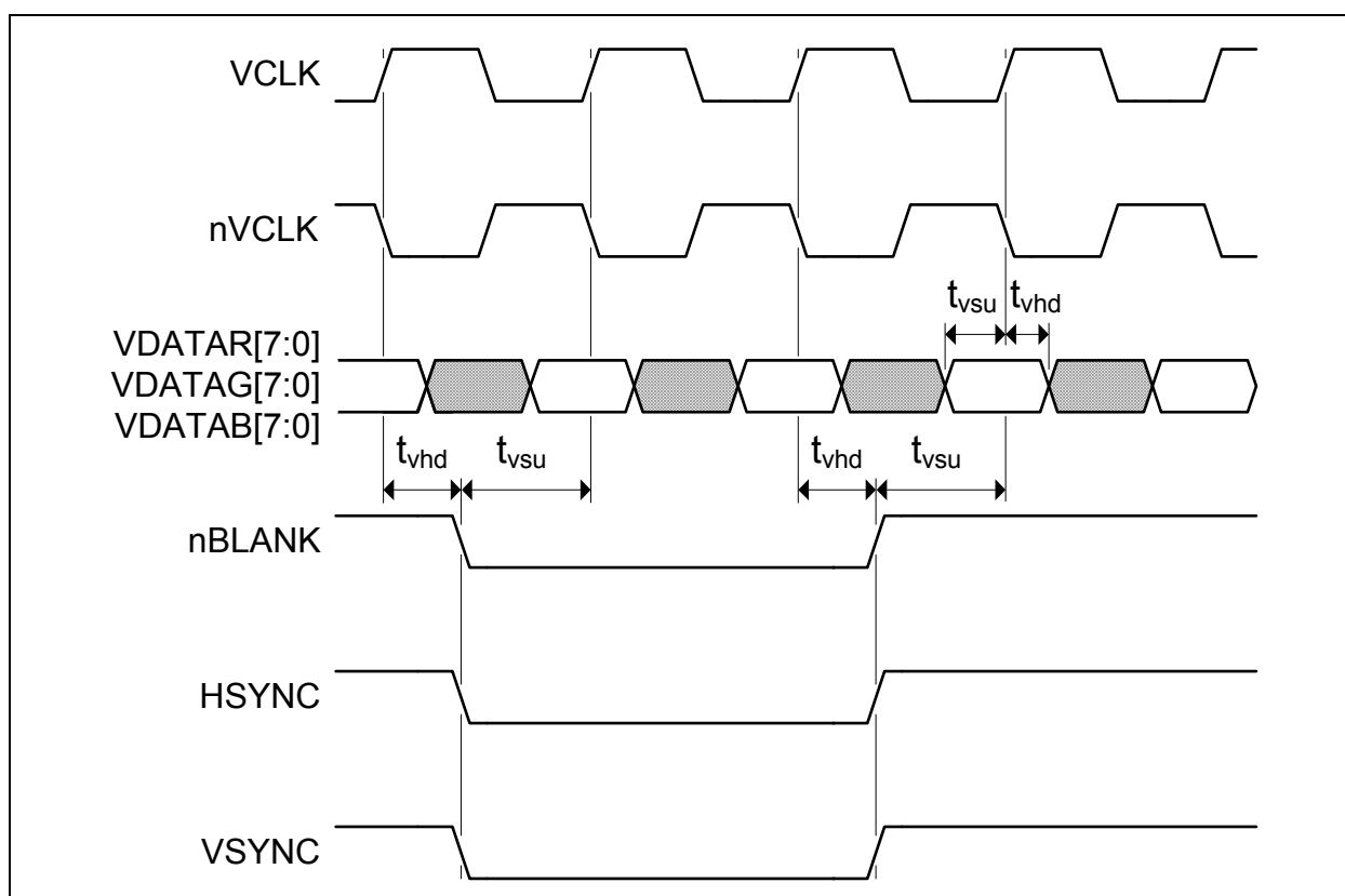
FIGURE 5-5: DIGITAL RGB TIMING - SDR MODE
