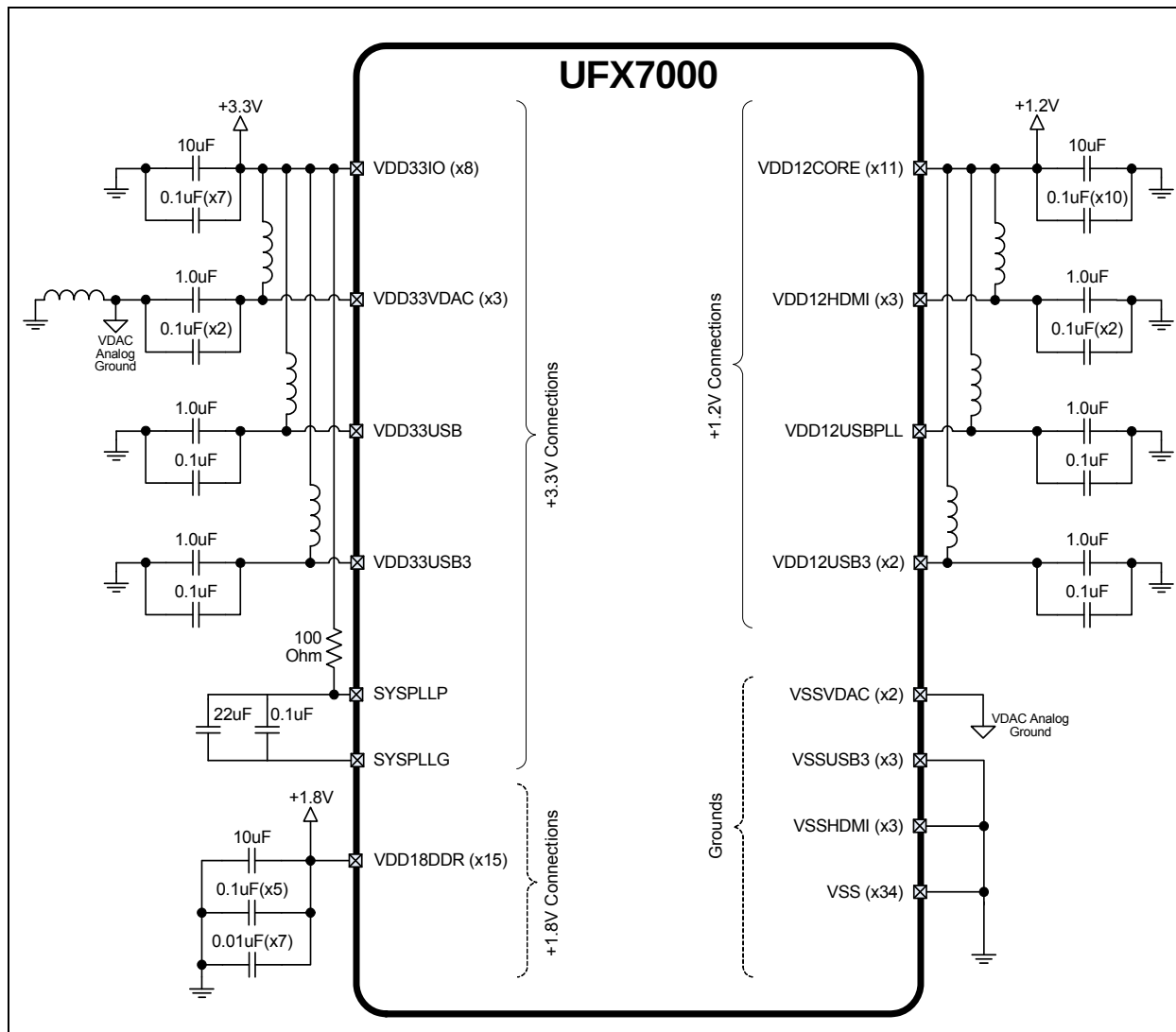
FIGURE 3-1: POWER CONNECTIONS
