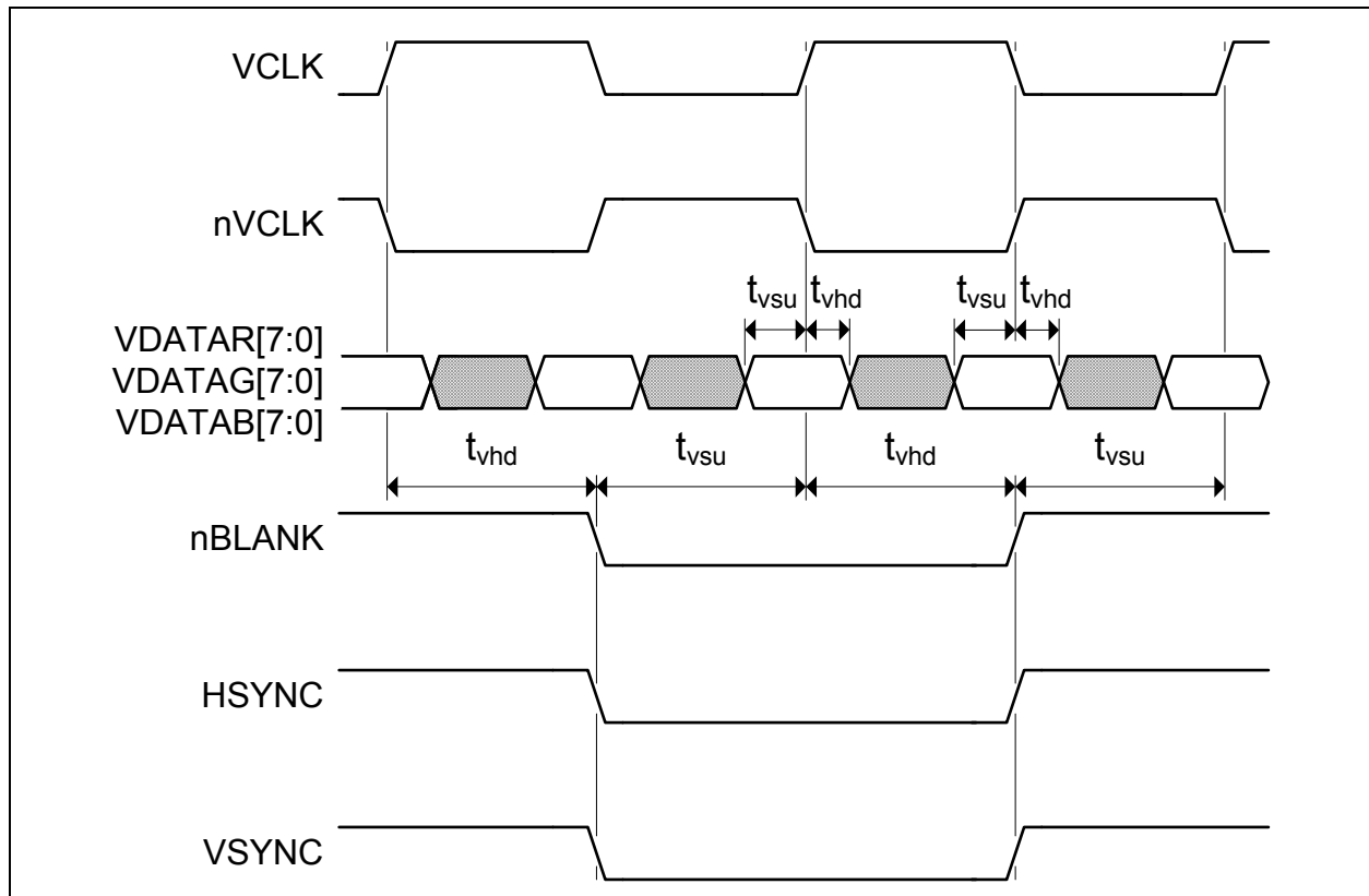
FIGURE 5-4: DIGITAL RGB TIMING - DDR MODE
