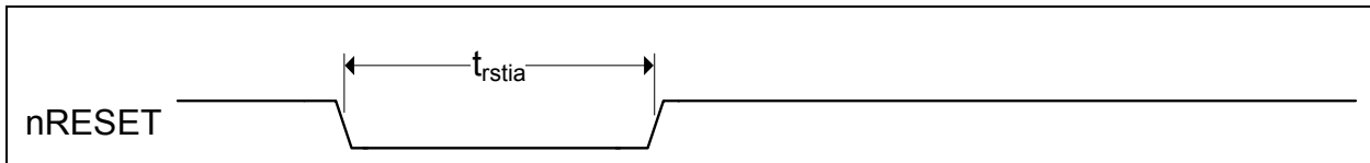
FIGURE 5-3: NRESET TIMING
