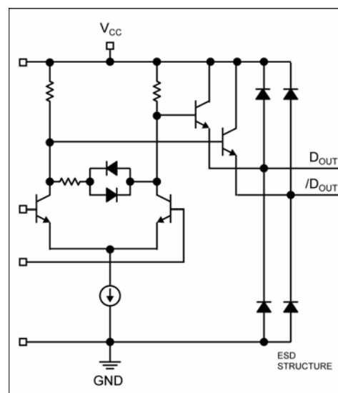
Figure 3. Output Structure
