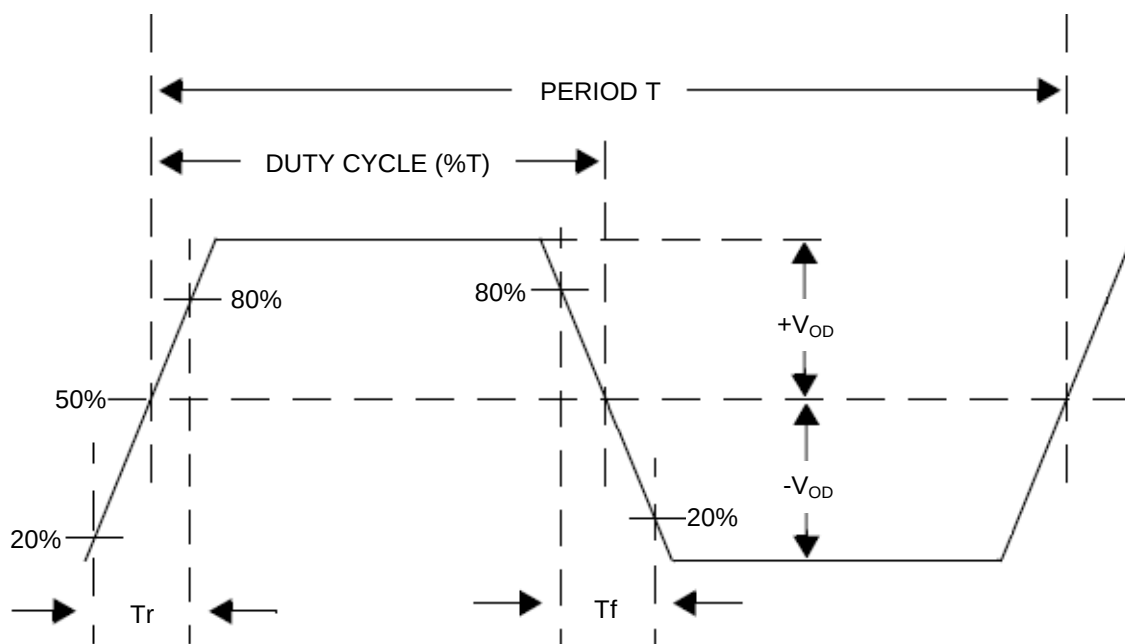
Figure 6-3. Differential Output Waveform
