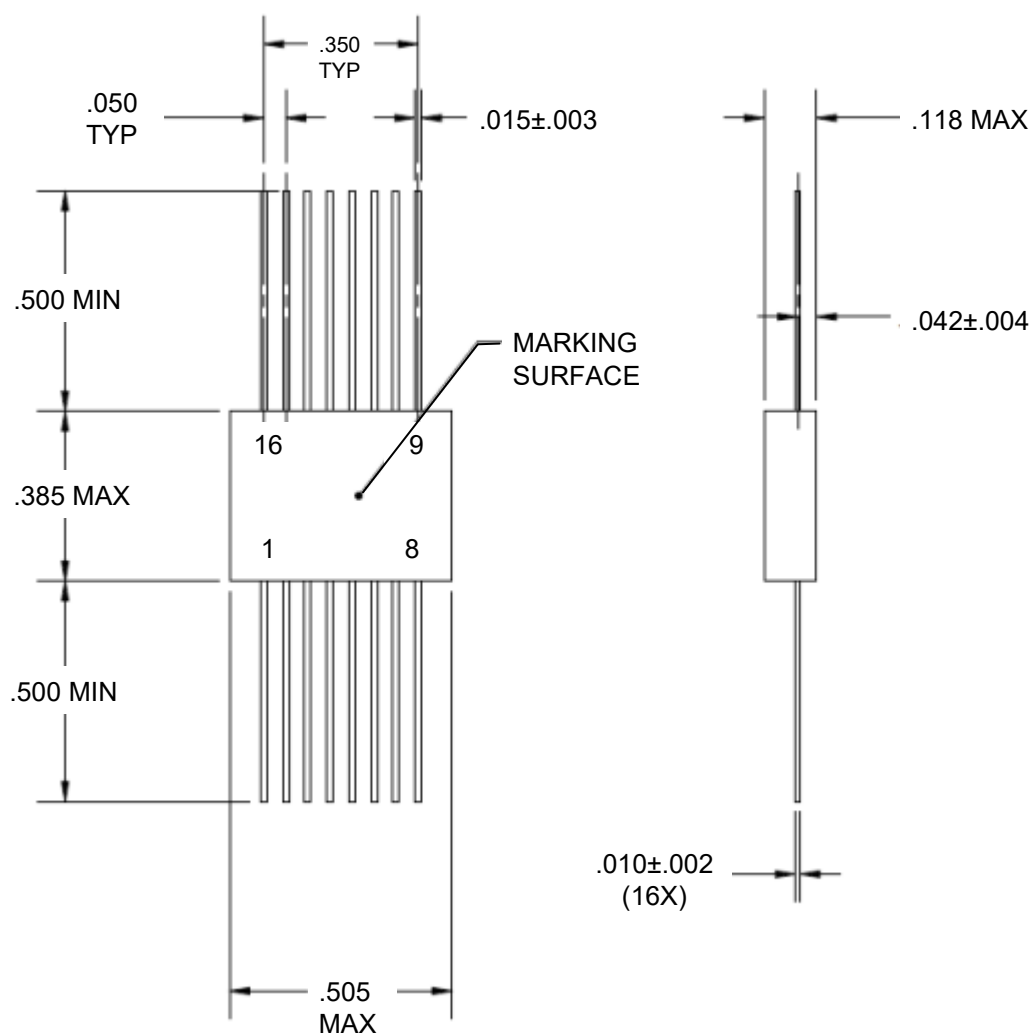
Figure 6-5. Model 1603/1606 Package Outline and I/O Connections
