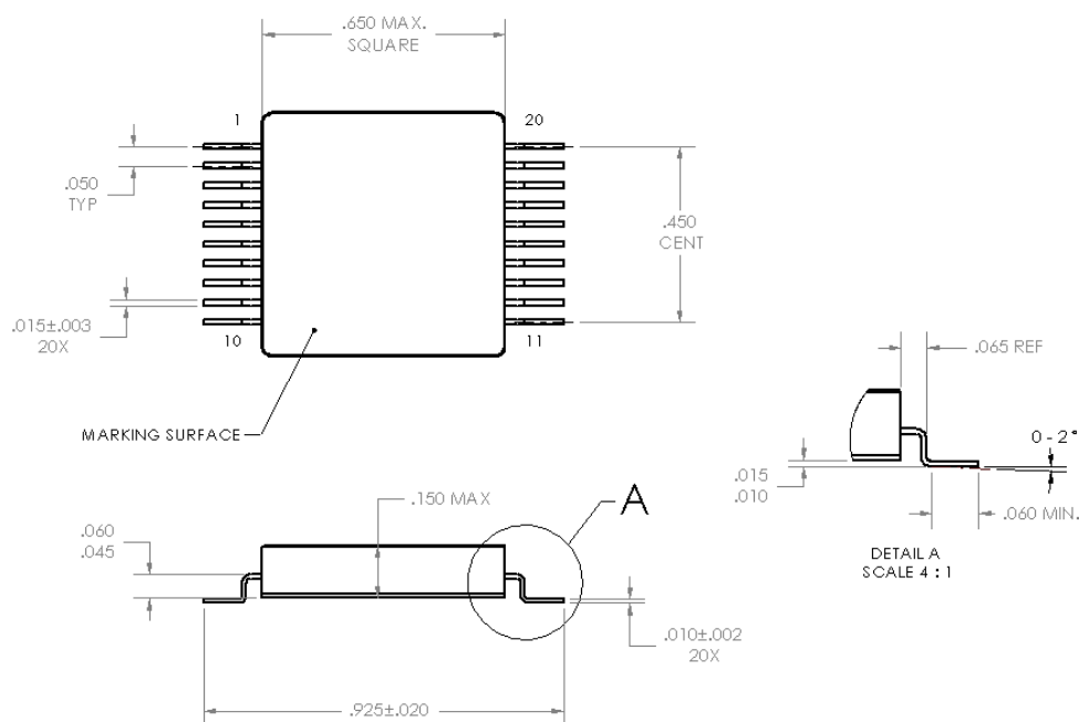
Figure 6-8. Model 1620/1640/1680 Package Outline and I/O Connections
