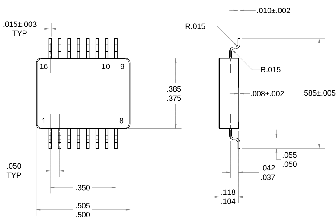
Figure 6-7. Model 1619/1638 Package Outline and I/O Connections
