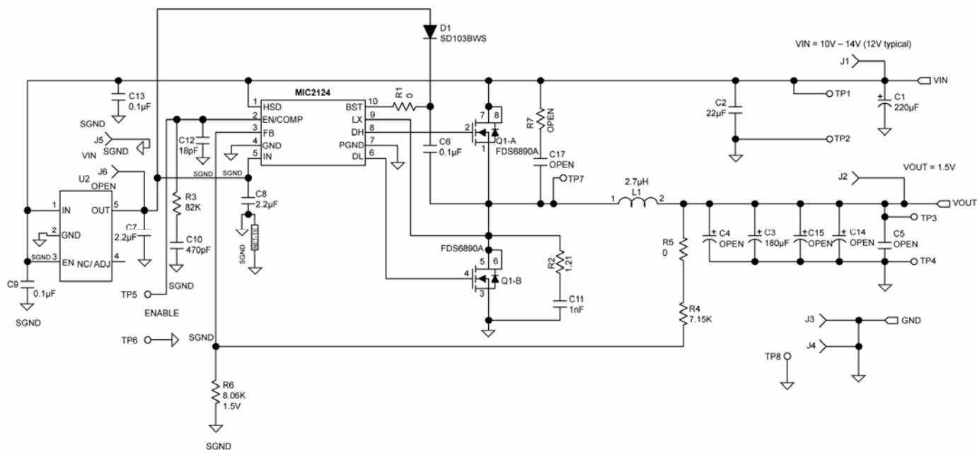
Figure 10. Schematic of MIC2124 5A Evaluation Board
