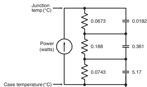
FIGURE 24b. TRANSIENT THERMAL IMPEDANCE MODEL
