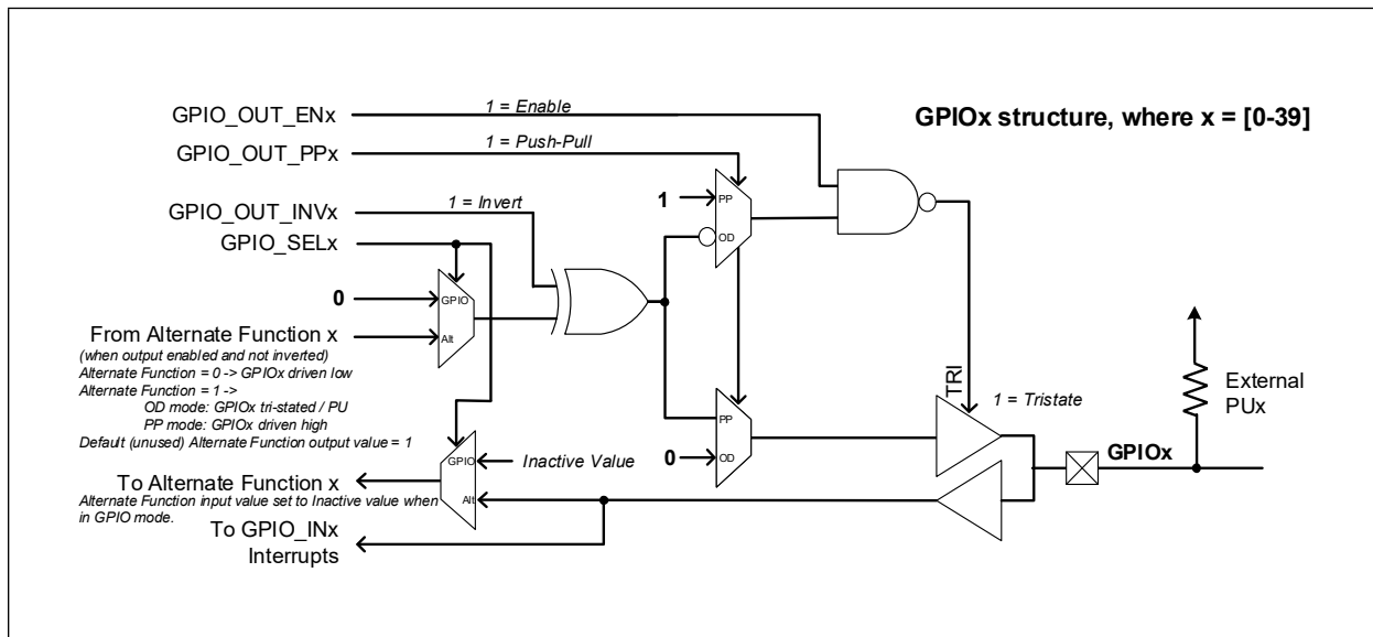
FIGURE 3-34: GPIO STRUCTURE
