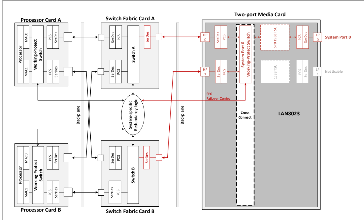
FIGURE 3-7: 1:1 OR 1+1 HOST PROTECTION
