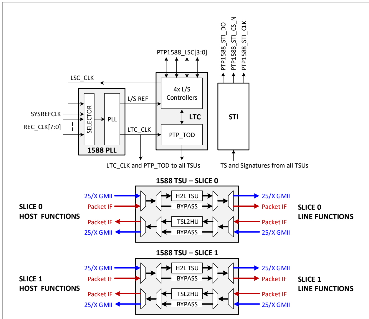
FIGURE 3-13: 1588 BLOCK DIAGRAM
