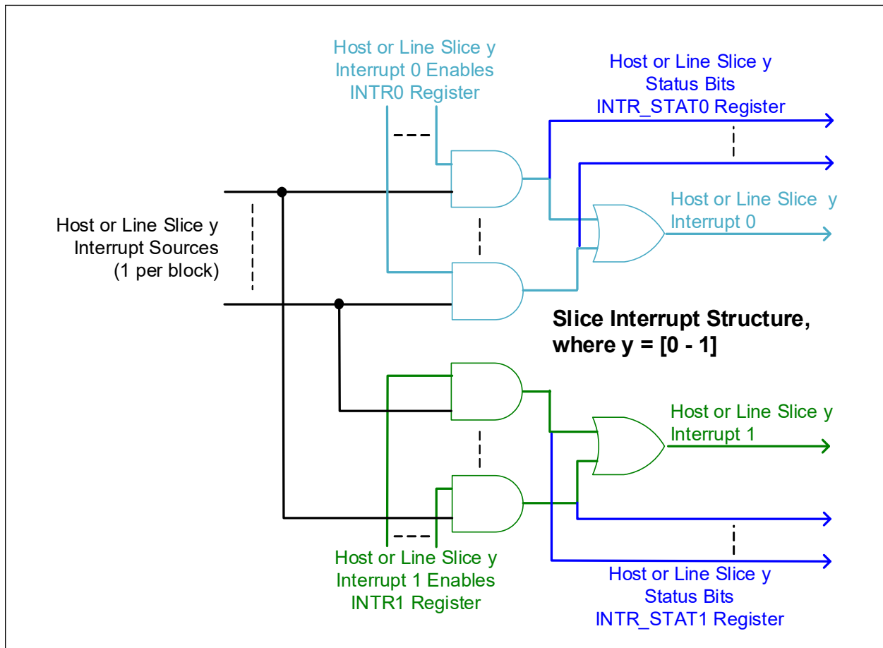
FIGURE 3-36: SLICE INTERRUPTS
