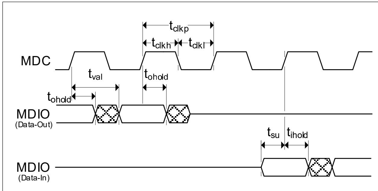
FIGURE 4-2: MDC/MDIO TIMING
