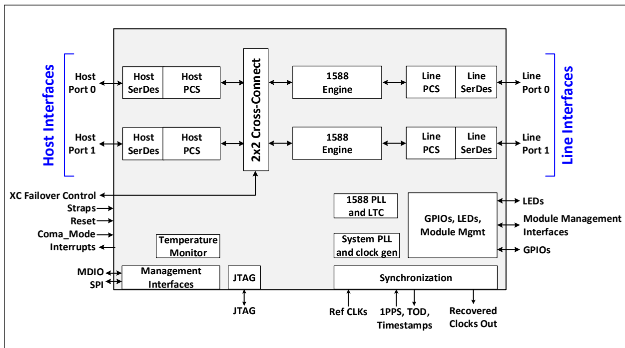
FIGURE 1-1: LAN8023 INTERNAL BLOCK DIAGRAM
