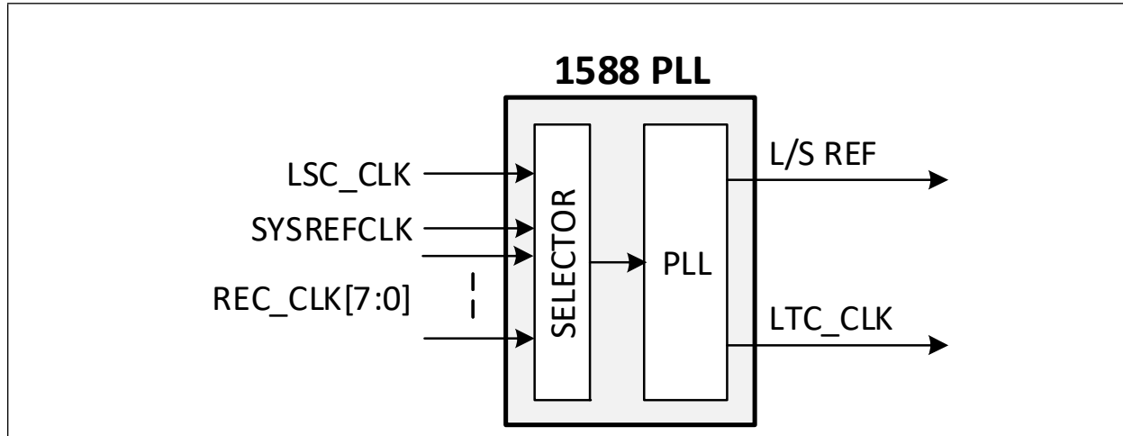
FIGURE 3-14: 1588 PLL
