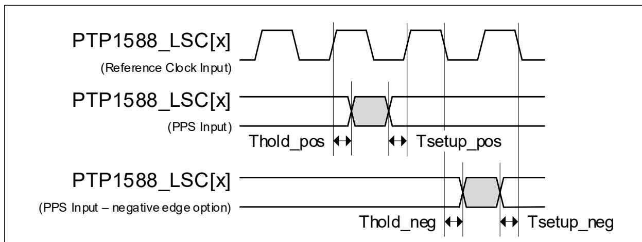
FIGURE 4-6: PTP EXTERNAL (2-PIN) SYNCHRONOUS PPS, PPS W/TOD INPUT TIMING
