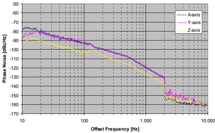
VX-990 without shock absorber vibration spectrum DO-160 curve C
