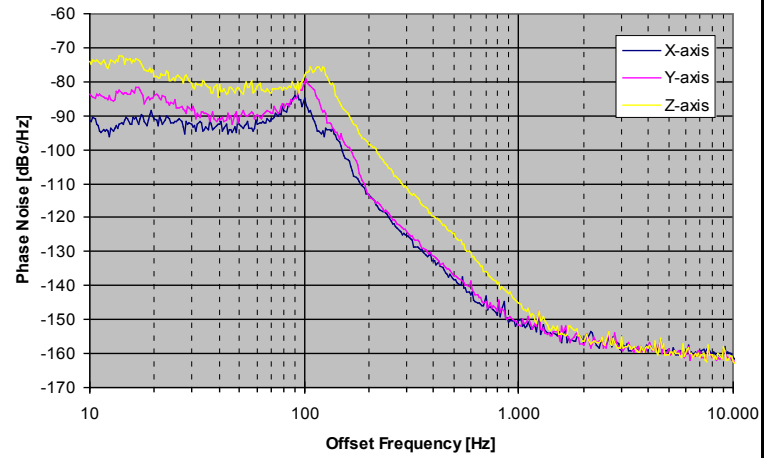
Typical Phase Noise: VX-990 vibration spectrum DO-160 curve C
