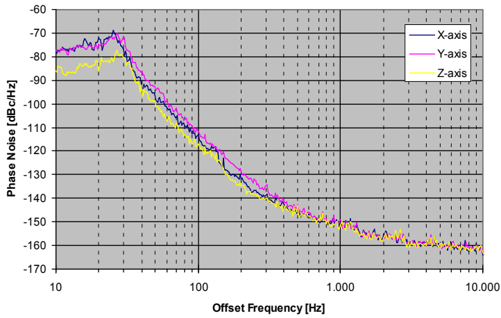
Typical Phase noise: VX-990 vibration spectrum DO-160 curve C
