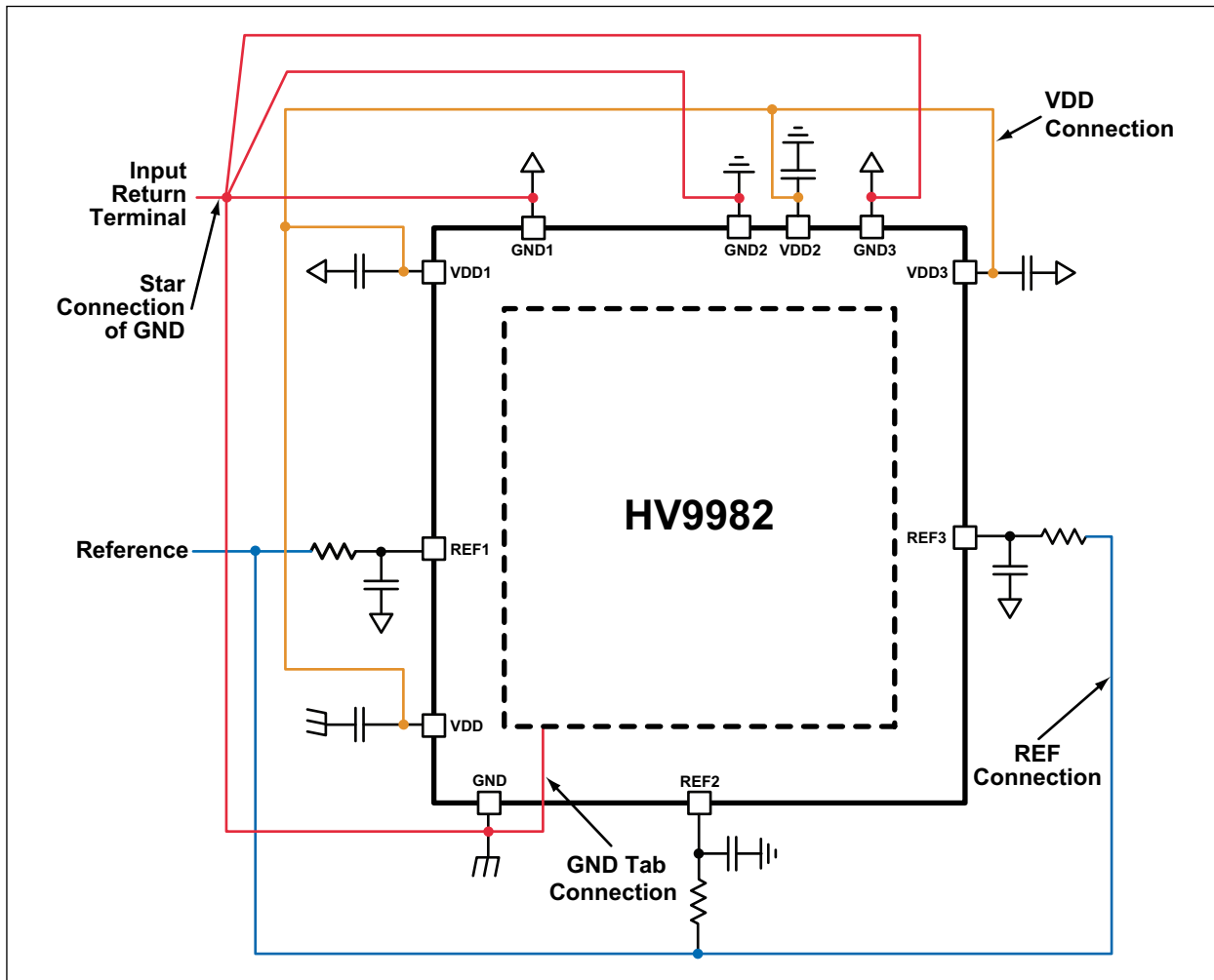
FIGURE 3-2: LAYOUT GUIDELINES
