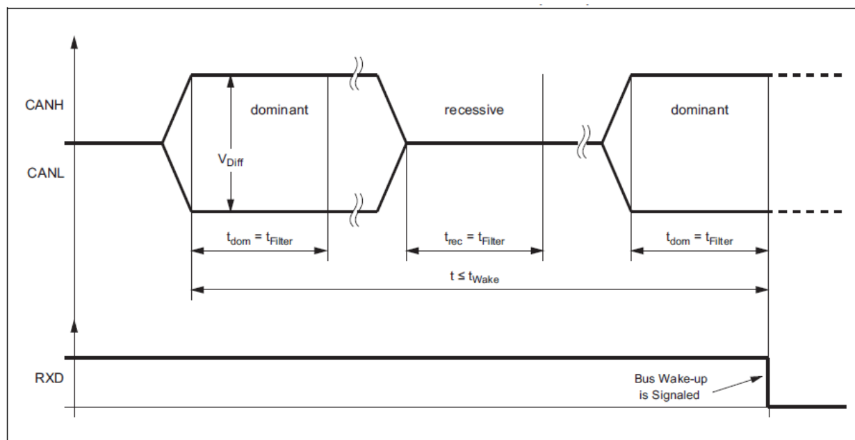
Figure 4-2. Timing of the Bus WUP in Standby Mode
