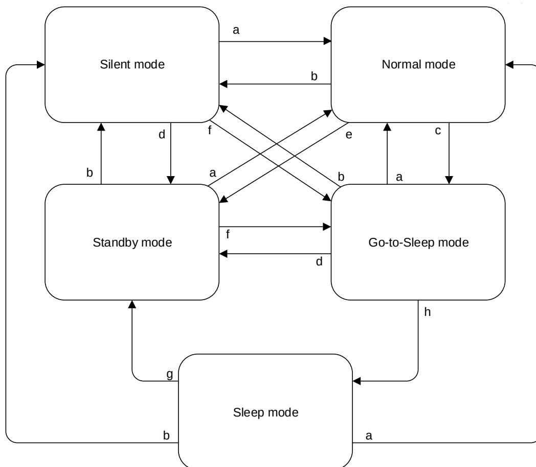
Figure 4-1. Operating Modes
