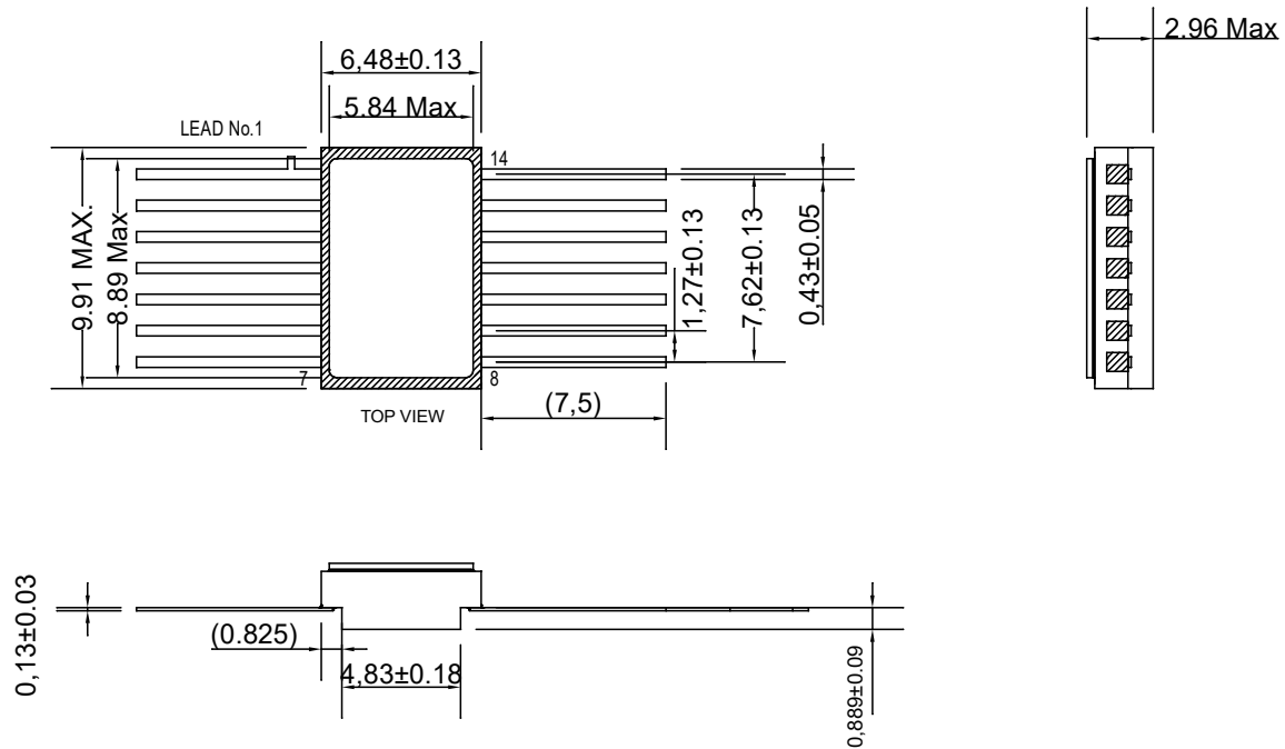
Figure 9-5. 14 -Lead Ceramic Dual Flat Pack (XGB) 6.48 × 9.91 mm with Flat Leads [CDFP]
