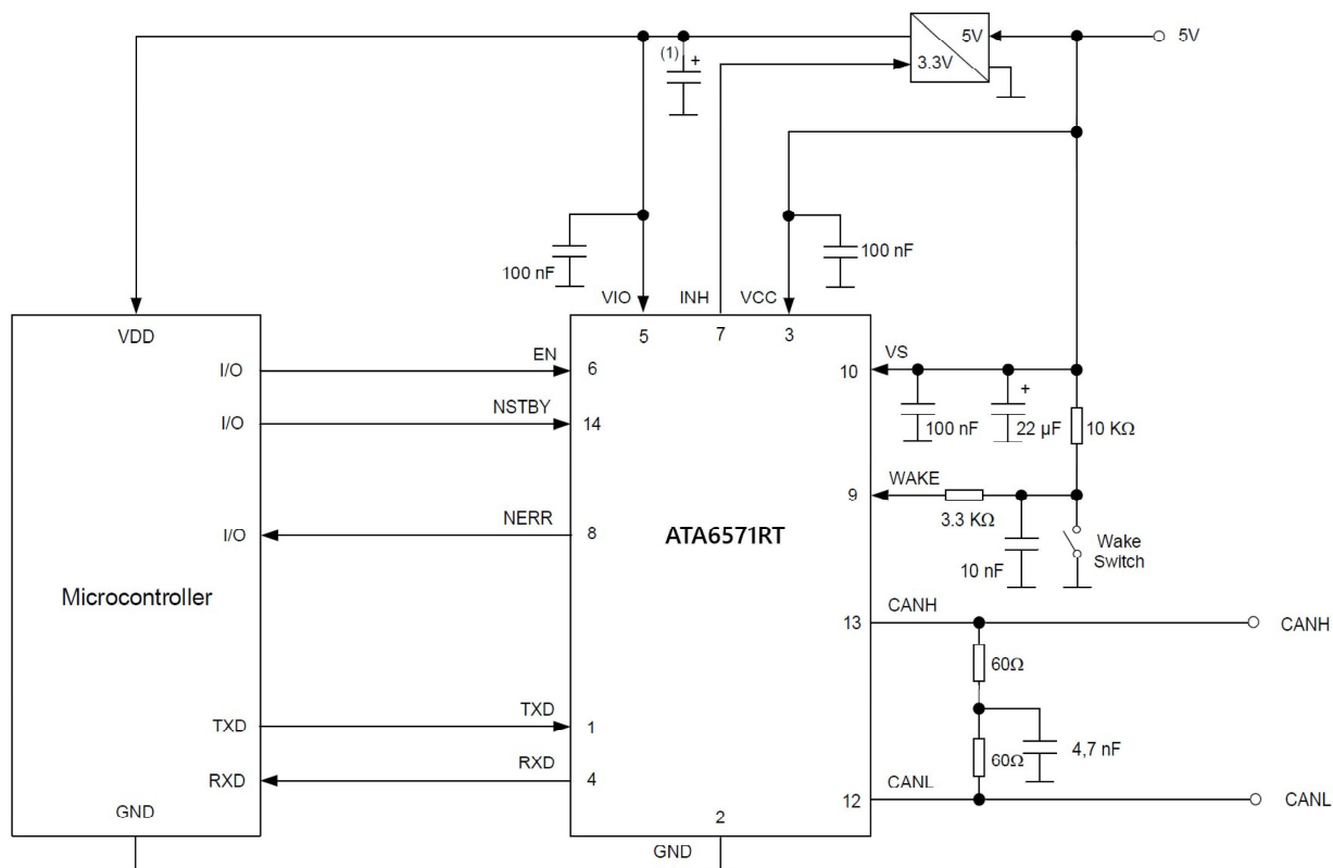
Figure 8-1. Typical Application Circuit
