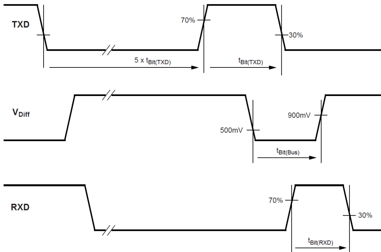
Figure 7-2. CAN Transceiver Timing Diagram 2
