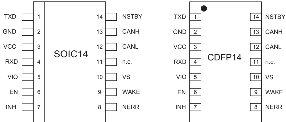
Figure 3-1. Pin Configuration
