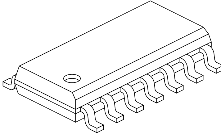
Figure 9-3. 14-Lead Plastic Small Outline (SL)—Narrow, 3.90 mm Body [SOIC]
