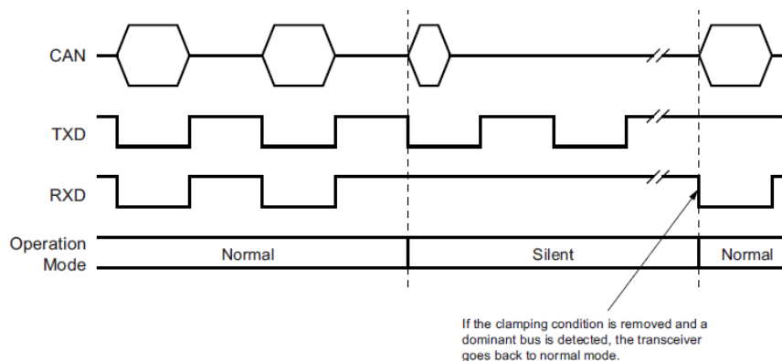
Figure 4-3. RXD Recessive Clamping Detection
