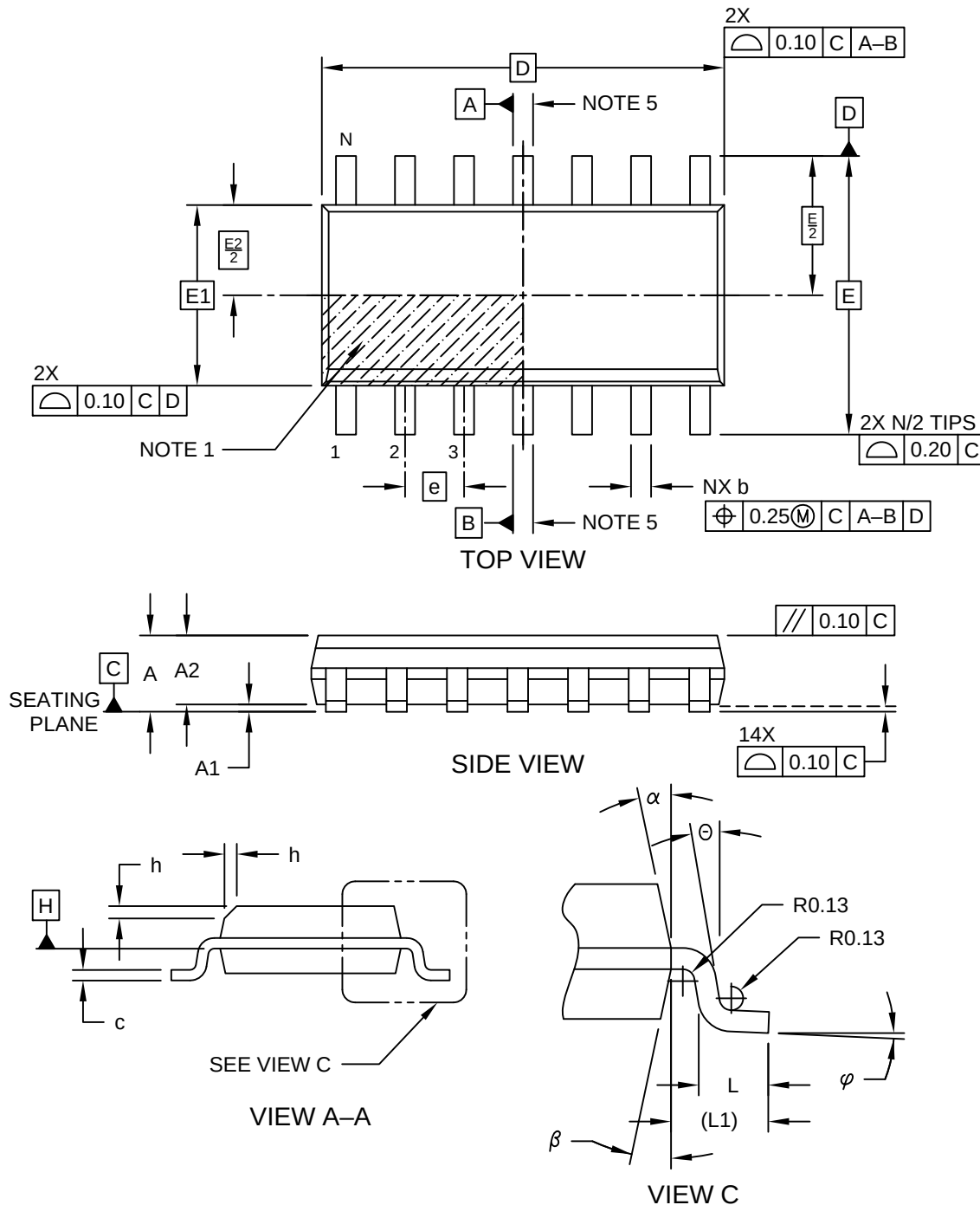
Figure 9-2. 14-Lead Plastic Small Outline (SL) - Narrow, 3.90 mm Body [SOIC]
