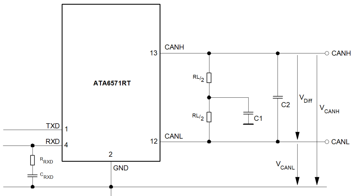
Figure 8-2. Test Circuit
