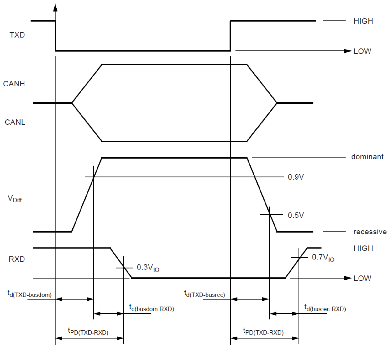
Figure 7-1. CAN Transceiver Timing Diagram 1
