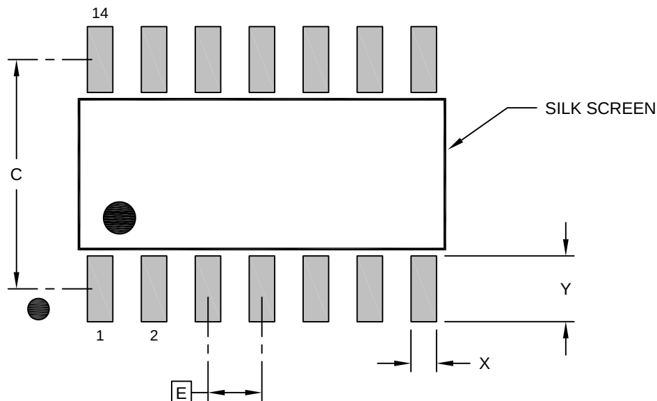
Figure 9-4. 14-Lead Plastic Small Outline (SL)—Narrow, 3.90 mm Body [SOIC]
