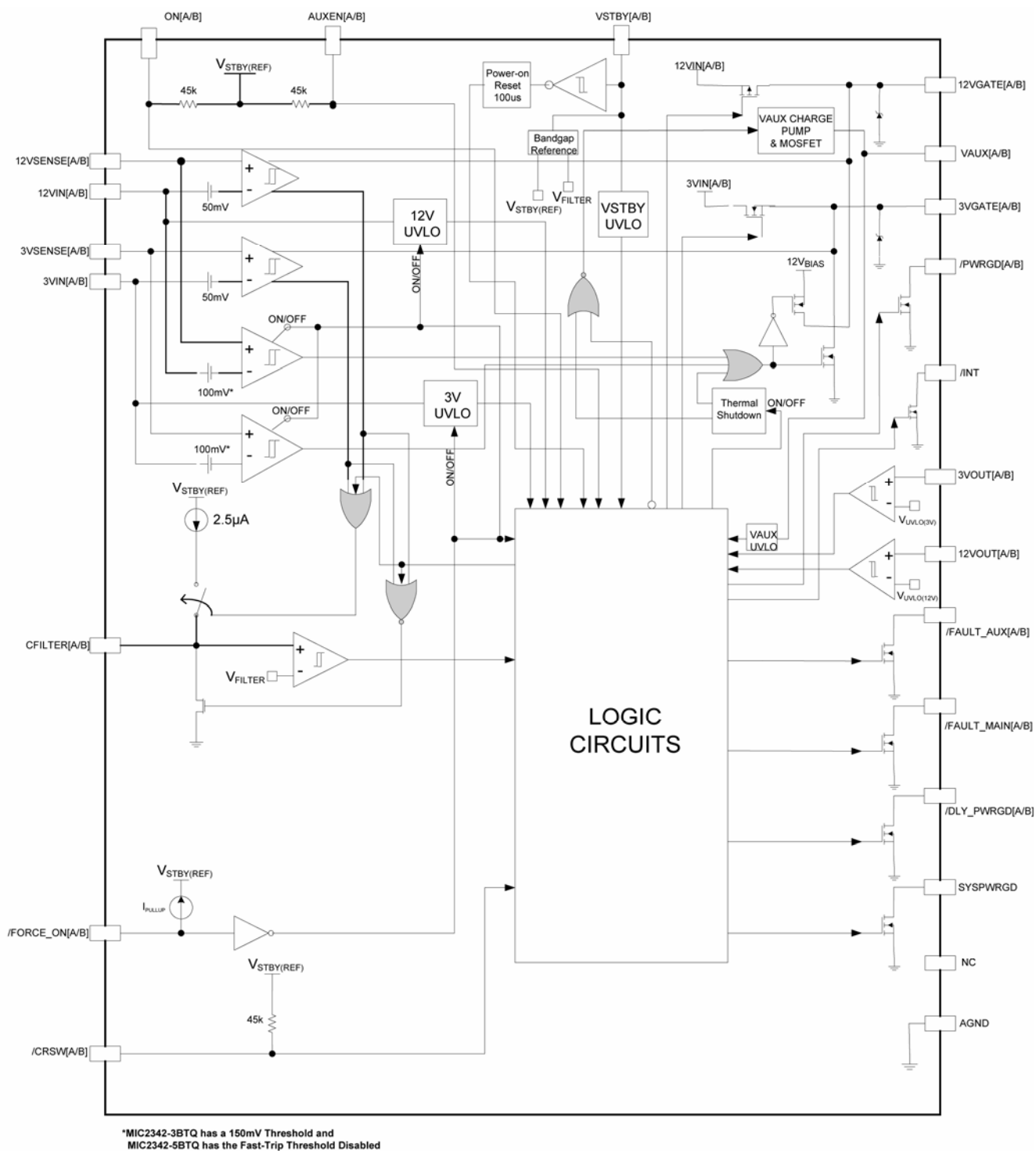
MIC2342/MIC2342R Block Diagram
