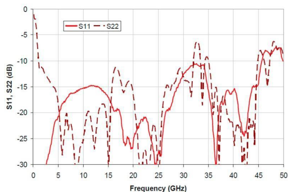
UA0U50HM S11, S22
