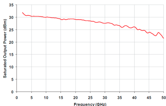
UA0U50HM Saturated Output Power
