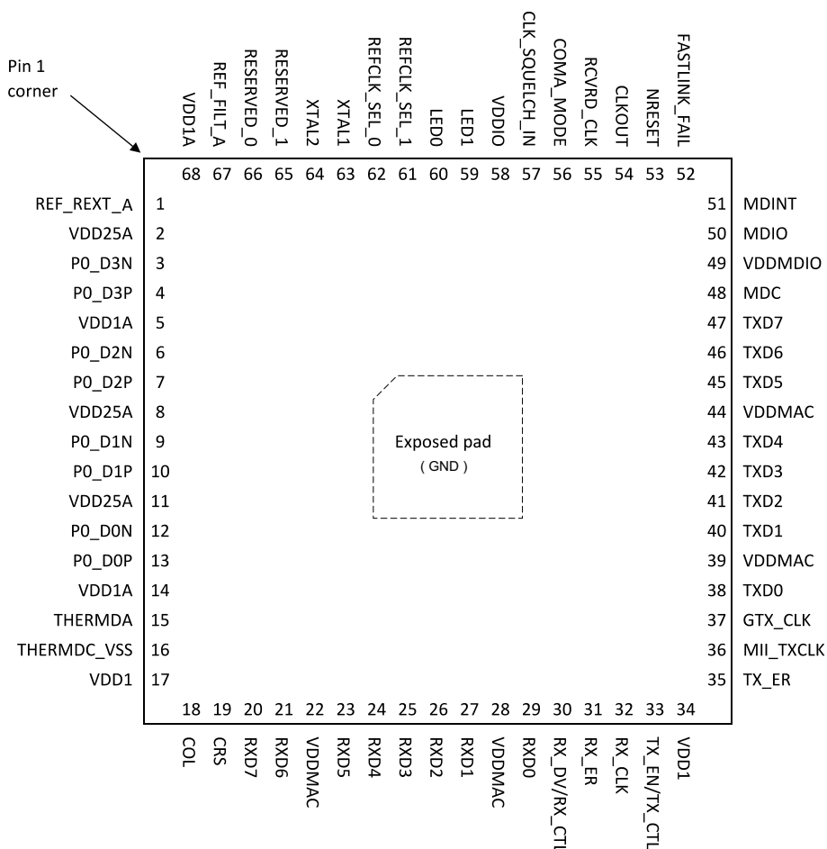
FIGURE 3-1: PIN DIAGRAM
