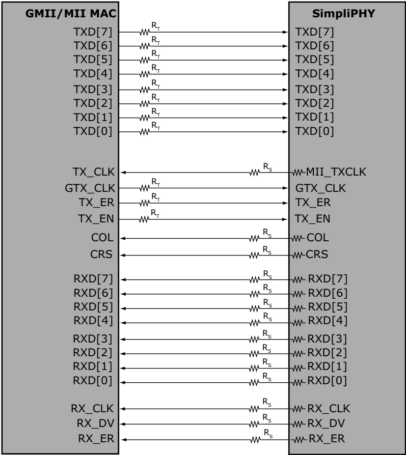
FIGURE 5-2: GMII/MII MAC INTERFACE
