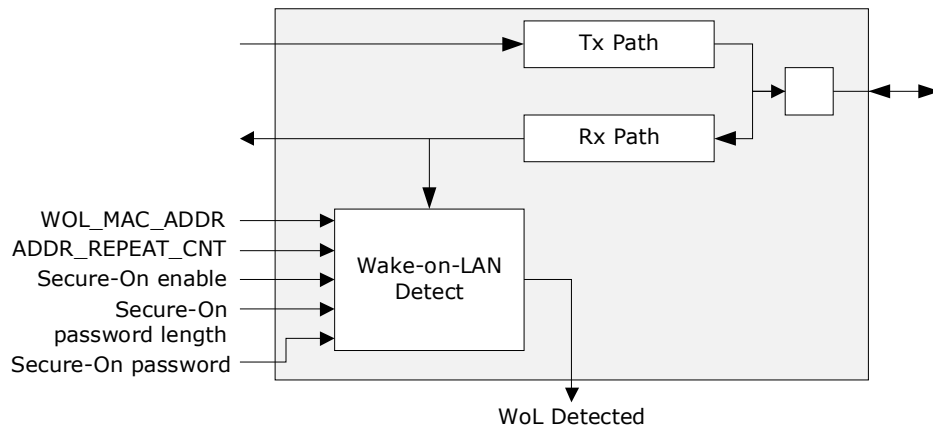
FIGURE 5-16: WAKE-ON-LAN FUNCTIONALITY
