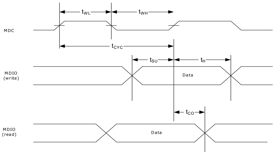
FIGURE 8-12: SERIAL MANAGEMENT INTERFACE TIMING
