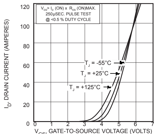
FIGURE 3, TRANSFER CHARACTERISTICS
