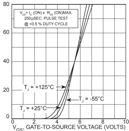
FIGURE 4, TRANSFER CHARACTERISTICS
