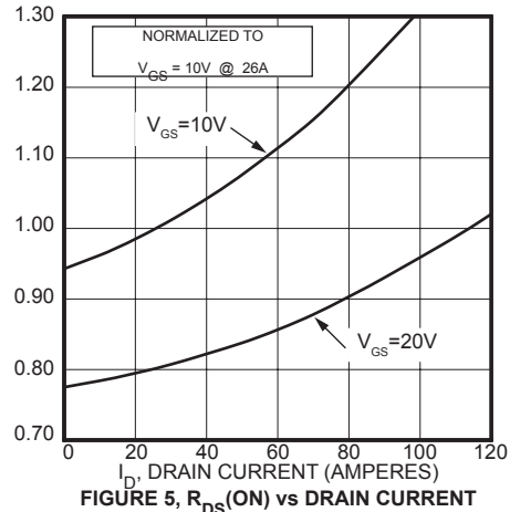
FIGURE 5, R_{DS(ON)} vs DRAIN CURRENT
