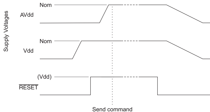
Figure 4-2. Power Sequencing on the mXT768E-AB – Late rise on AVDD
