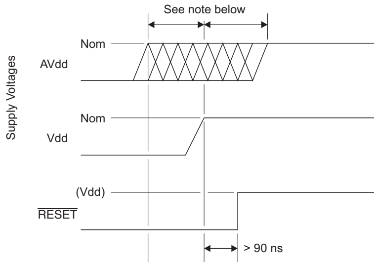
Figure 4-1. Power Sequencing on the mXT768E-AB
