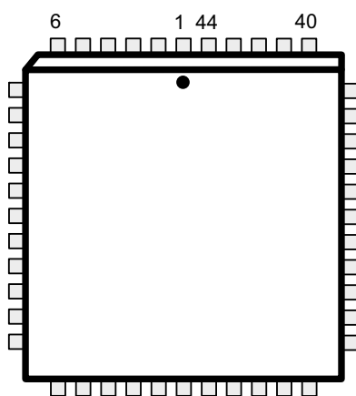
44-Lead PLCC
