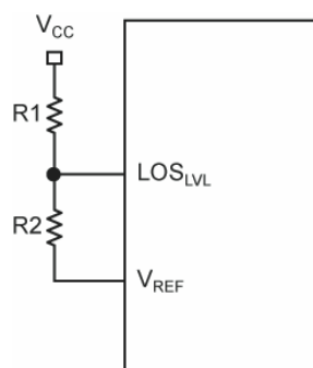
Figure 5. LOSL_{LVL} Circuit
