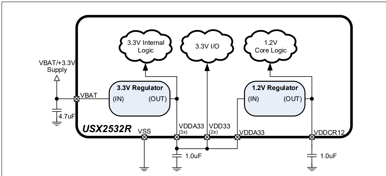
FIGURE 4-1: POWER CONNECTIONS
