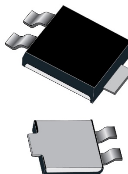
Figure 1. Powermite 3® Package
