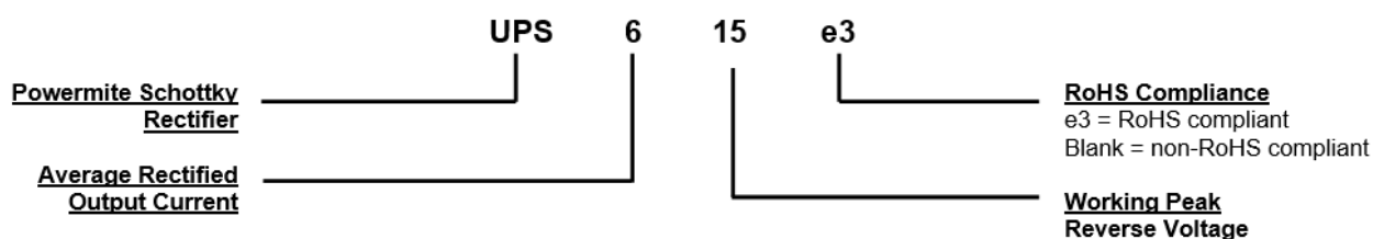
Figure 1-1. Part Nomenclature
