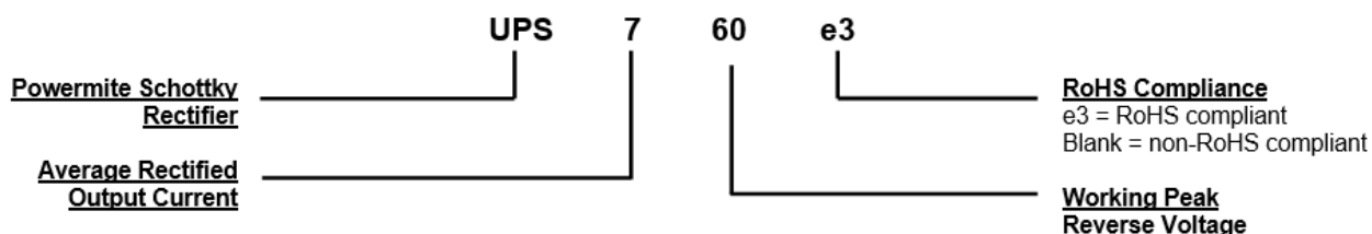
Figure 1-1. Part Nomenclature
