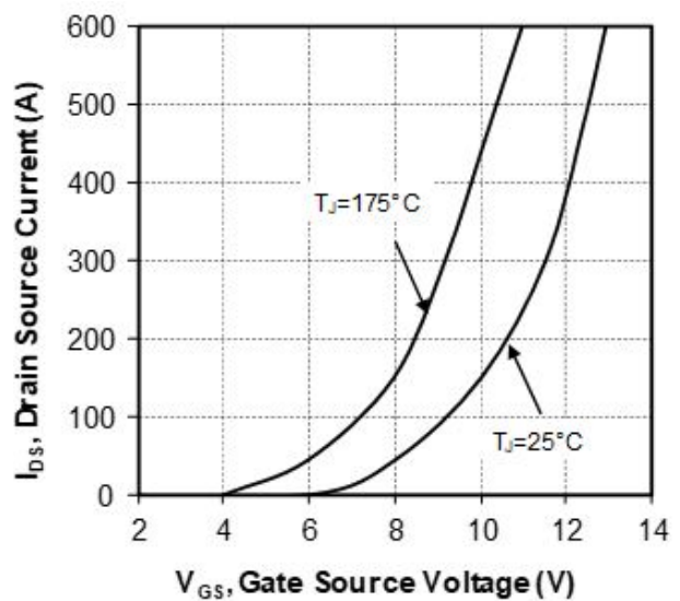
Figure 1-5. Transfer Characteristics
