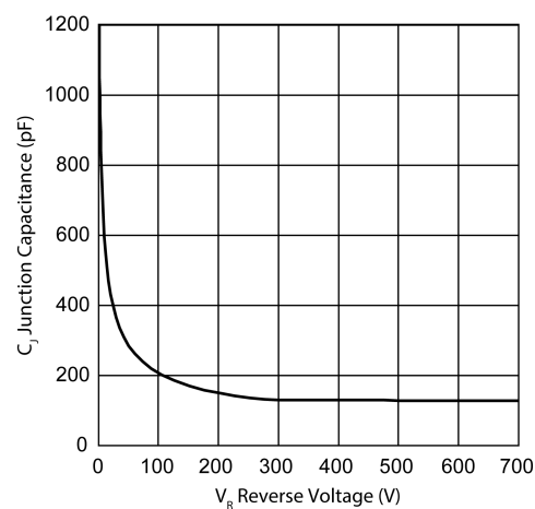
Figure 7 • Junction Capacitance vs. V_R
