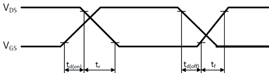
Figure 1-18. Switching Waveform
