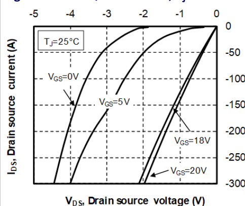
Figure 11 • 3 rd Quadrant Char, T_J = 25^\circ\text{C}
