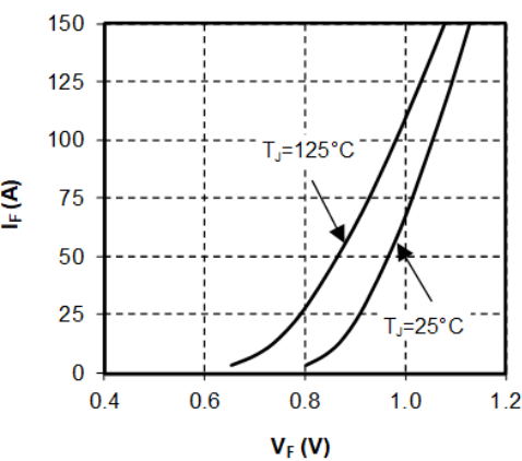
Figure 22 • Forward Characteristics
