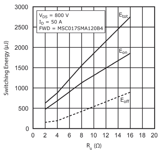
Figure 1-13. Switching Energy vs. R_g
