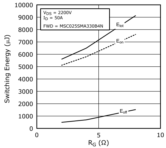
Figure 1-14. Switching Energy vs. R_G
