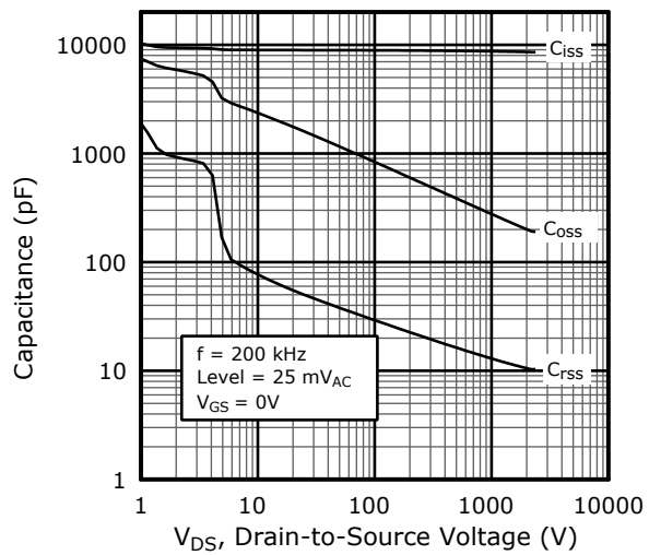
Figure 1-7. Capacitance vs. Drain-to-Source Voltage
