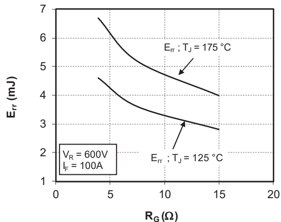
Figure 1-13. Switching Losses vs. Gate Resistance
