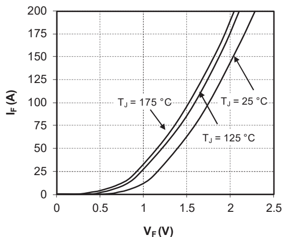
Figure 1-12. Forward Characteristics
