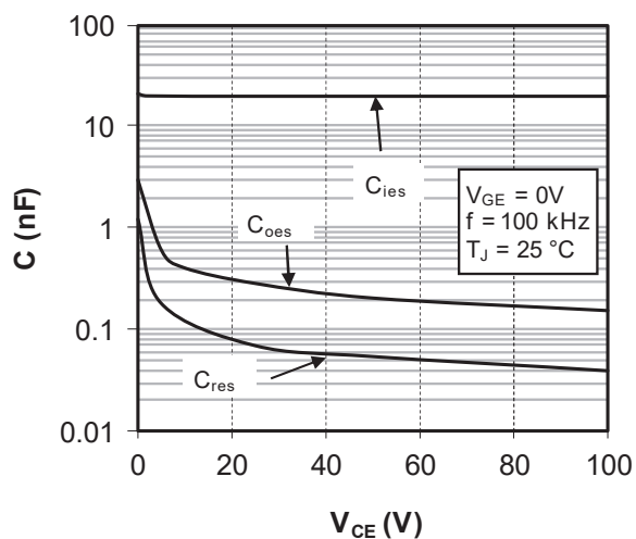
Figure 1-9. Capacity Characteristics
