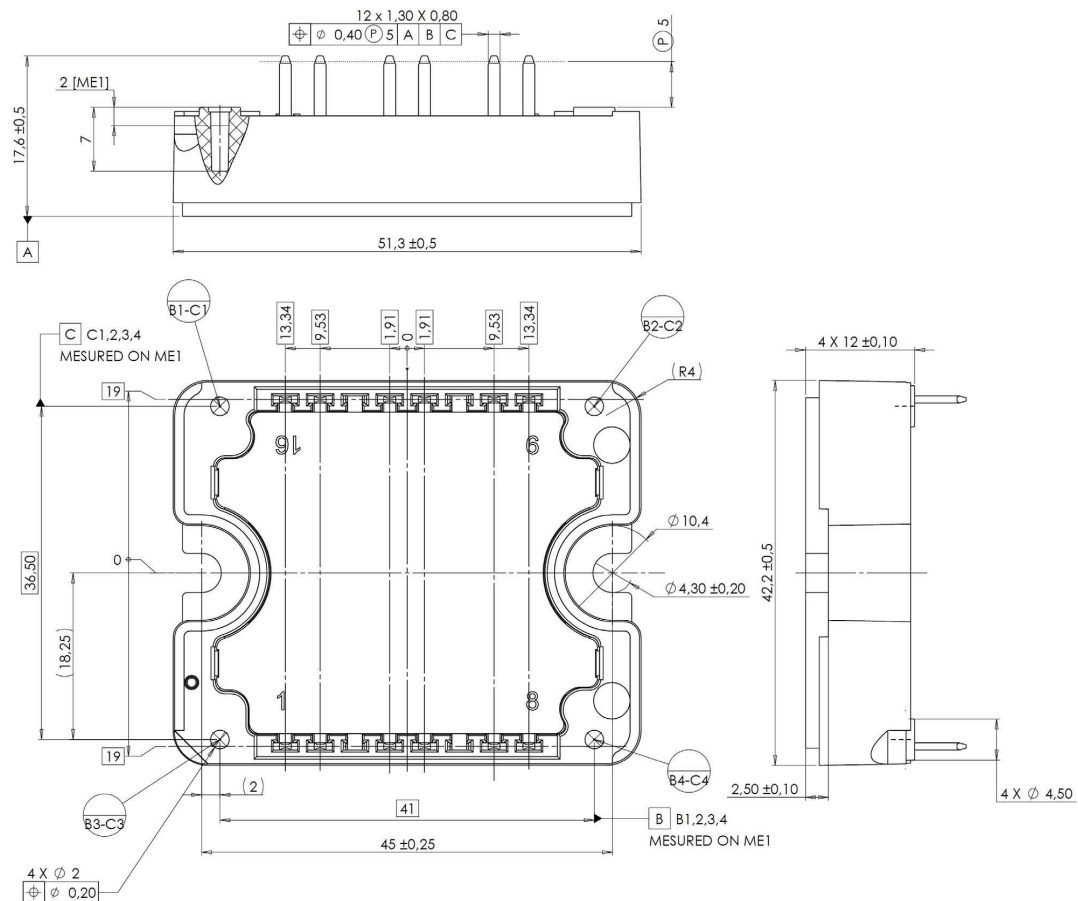
Figure 2-1. Package Outline Drawing
