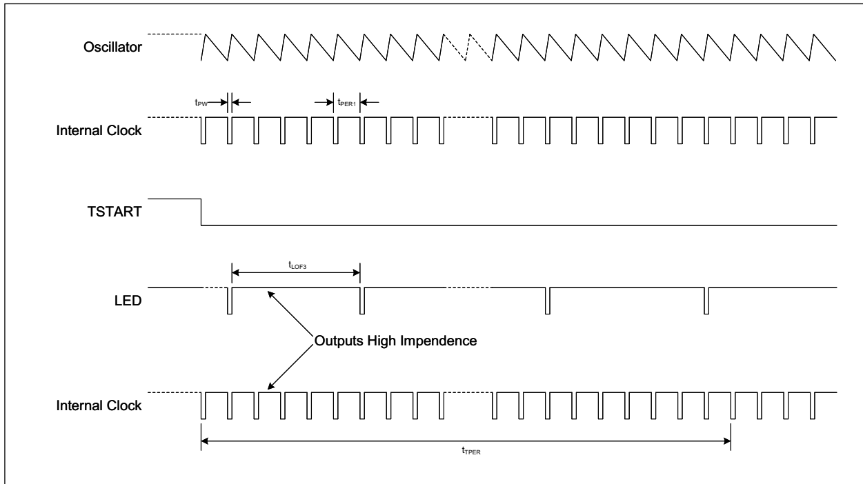
FIGURE 3-2: RE46C127 Timing Diagram – Timer Mode.
