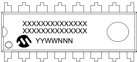
16-Lead PDIP (300 mil.)
