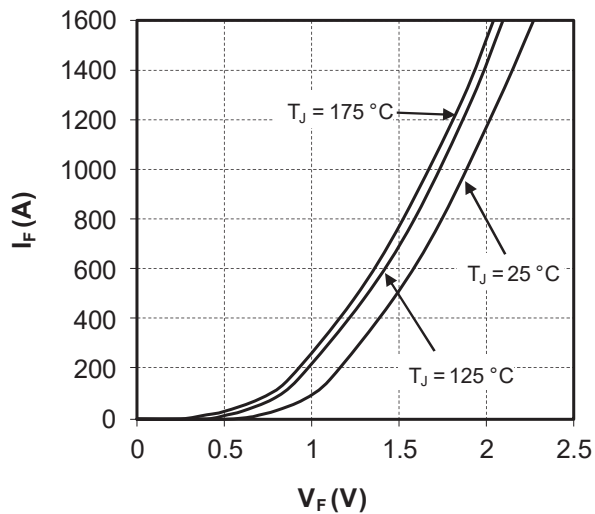
Figure 1-12. Forward Characteristics
