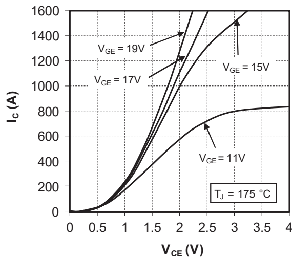
Figure 1-3. Output Characteristics, T_J = 175\text{ °C}
