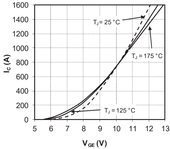
Figure 1-8. Transfer Characteristics
