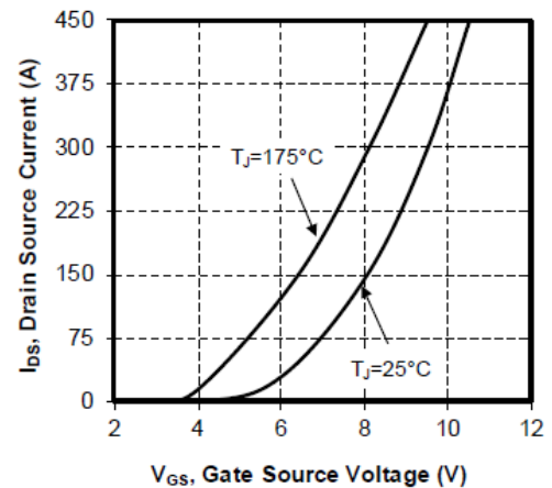
Figure 7 • Transfer Characteristics
