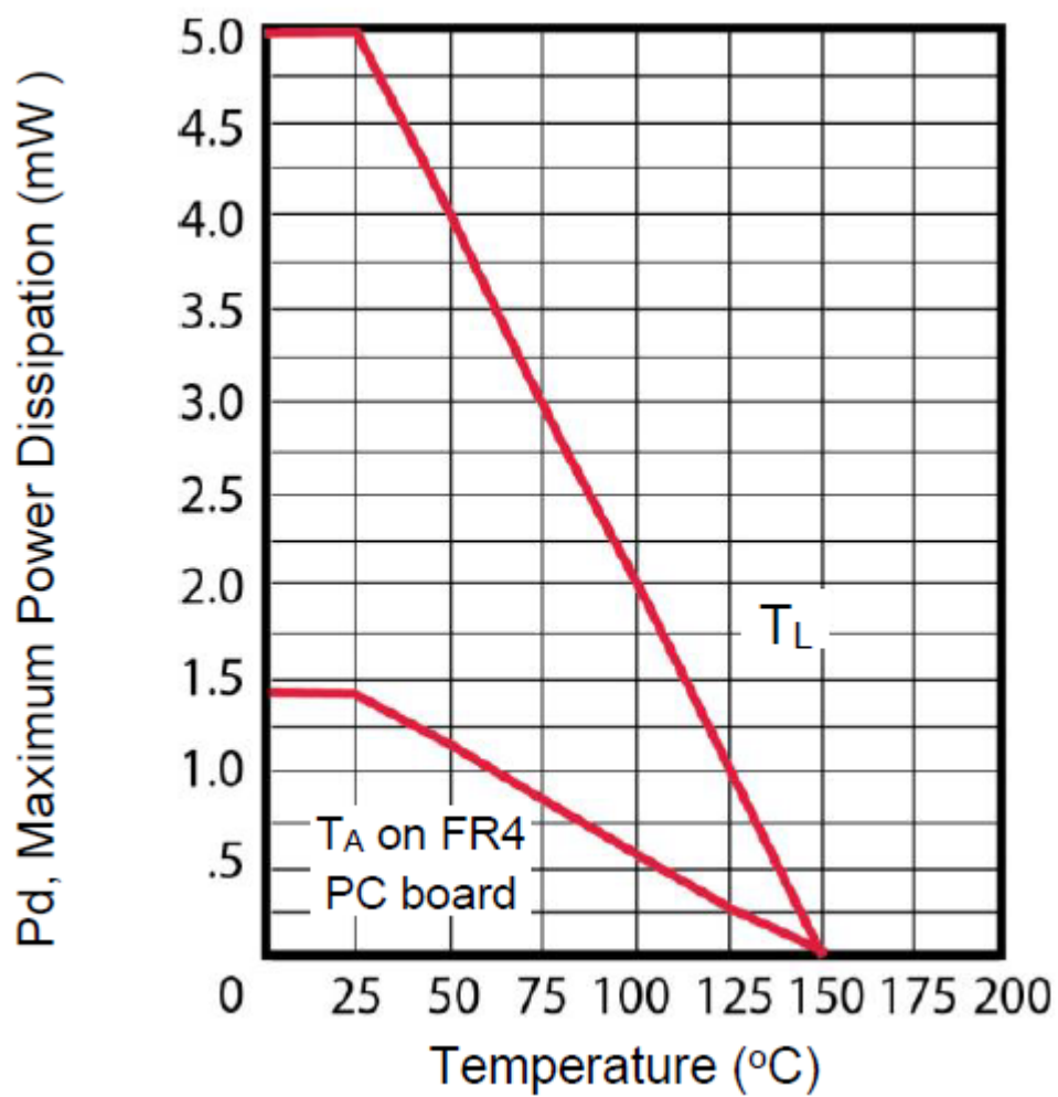
Figure 4-1. Power Derating Curve
