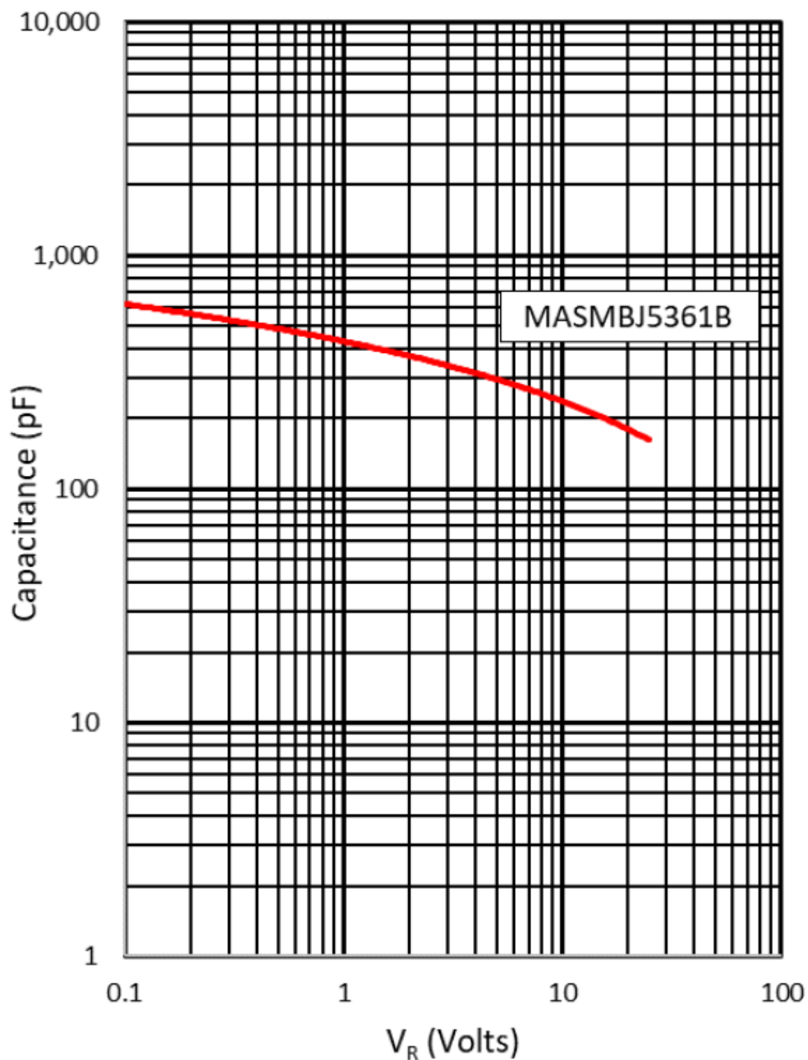
Figure 4-2. Typical Capacitance Vs. Reverse Voltage for 5 Watt Zener
