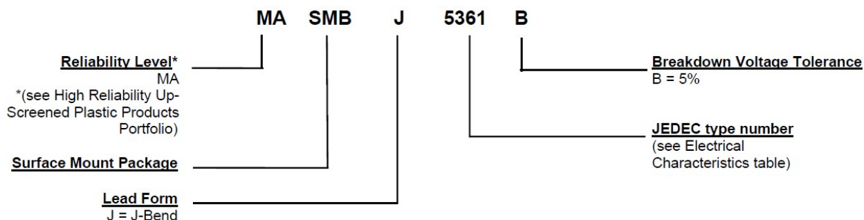
Figure 2-1. Part Nomenclature
