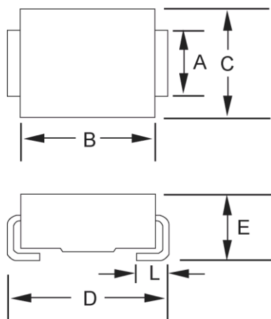
Figure 5-1. Package Dimensions
