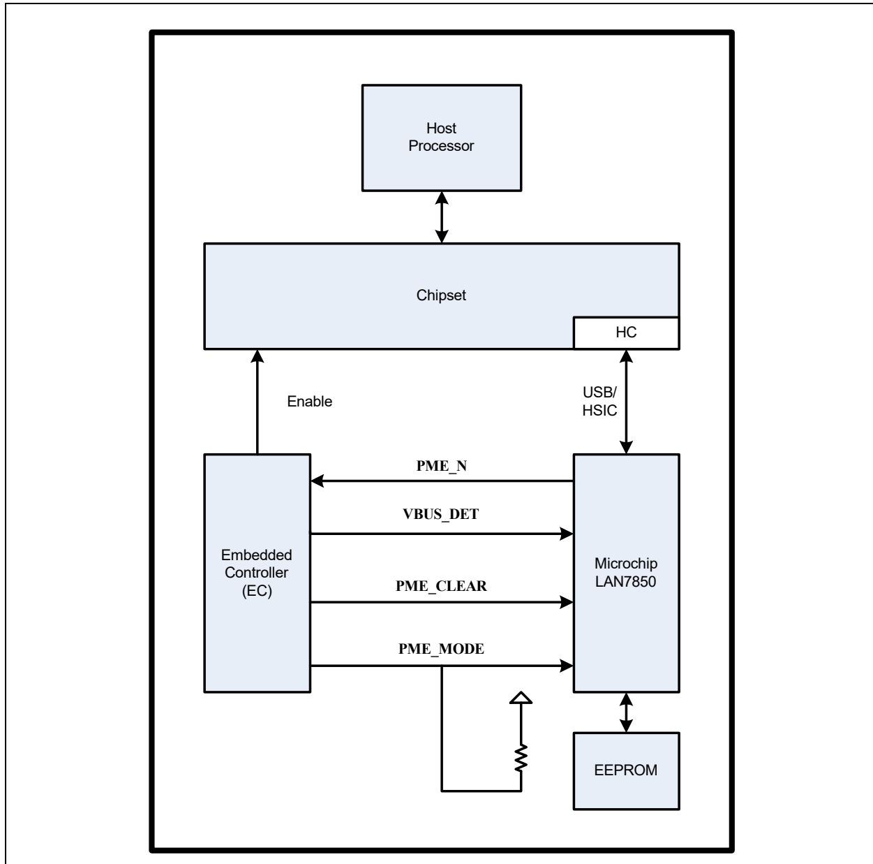
FIGURE 14-1: TYPICAL APPLICATION
