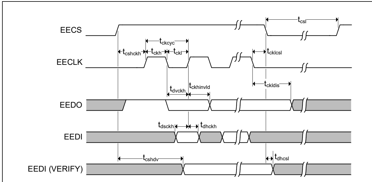
FIGURE 16-4: EEPROM TIMING
