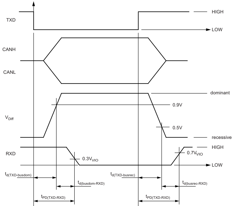
Figure 6-1. CAN Transceiver Timing Diagram 1
